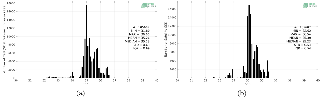
Figure 2: Histograms of SSS from TSG (GOSUD-Research-vessel) (a) and Aquarius SSS L4 OI v5 - Monthly (IPRC) (b) considering all match-up pairs per bins of 0.1 over the South Pacific Ocean Pi-MEP region and for the full satellite product period.
