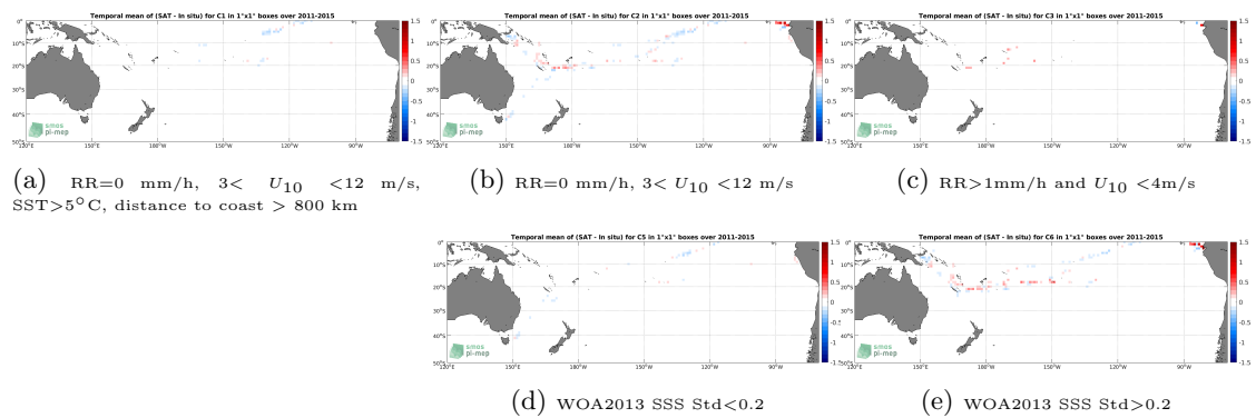
Figure 12: Temporal mean gridded over spatial boxes of size 1^\circ \times 1^\circ of \Delta\text{SSS} (Aquarius SSS L4 OI v5 - Monthly (IPRC) - TSG (GOSUD-Research-vessel)) for 5 different subdatasets corresponding to:RR=0 mm/h, 3 < U_{10} < 12 m/s, SST>5°C, distance to coast > 800 km (a), RR=0 mm/h, 3 < U_{10} < 12 m/s (b), RR>1mm/h and U_{10} < 4 m/s (c), WOA2013 SSS Std<0.2 (d), WOA2013 SSS Std>0.2 (e).
