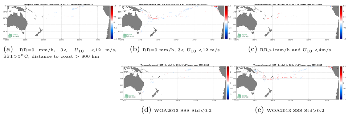
Figure 12: Temporal mean gridded over spatial boxes of size 1°x1° of \Delta SSS (Aquarius SSS L4 OI v5 - Monthly (IPRC) - TSG (GOSUD-Research-vessel)) for 5 different subdatasets corresponding to:RR=0 mm/h, 3 < U_{10} < 12 m/s, SST>5°C, distance to coast > 800 km (a), RR=0 mm/h, 3 < U_{10} < 12 m/s (b), RR>1mm/h and U_{10} < 4 m/s (c), WOA2013 SSS Std<0.2 (d), WOA2013 SSS Std>0.2 (e).
