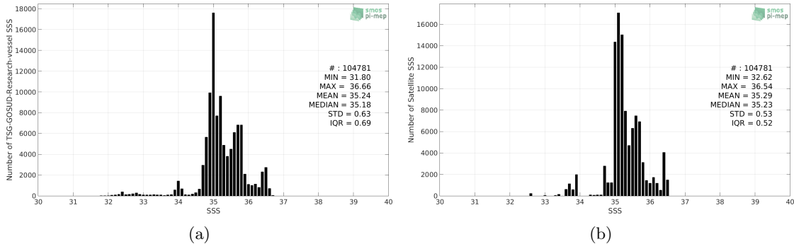
Figure 2: Histograms of SSS from TSG-GOSUD-Research-vessel (a) and Aquarius-L4-IPRC-V5-MONTHLY (b) considering all match-up pairs per bins of 0.1 over the South Pacific Ocean Pi-MEP region and for the full satellite product period.
