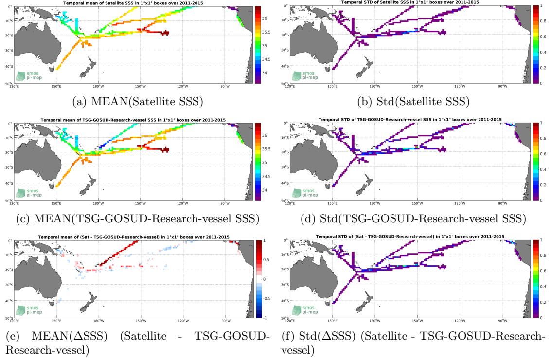
Figure 6: Temporal mean (left) and Std (right) of SSS from Aquarius-L4-IPRC-V5-MONTHLY (top), TSG-GOSUD-Research-vessel (middle), and of \Delta SSS (Satellite - TSG-GOSUD-Research-vessel). Only match-up pairs are used to generate these maps.
