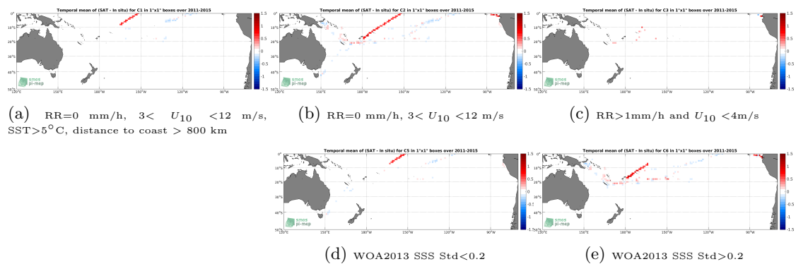
Figure 12: Temporal mean gridded over spatial boxes of size 1^\circ \times 1^\circ of \Delta SSS (Aquarius-L4-IPRC-V5-MONTHLY - TSG-GOSUD-Research-vessel) for 5 different subdatasets corresponding to:RR=0 mm/h, 3 < U_{10} < 12 m/s, SST >5^\circ\text{C} , distance to coast > 800 km (a), RR=0 mm/h, 3 < U_{10} < 12 m/s (b), RR >1 mm/h and U_{10} < 4 m/s (c), WOA2013 SSS Std <0.2 (d), WOA2013 SSS Std >0.2 (e).
