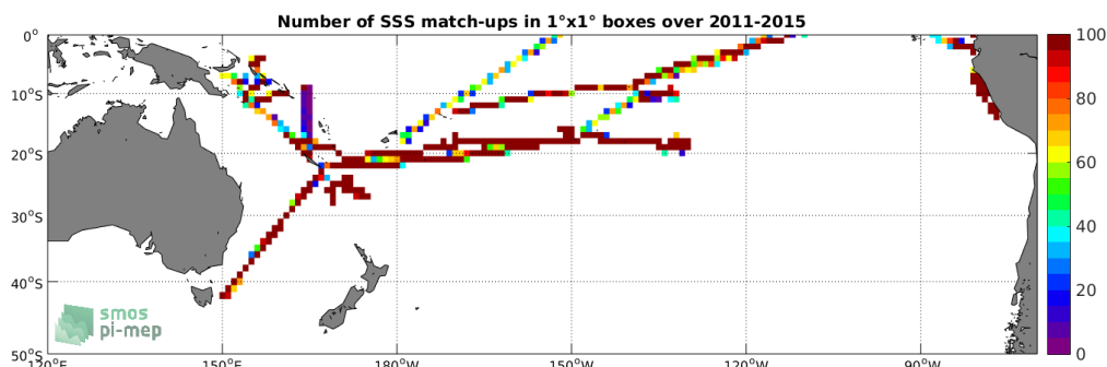
Figure 4: Number of SSS match-ups between TSG-GOSUD-Research-vessel SSS and the Aquarius-L4-IPRC-V5-MONTHLY SSS product for the South Pacific Ocean Pi-MEP region over 1°x1° boxes and for the full satellite product period.
