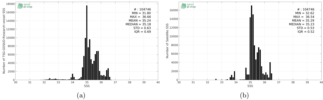
Figure 2: Histograms of SSS from TSG-GOSUD-Research-vessel (a) and Aquarius-L4-IPRC-V5-MONTHLY (b) considering all match-up pairs per bins of 0.1 over the South Pacific Ocean Pi-MEP region and for the full satellite product period.
