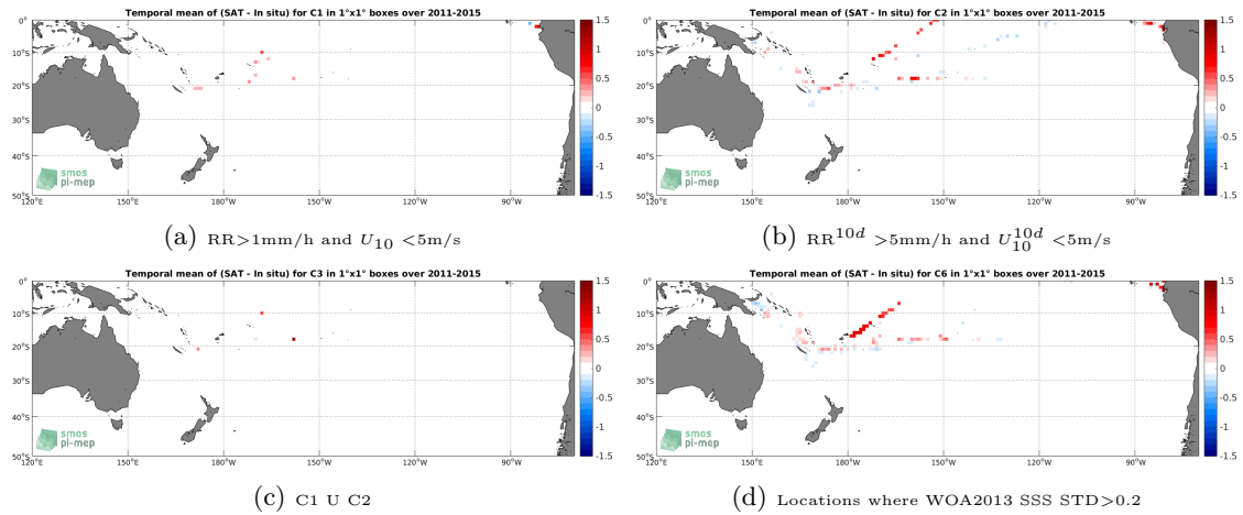
Figure 12: Temporal mean gridded over spatial boxes of size 1^\circ \times 1^\circ of \Delta SSS (Aquarius-L4-IPRC-V5-MONTHLY - TSG-GOSUD-Research-vessel) for 4 different subdatasets corresponding to: RR > 1\text{mm/h} and U_{10} < 5\text{m/s} (a), RR^{10d} > 5\text{mm/h} and U_{10}^{10d} < 5\text{m/s} (b), C1 U C2 (c), Locations where WOA2013 SSS STD > 0.2 (d).
