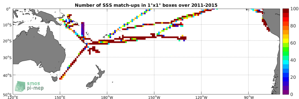
Figure 4: Number of SSS match-ups between TSG-GOSUD-Research-vessel SSS and the Aquarius-L4-IPRC-V5-MONTHLY SSS product for the South Pacific Ocean Pi-MEP region over 1^\circ \times 1^\circ boxes and for the full satellite product period.
