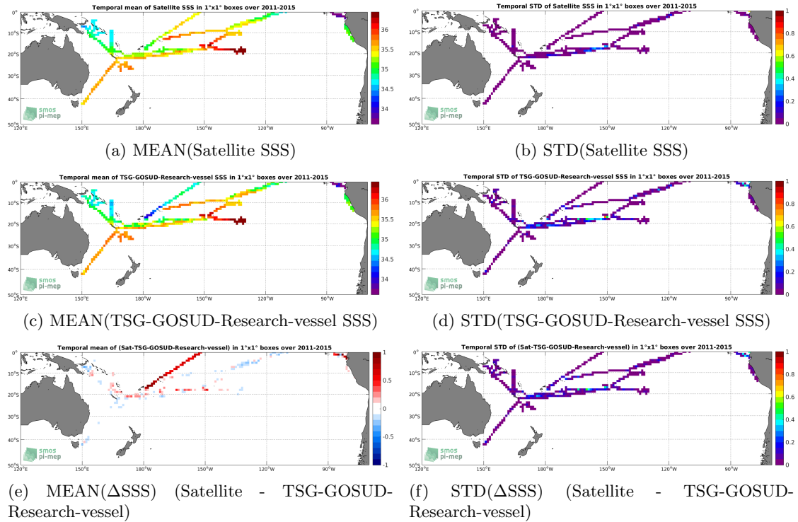
Figure 6: Temporal mean (left) and STD (right) of SSS from Aquarius-L4-IPRC-V5-MONTHLY (top), TSG-GOSUD-Research-vessel (middle), and of \Delta SSS (Satellite - TSG-GOSUD-Research-vessel). Only match-up pairs are used to generate these maps.
