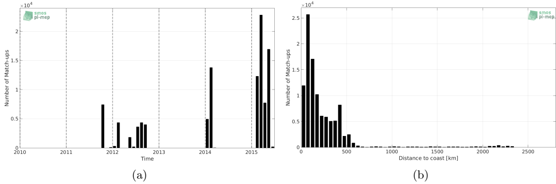
Figure 1: Number of match-ups between TSG-GOSUD-Research-vessel and Aquarius-L4-IPRC-V5-MONTHLY SSS as a function of time (a) and as function of the distance to coast (b) over the South Pacific Ocean Pi-MEP region and for the full satellite product period.
