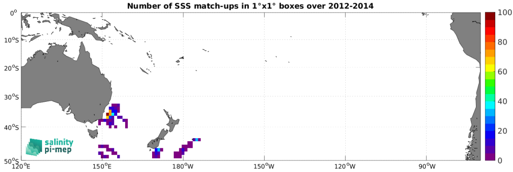
Figure 5: Number of SSS match-ups between Marine mammals SSS and the Aquarius SSS L4 OI v5 - Monthly (IPRC) SSS product for the South Pacific Ocean Pi-MEP region over 1^\circ \times 1^\circ boxes and for the full satellite product period.
