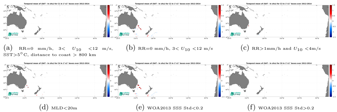
Figure 14: Temporal mean gridded over spatial boxes of size 1^\circ \times 1^\circ of \Delta SSS (Aquarius SSS L4 OI v5 - Monthly (IPRC) - Marine mammals) for 6 different subdatasets corresponding to:RR=0 mm/h, 3 < U_{10} < 12 m/s, SST >5^\circ C, distance to coast > 800 km (a), RR=0 mm/h, 3 < U_{10} < 12 m/s (b), RR >1 mm/h and U_{10} < 4 m/s (c),MLD <20 m (d),WOA2013 SSS Std <0.2 (e),WOA2013 SSS Std >0.2 (f).
