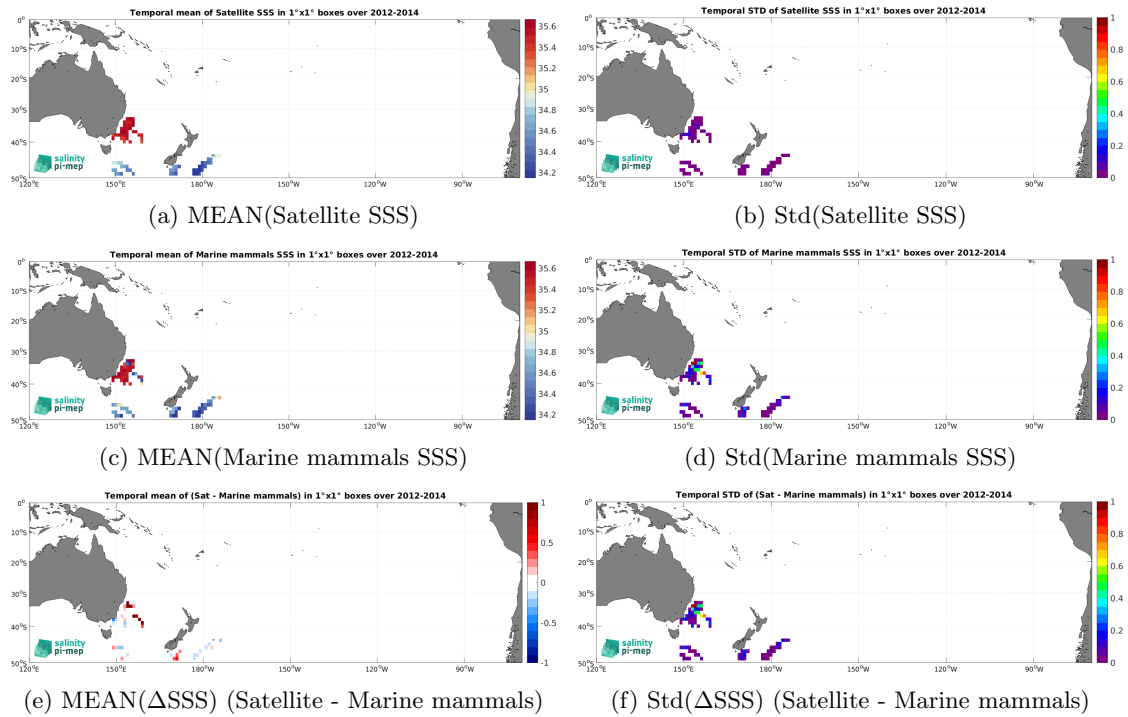
Figure 7: Temporal mean (left) and Std (right) of SSS from Aquarius SSS L4 OI v5 - Monthly (IPRC) (top), Marine mammals (middle), and of \Delta SSS (Satellite - Marine mammals). Only match-up pairs are used to generate these maps.
