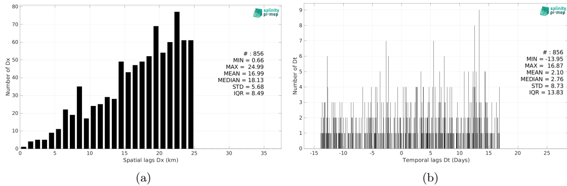
Figure 6: Histograms of the spatial (a) and temporal (b) lags between the location/time of the Marine mammals measurement and the date of the corresponding Aquarius SSS L4 OI v5 - Monthly (IPRC) SSS pixel.
