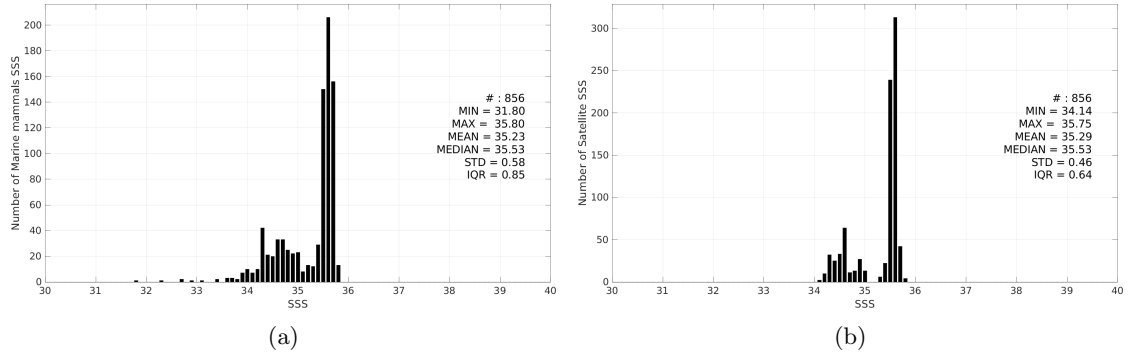
Figure 3: Histograms of SSS from Marine mammals (a) and Aquarius SSS L4 OI v5 - Monthly (IPRC) (b) considering all match-up pairs per bins of 0.1 over the South Pacific Ocean Pi-MEP region and for the full satellite product period.
