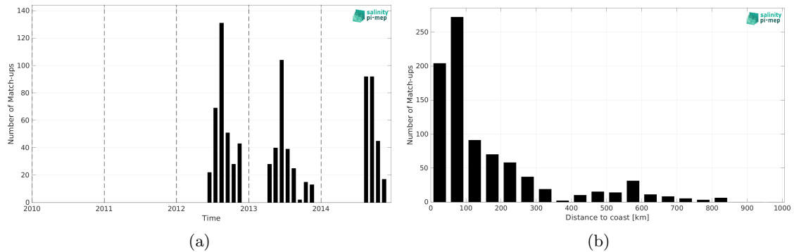
Figure 2: Number of match-ups between Marine mammals and Aquarius SSS L4 OI v5 - Monthly (IPRC) SSS as a function of time (a) and as function of the distance to coast (b) over the South Pacific Ocean Pi-MEP region and for the full satellite product period.
