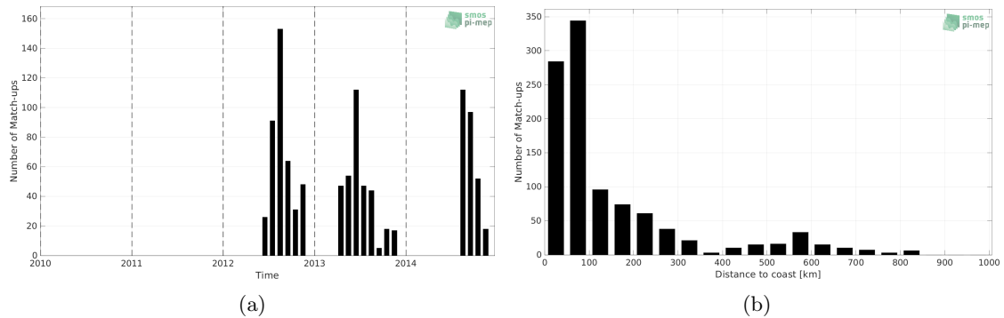
Figure 1: Number of match-ups between Marine mammals and Aquarius SSS L4 OI v5 - Monthly (IPRC) SSS as a function of time (a) and as function of the distance to coast (b) over the South Pacific Ocean Pi-MEP region and for the full satellite product period.
