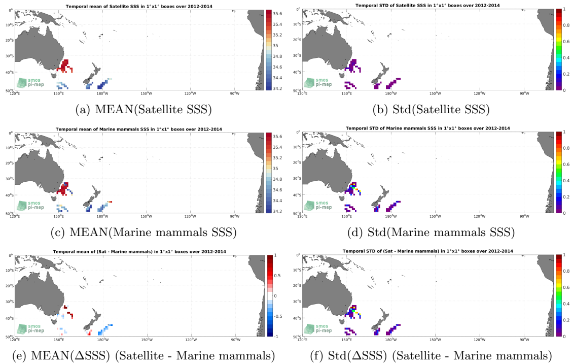
Figure 6: Temporal mean (left) and Std (right) of SSS from Aquarius SSS L4 OI v5 - Monthly (IPRC) (top), Marine mammals (middle), and of \Delta SSS (Satellite - Marine mammals). Only match-up pairs are used to generate these maps.
