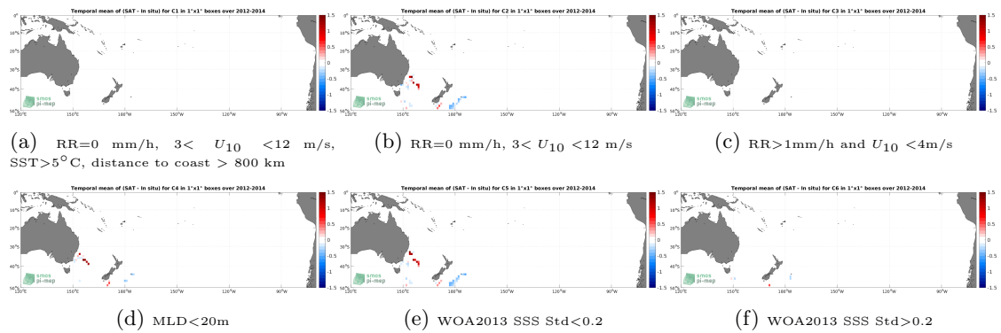
Figure 12: Temporal mean gridded over spatial boxes of size 1^\circ \times 1^\circ of \Delta SSS (Aquarius SSS L4 OI v5 - Monthly (IPRC) - Marine mammals) for 6 different subdatasets corresponding to:RR=0 mm/h, 3 < U_{10} < 12 m/s, SST >5^\circ C, distance to coast > 800 km (a), RR=0 mm/h, 3 < U_{10} < 12 m/s (b), RR >1 mm/h and U_{10} < 4 m/s (c),MLD <20 m (d),WOA2013 SSS Std <0.2 (e),WOA2013 SSS Std >0.2 (f).
