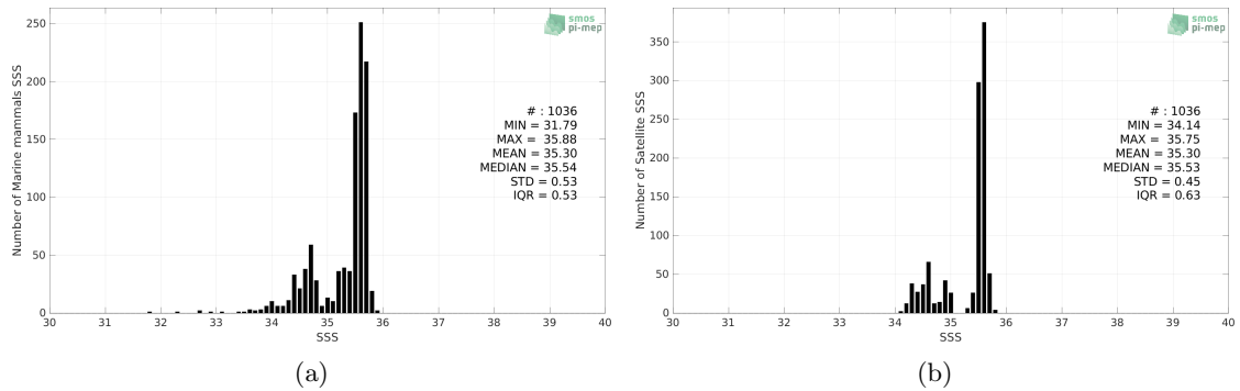
Figure 2: Histograms of SSS from Marine mammals (a) and Aquarius SSS L4 OI v5 - Monthly (IPRC) (b) considering all match-up pairs per bins of 0.1 over the South Pacific Ocean Pi-MEP region and for the full satellite product period.
