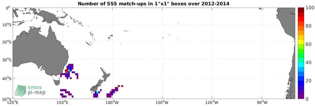
Figure 4: Number of SSS match-ups between Marine mammals SSS and the Aquarius SSS L4 OI v5 - Monthly (IPRC) SSS product for the South Pacific Ocean Pi-MEP region over 1^\circ \times 1^\circ boxes and for the full satellite product period.
