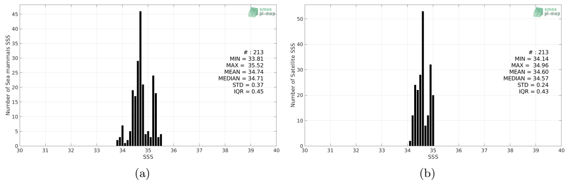
Figure 2: Histograms of SSS from Sea mammals (a) and Aquarius SSS L4 OI v5 - Monthly (IPRC) (b) considering all match-up pairs per bins of 0.1 over the South Pacific Ocean Pi-MEP region and for the full satellite product period.
