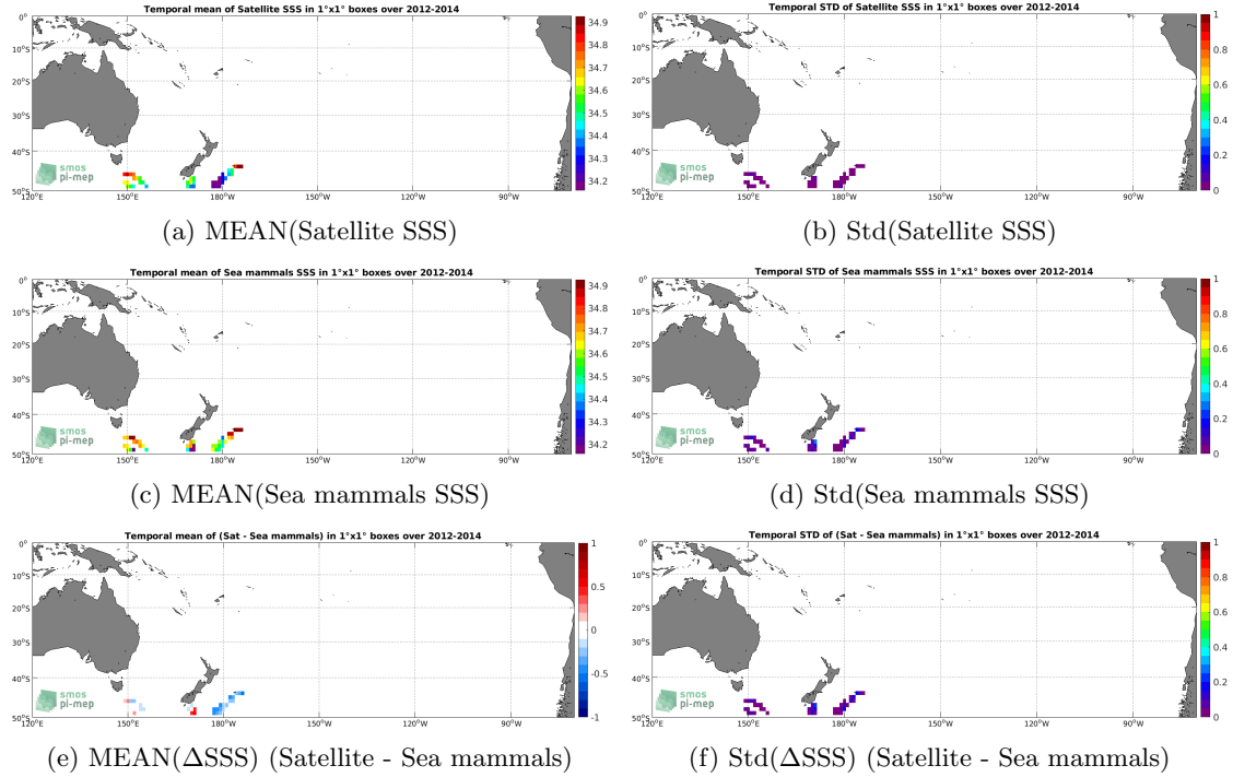
Figure 6: Temporal mean (left) and Std (right) of SSS from Aquarius SSS L4 OI v5 - Monthly (IPRC) (top), Sea mammals (middle), and of \Delta SSS (Satellite - Sea mammals). Only match-up pairs are used to generate these maps.
