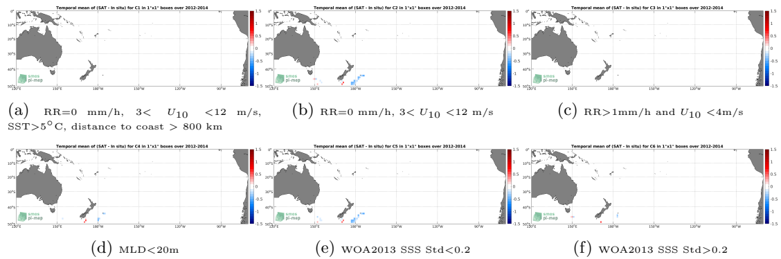
Figure 12: Temporal mean gridded over spatial boxes of size 1^{\circ}\times 1^{\circ} of \Delta\text{SSS} (Aquarius SSS L4 OI v5 - Monthly (IPRC) - Sea mammals) for 6 different subdatasets corresponding to: \text{RR}=0 mm/h, 3 < U_{10} < 12 m/s, \text{SST} > 5^{\circ}\text{C} , distance to coast > 800 km (a), \text{RR}=0 mm/h, 3 < U_{10} < 12 m/s (b), \text{RR} > 1\text{mm/h} and U_{10} < 4\text{m/s} (c), \text{MLD} < 20\text{m} (d), \text{WOA2013 SSS Std} < 0.2 (e), \text{WOA2013 SSS Std} > 0.2 (f).
