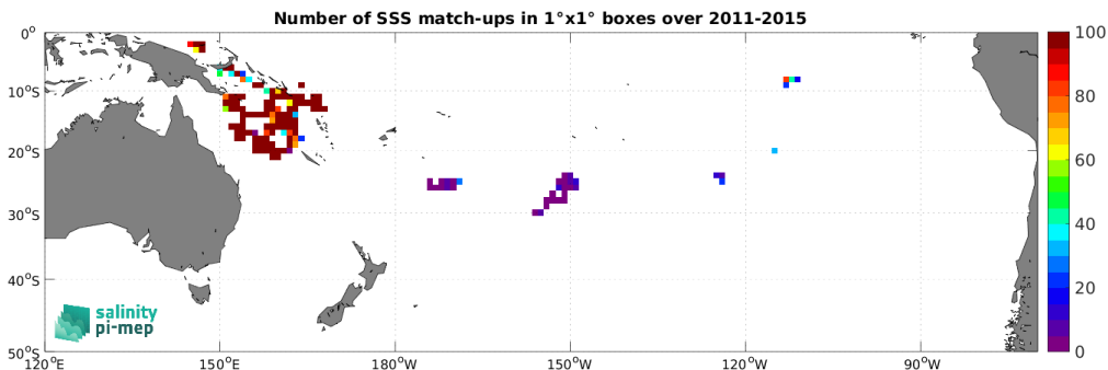
Figure 4: Number of SSS match-ups between Surface drifters SSS and the Aquarius SSS L4 OI v5 - Monthly (IPRC) SSS product for the South Pacific Ocean Pi-MEP region over 1^\circ \times 1^\circ boxes and for the full satellite product period.
