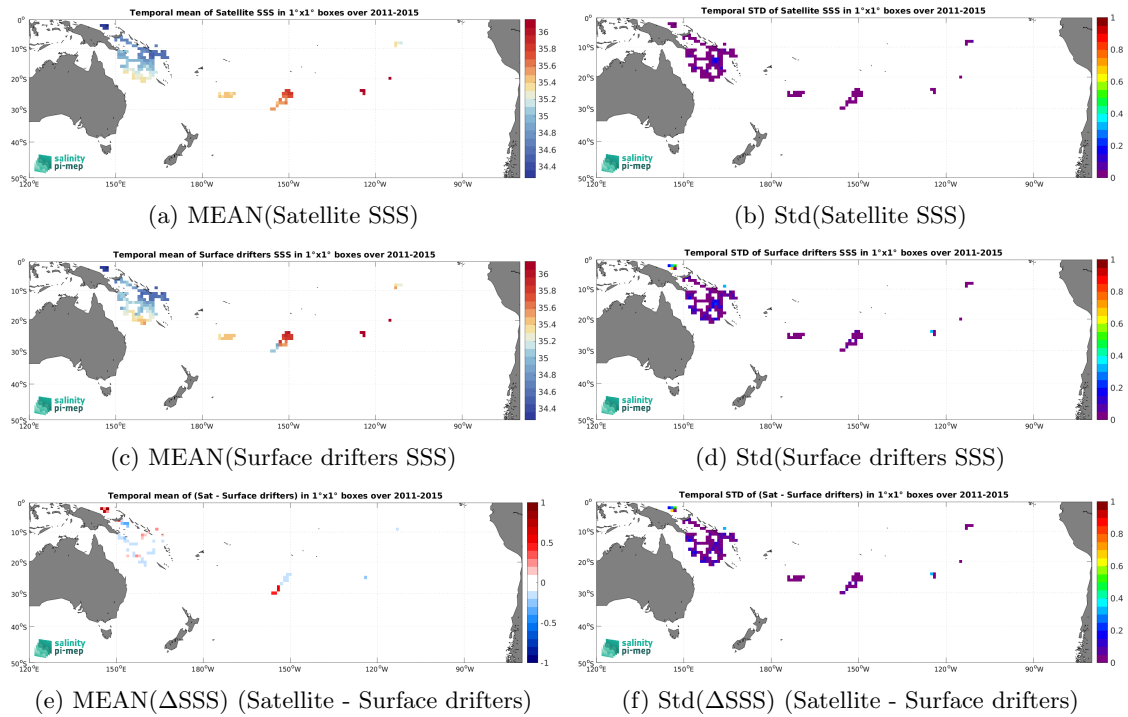
Figure 6: Temporal mean (left) and Std (right) of SSS from Aquarius SSS L4 OI v5 - Monthly (IPRC) (top), Surface drifters (middle), and of \Delta SSS (Satellite - Surface drifters). Only match-up pairs are used to generate these maps.
