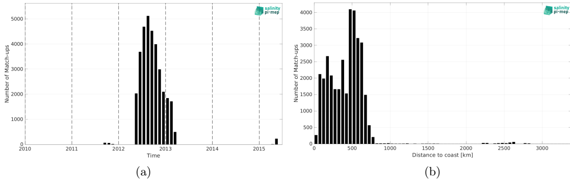
Figure 2: Number of match-ups between Surface drifters and Aquarius SSS L4 OI v5 - Monthly (IPRC) SSS as a function of time (a) and as function of the distance to coast (b) over the South Pacific Ocean Pi-MEP region and for the full satellite product period.
