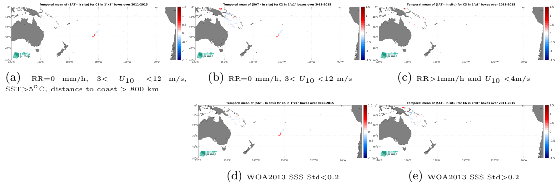
Figure 13: Temporal mean gridded over spatial boxes of size 1^\circ \times 1^\circ of \Delta SSS (Aquarius SSS L4 OI v5 - Monthly (IPRC) - Surface drifters) for 5 different subdatasets corresponding to:RR=0 mm/h, 3 < U_{10} < 12 m/s, SST >5^\circ\text{C} , distance to coast > 800 km (a), RR=0 mm/h, 3 < U_{10} < 12 m/s (b), RR >1 mm/h and U_{10} < 4 m/s (c), WOA2013 SSS Std <0.2 (d), WOA2013 SSS Std >0.2 (e).
