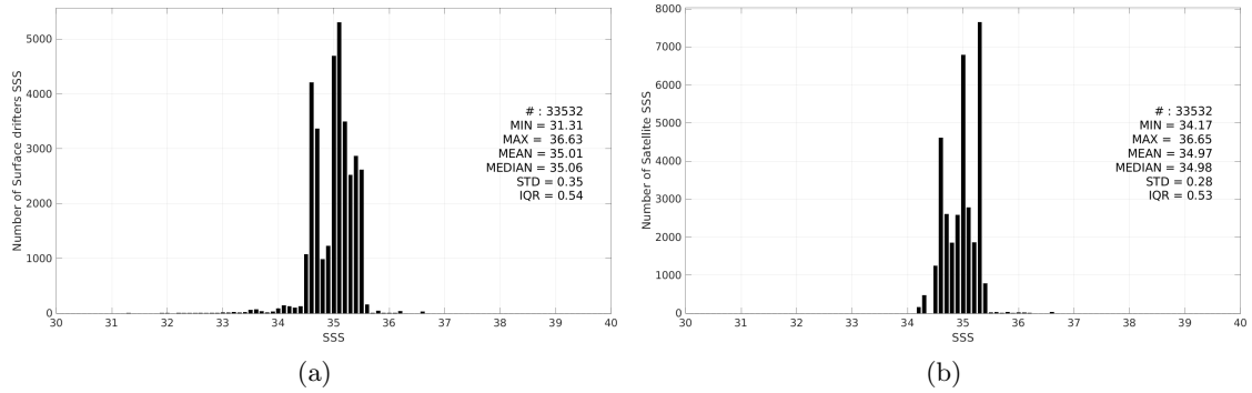
Figure 3: Histograms of SSS from Surface drifters (a) and Aquarius SSS L4 OI v5 - Monthly (IPRC) (b) considering all match-up pairs per bins of 0.1 over the South Pacific Ocean Pi-MEP region and for the full satellite product period.
