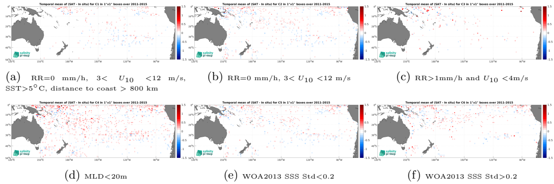
Figure 14: Temporal mean gridded over spatial boxes of size 1^\circ \times 1^\circ of \Delta SSS (Aquarius SSS L4 OI v5 - Monthly (IPRC) - Argo) for 6 different subdatasets corresponding to:RR=0 mm/h, 3 < U_{10} < 12 m/s, SST >5^\circ C, distance to coast > 800 km (a), RR=0 mm/h, 3 < U_{10} < 12 m/s (b), RR >1 mm/h and U_{10} < 4 m/s (c),MLD <20 m (d),WOA2013 SSS Std <0.2 (e),WOA2013 SSS Std >0.2 (f).
