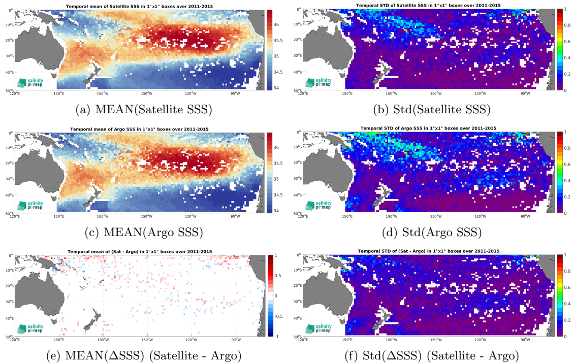
Figure 7: Temporal mean (left) and Std (right) of SSS from Aquarius SSS L4 OI v5 - Monthly (IPRC) (top), Argo (middle), and of \Delta SSS (Satellite - Argo). Only match-up pairs are used to generate these maps.
