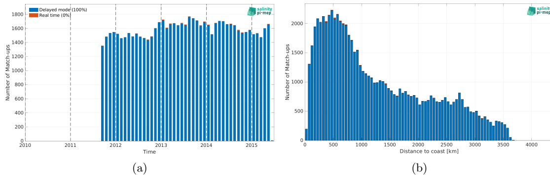
Figure 2: Number of match-ups between Argo and Aquarius SSS L4 OI v5 - Monthly (IPRC) SSS as a function of time (a) and as function of the distance to coast (b) over the South Pacific Ocean Pi-MEP region and for the full satellite product period.
