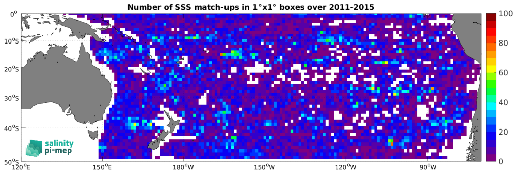
Figure 5: Number of SSS match-ups between Argo SSS and the Aquarius SSS L4 OI v5 - Monthly (IPRC) SSS product for the South Pacific Ocean Pi-MEP region over 1^\circ \times 1^\circ boxes and for the full satellite product period.
