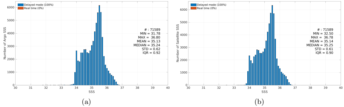
Figure 3: Histograms of SSS from Argo (a) and Aquarius SSS L4 OI v5 - Monthly (IPRC) (b) considering all match-up pairs per bins of 0.1 over the South Pacific Ocean Pi-MEP region and for the full satellite product period.
