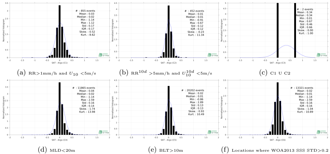
Figure 13: Normalized histogram of \Delta SSS (Aquarius-L4-IPRC-V5-MONTHLY - Argo) for 6 different subdatasets corresponding to: RR>1mm/h and U_{10} <5m/s (a), RR^{10d} >5mm/h and U_{10}^{10d} <5m/s (b), C1 U C2 (c),MLD<20m (d),BLT>10m (e),Locations where WOA2013 SSS STD>0.2 (f).
