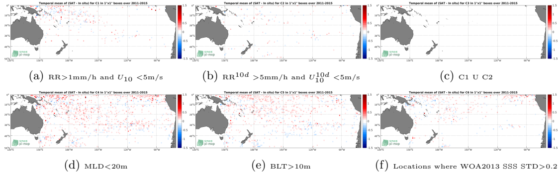
Figure 12: Temporal mean gridded over spatial boxes of size 1°x1° of \Delta SSS (Aquarius-L4-IPRC-V5-MONTHLY - Argo) for 6 different subdatasets corresponding to:RR>1mm/h and U_{10} <5m/s (a), RR^{10d} >5mm/h and U_{10}^{10d} <5m/s (b), C1 U C2 (c),MLD<20m (d),BLT>10m (e),Locations where WOA2013 SSS STD>0.2 (f).
