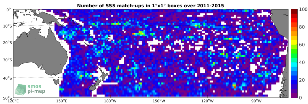
Figure 4: Number of SSS match-ups between Argo SSS and the Aquarius-L4-IPRC-V5-MONTHLY SSS product for the South Pacific Ocean Pi-MEP region over 1^\circ \times 1^\circ boxes and for the full satellite product period.
