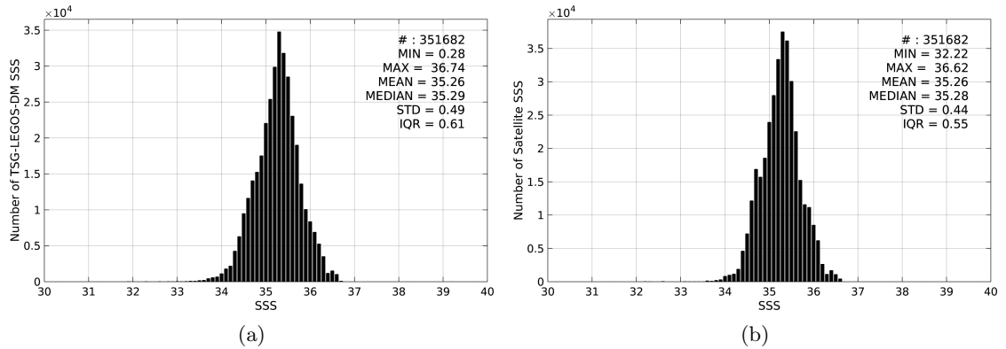
Figure 2: Histograms of SSS from TSG-LEGOS-DM (a) and Aquarius-L4-IPRC-V4-WEEKLY (b) considering all match-up pairs per bins of 0.1 over the South Pacific Ocean Pi-MEP region and for the full satellite product period.
