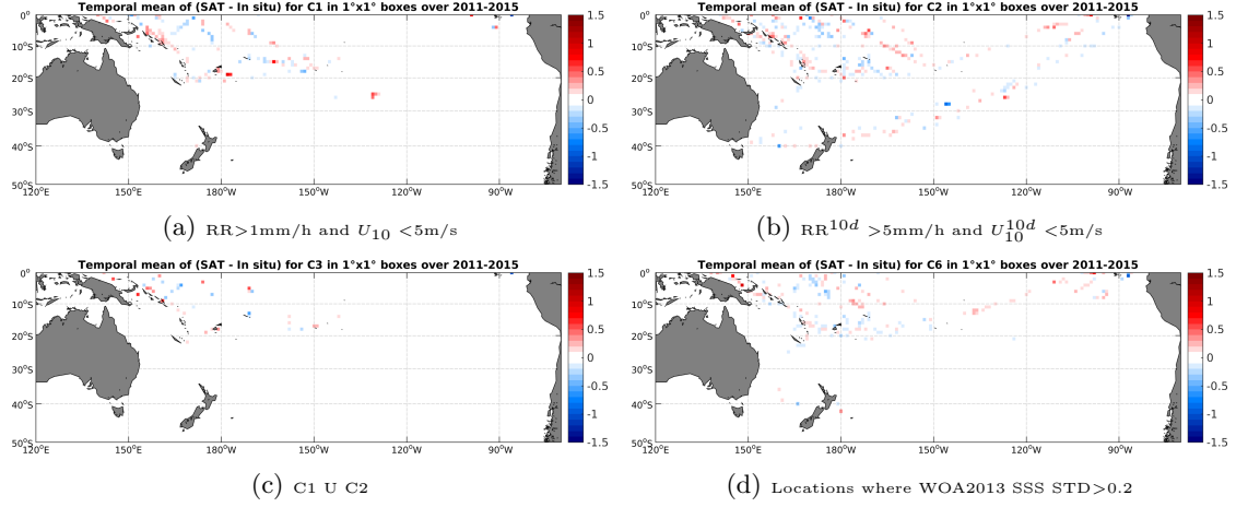
Figure 12: Temporal mean gridded over spatial boxes of size 1^\circ \times 1^\circ of \Delta SSS (Aquarius-L4-IPRC-V4-WEEKLY - TSG-LEGOS-DM) for 4 different subdatasets corresponding to: RR > 1 mm/h and U_{10} < 5 m/s (a), RR 10d > 5 mm/h and U_{10}^{10d} < 5 m/s (b), C1 U C2 (c), Locations where WOA2013 SSS STD > 0.2 (d).
