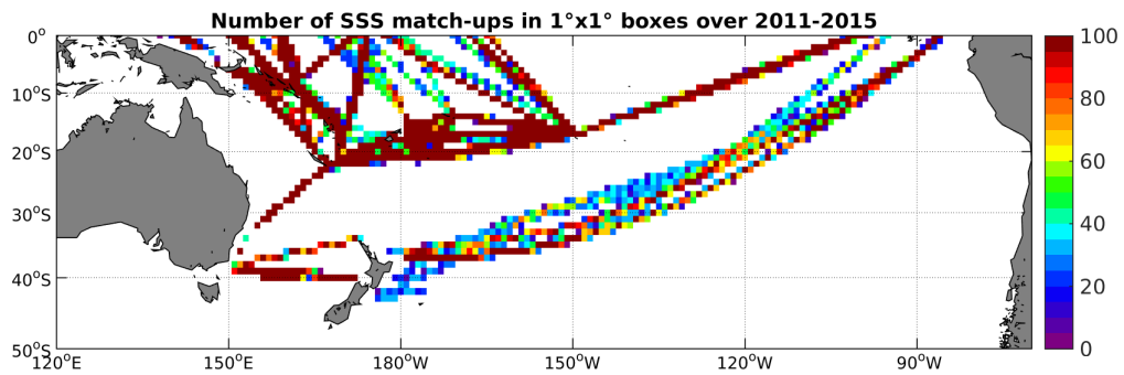
Figure 4: Number of SSS match-ups between TSG-LEGOS-DM SSS and the Aquarius-L4-IPRC-V4-WEEKLY SSS product for the South Pacific Ocean Pi-MEP region over 1^\circ \times 1^\circ boxes and for the full satellite product period.
