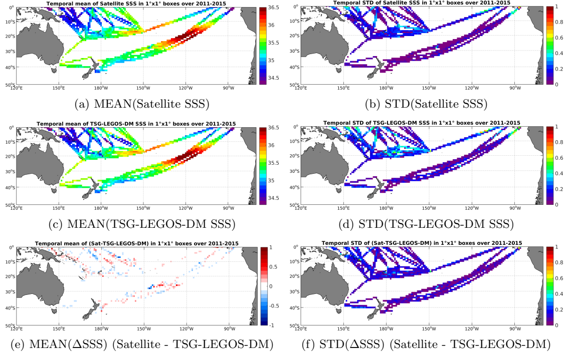
Figure 6: Temporal mean (left) and STD (right) of SSS from Aquarius-L4-IPRC-V4-WEEKLY (top), TSG-LEGOS-DM (middle), and of \Delta SSS (Satellite - TSG-LEGOS-DM). Only match-up pairs are used to generate these maps.
