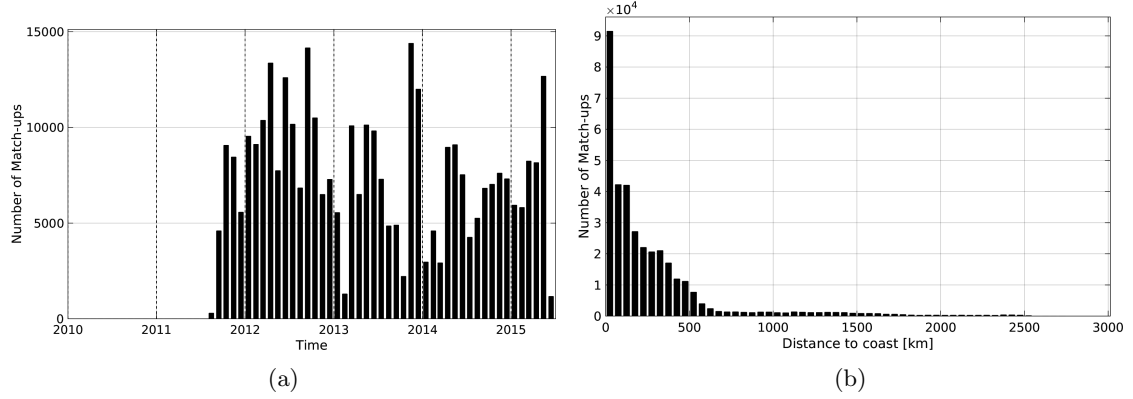
Figure 1: Number of match-ups between TSG-LEGOS-DM and Aquarius-L4-IPRC-V4-WEEKLY SSS as a function of time (a) and as function of the distance to coast (b) over the South Pacific Ocean Pi-MEP region and for the full satellite product period.
