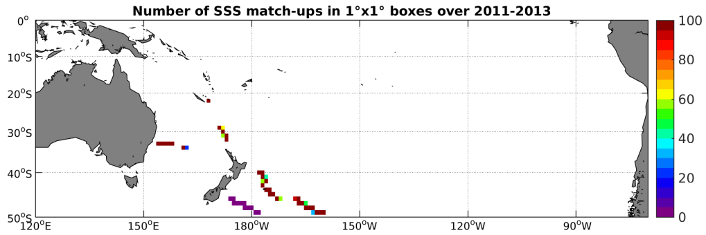
Figure 4: Number of SSS match-ups between TSG-GOSUD-Sailing-ship SSS and the Aquarius-L4-IPRC-V4-WEEKLY SSS product for the South Pacific Ocean Pi-MEP region over 1^\circ \times 1^\circ boxes and for the full satellite product period.
