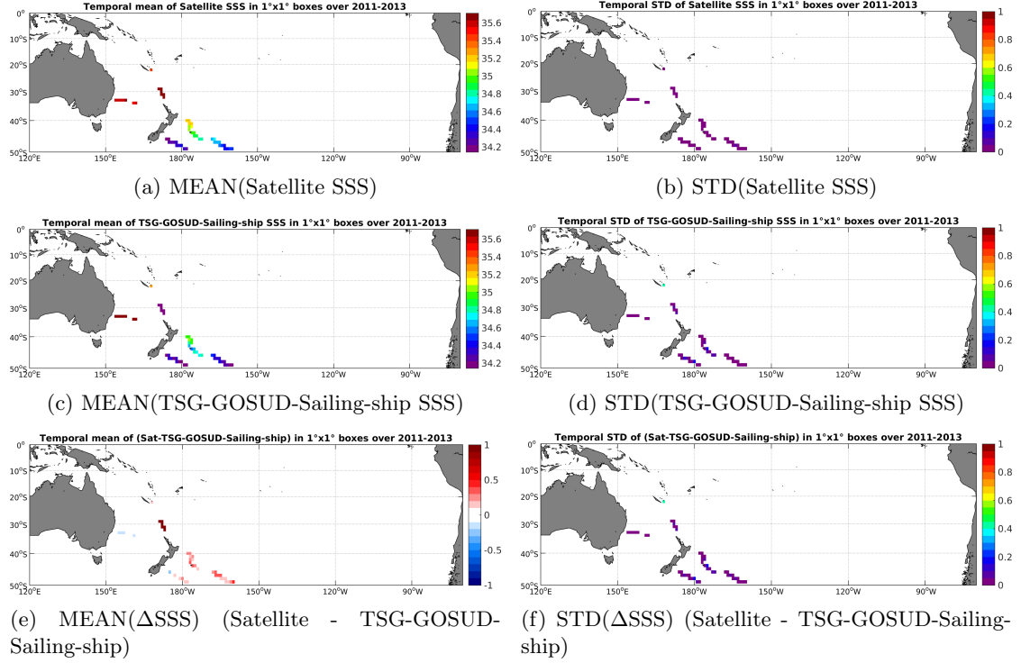
Figure 6: Temporal mean (left) and STD (right) of SSS from Aquarius-L4-IPRC-V4-WEEKLY (top), TSG-GOSUD-Sailing-ship (middle), and of \Delta SSS (Satellite - TSG-GOSUD-Sailing-ship). Only match-up pairs are used to generate these maps.
