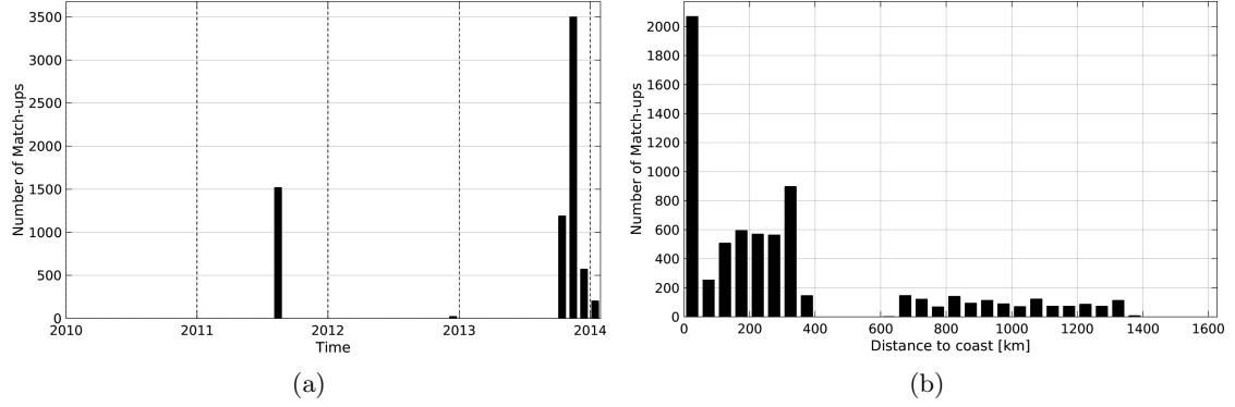
Figure 1: Number of match-ups between TSG-GOSUD-Sailing-ship and Aquarius-L4-IPRC-V4-WEEKLY SSS as a function of time (a) and as function of the distance to coast (b) over the South Pacific Ocean Pi-MEP region and for the full satellite product period.
