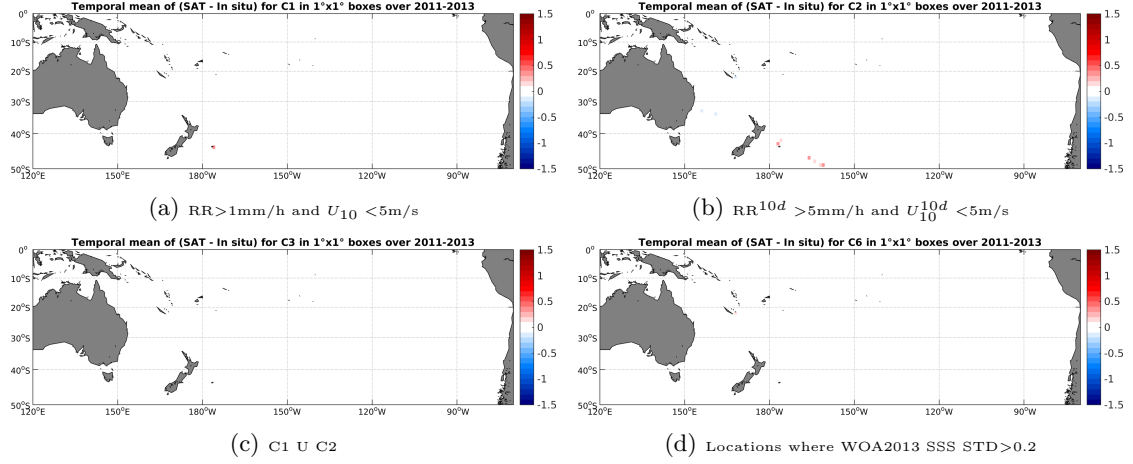
Figure 12: Temporal mean gridded over spatial boxes of size 1^\circ \times 1^\circ of \Delta SSS (Aquarius-L4-IPRC-V4-WEEKLY - TSG-GOSUD-Sailing-ship) for 4 different subdatasets corresponding to: RR > 1 mm/h and U_{10} < 5 m/s (a), RR^{10d} > 5 mm/h and U_{10}^{10d} < 5 m/s (b), C1 U C2 (c), Locations where WOA2013 SSS STD > 0.2 (d).
