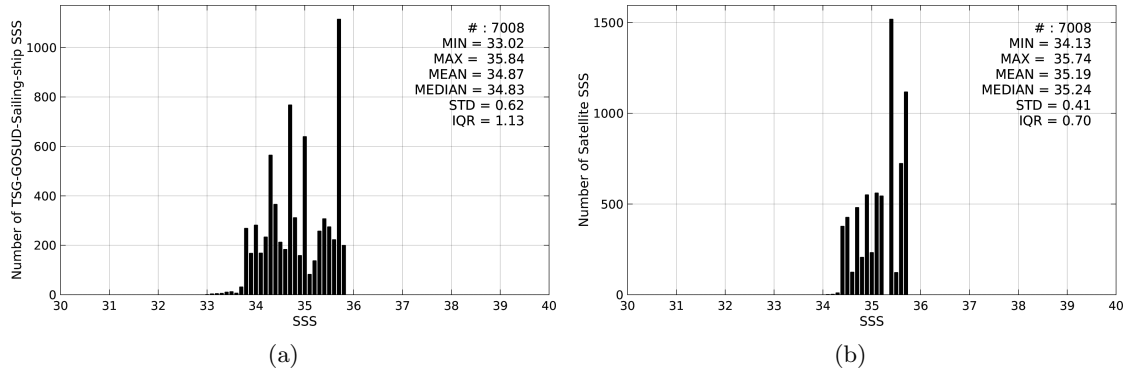
Figure 2: Histograms of SSS from TSG-GOSUD-Sailing-ship (a) and Aquarius-L4-IPRC-V4-WEEKLY (b) considering all match-up pairs per bins of 0.1 over the South Pacific Ocean Pi-MEP region and for the full satellite product period.
