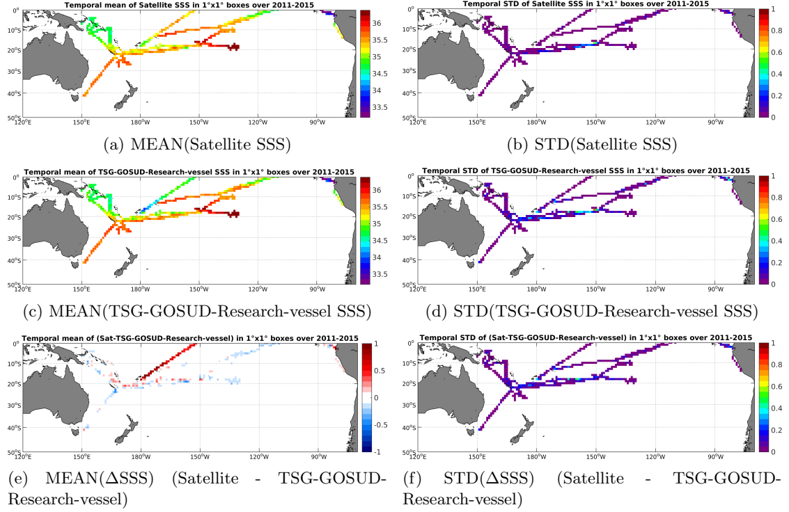
Figure 6: Temporal mean (left) and STD (right) of SSS from Aquarius-L4-IPRC-V4-WEEKLY (top), TSG-GOSUD-Research-vessel (middle), and of \Delta SSS (Satellite - TSG-GOSUD-Research-vessel). Only match-up pairs are used to generate these maps.
