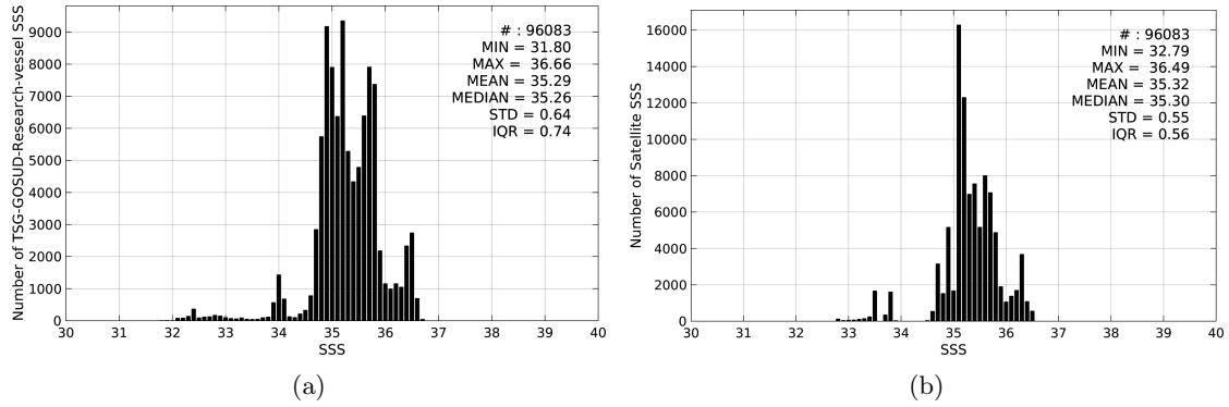
Figure 2: Histograms of SSS from TSG-GOSUD-Research-vessel (a) and Aquarius-L4-IPRC-V4-WEEKLY (b) considering all match-up pairs per bins of 0.1 over the South Pacific Ocean Pi-MEP region and for the full satellite product period.
