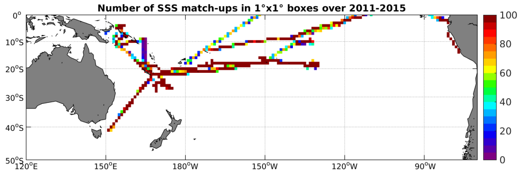
Figure 4: Number of SSS match-ups between TSG-GOSUD-Research-vessel SSS and the Aquarius-L4-IPRC-V4-WEEKLY SSS product for the South Pacific Ocean Pi-MEP region over 1^\circ \times 1^\circ boxes and for the full satellite product period.
