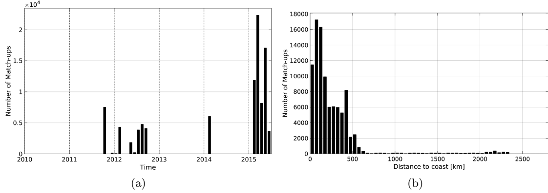
Figure 1: Number of match-ups between TSG-GOSUD-Research-vessel and Aquarius-L4-IPRC-V4-WEEKLY SSS as a function of time (a) and as function of the distance to coast (b) over the South Pacific Ocean Pi-MEP region and for the full satellite product period.
