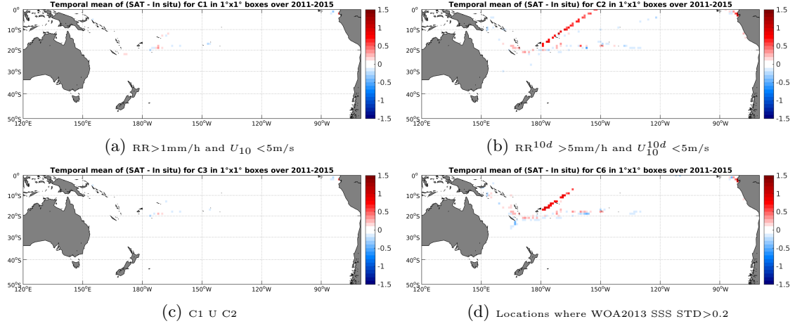
Figure 12: Temporal mean gridded over spatial boxes of size 1^\circ \times 1^\circ of \Delta SSS (Aquarius-L4-IPRC-V4-WEEKLY - TSG-GOSUD-Research-vessel) for 4 different subdatasets corresponding to: RR > 1mm/h and U_{10} < 5 m/s (a), RR^{10d} > 5 mm/h and U_{10}^{10d} < 5 m/s (b), C1 U C2 (c), Locations where WOA2013 SSS STD > 0.2 (d).
