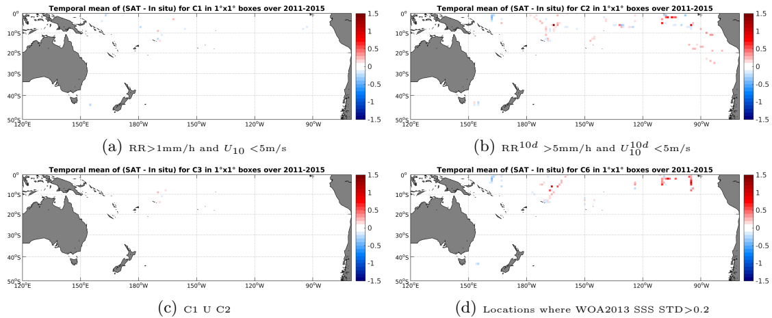
Figure 12: Temporal mean gridded over spatial boxes of size 1^\circ \times 1^\circ of \Delta SSS (Aquarius-L4-IPRC-V4-MONTHLY - TSG-SAMOS) for 4 different subdatasets corresponding to: RR > 1\text{mm/h} and U_{10} < 5\text{m/s} (a), RR^{10d} > 5\text{mm/h} and U_{10}^{10d} < 5\text{m/s} (b), C1 U C2 (c), Locations where WOA2013 SSS STD > 0.2 (d).
