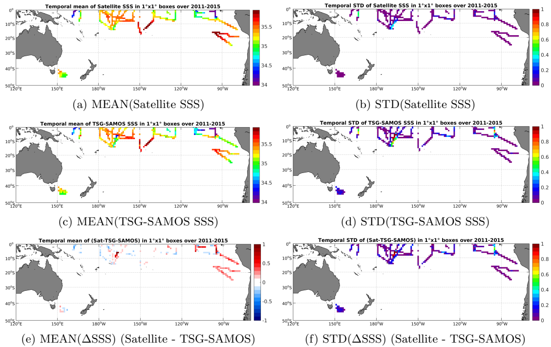
Figure 6: Temporal mean (left) and STD (right) of SSS from Aquarius-L4-IPRC-V4-MONTHLY (top), TSG-SAMOS (middle), and of \Delta SSS (Satellite - TSG-SAMOS). Only match-up pairs are used to generate these maps.
