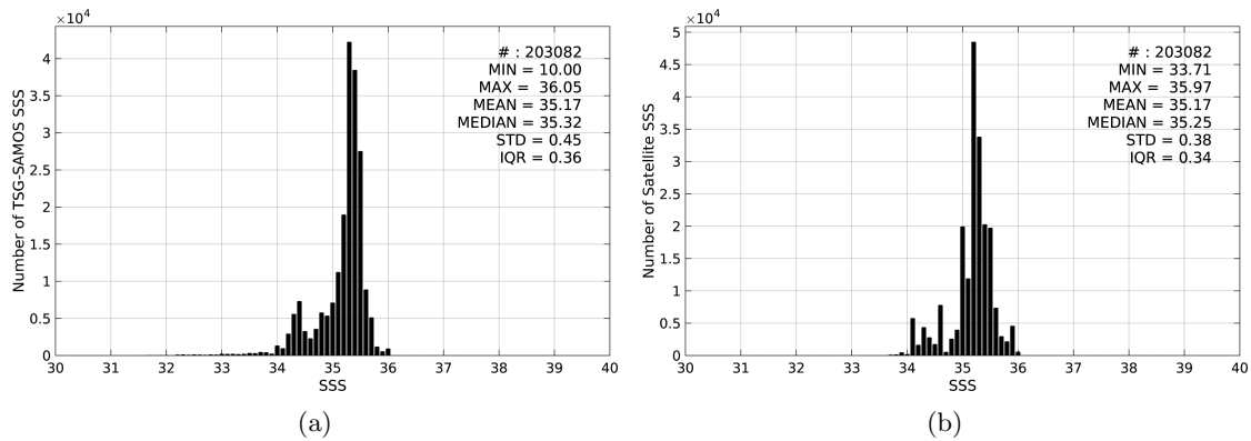
Figure 2: Histograms of SSS from TSG-SAMOS (a) and Aquarius-L4-IPRC-V4-MONTHLY (b) considering all match-up pairs per bins of 0.1 over the South Pacific Ocean Pi-MEP region and for the full satellite product period.
