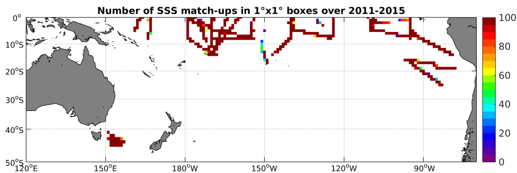
Figure 4: Number of SSS match-ups between TSG-SAMOS SSS and the Aquarius-L4-IPRC-V4-MONTHLY SSS product for the South Pacific Ocean Pi-MEP region over 1^\circ \times 1^\circ boxes and for the full satellite product period.
