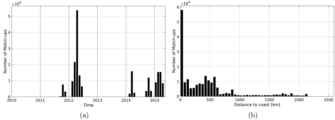
Figure 1: Number of match-ups between TSG-SAMOS and Aquarius-L4-IPRC-V4-MONTHLY SSS as a function of time (a) and as function of the distance to coast (b) over the South Pacific Ocean Pi-MEP region and for the full satellite product period.
