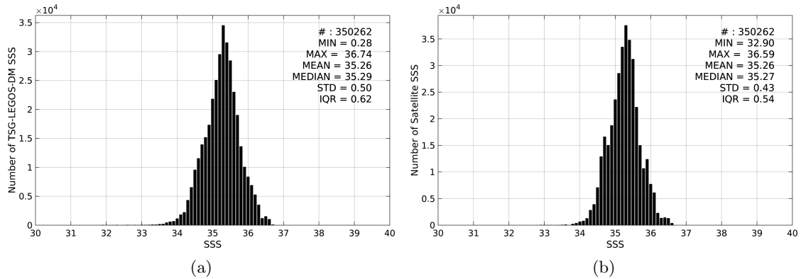
Figure 2: Histograms of SSS from TSG-LEGOS-DM (a) and Aquarius-L4-IPRC-V4-MONTHLY (b) considering all match-up pairs per bins of 0.1 over the South Pacific Ocean Pi-MEP region and for the full satellite product period.
