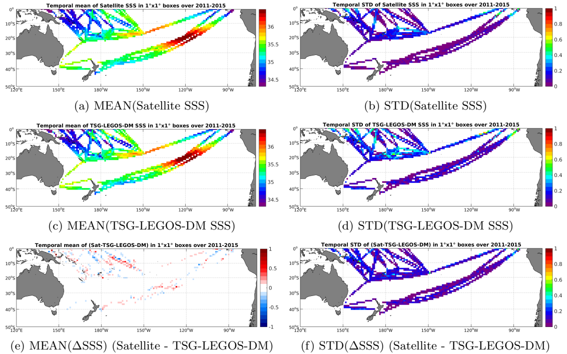
Figure 6: Temporal mean (left) and STD (right) of SSS from Aquarius-L4-IPRC-V4-MONTHLY (top), TSG-LEGOS-DM (middle), and of \Delta SSS (Satellite - TSG-LEGOS-DM). Only match-up pairs are used to generate these maps.
