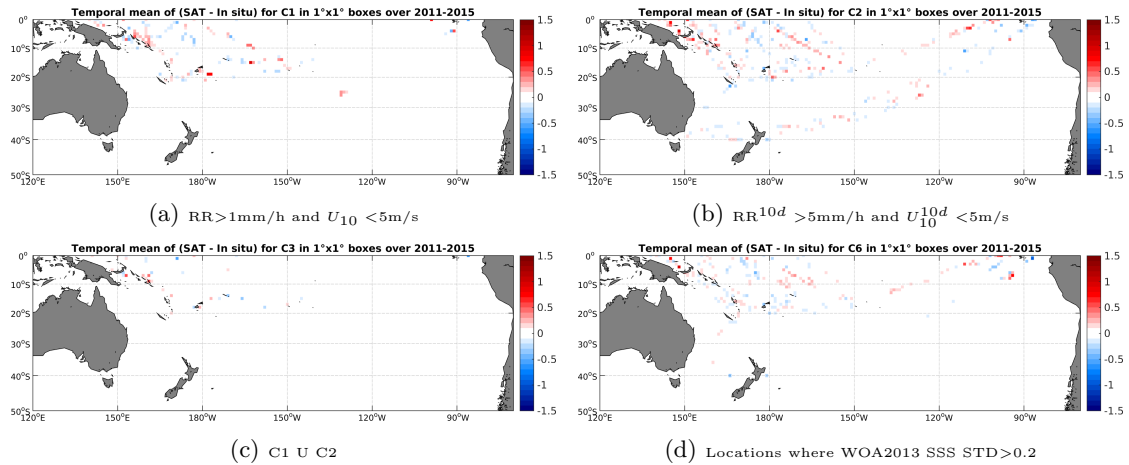
Figure 12: Temporal mean gridded over spatial boxes of size 1^\circ \times 1^\circ of \Delta SSS (Aquarius-L4-IPRC-V4-MONTHLY - TSG-LEGOS-DM) for 4 different subdatasets corresponding to: RR > 1\text{mm/h} and U_{10} < 5\text{m/s} (a), RR^{10d} > 5\text{mm/h} and U_{10}^{10d} < 5\text{m/s} (b), C1 U C2 (c), Locations where WOA2013 SSS STD > 0.2 (d).
