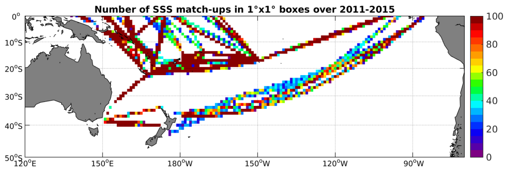
Figure 4: Number of SSS match-ups between TSG-LEGOS-DM SSS and the Aquarius-L4-IPRC-V4-MONTHLY SSS product for the South Pacific Ocean Pi-MEP region over 1^\circ \times 1^\circ boxes and for the full satellite product period.
