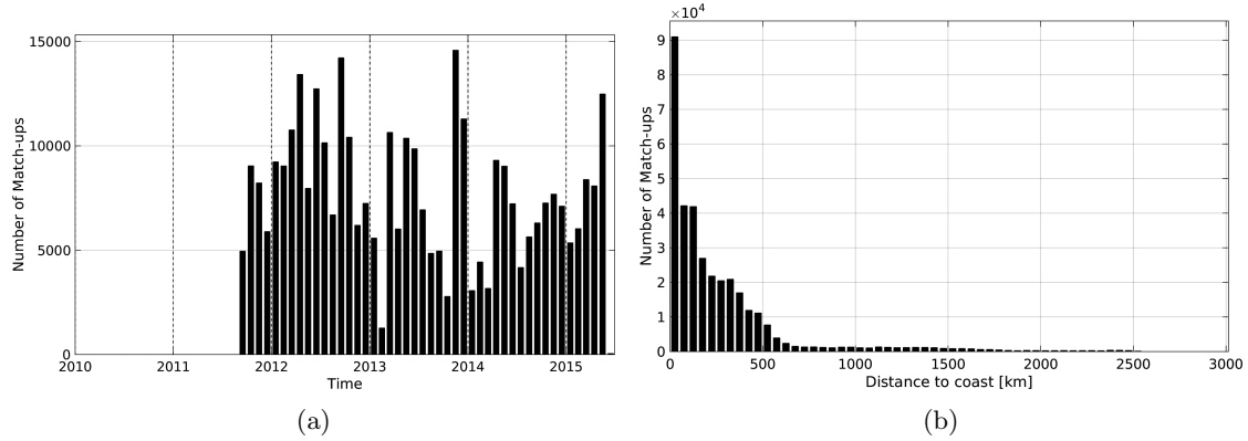
Figure 1: Number of match-ups between TSG-LEGOS-DM and Aquarius-L4-IPRC-V4-MONTHLY SSS as a function of time (a) and as function of the distance to coast (b) over the South Pacific Ocean Pi-MEP region and for the full satellite product period.
