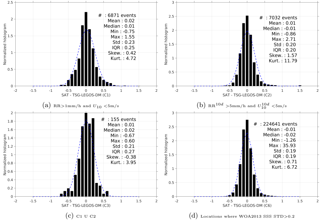
Figure 13: Normalized histogram of \Delta\text{SSS} (Aquarius-L4-IPRC-V4-MONTHLY - TSG-LEGOS-DM) for 6 different subdatasets corresponding to: \text{RR} > 1\text{mm/h} and U_{10} < 5\text{m/s} (a), \text{RR}^{10d} > 5\text{mm/h} and U_{10}^{10d} < 5\text{m/s} (b), C1 U C2 (c), Locations where WOA2013 SSS STD > 0.2 (d).
