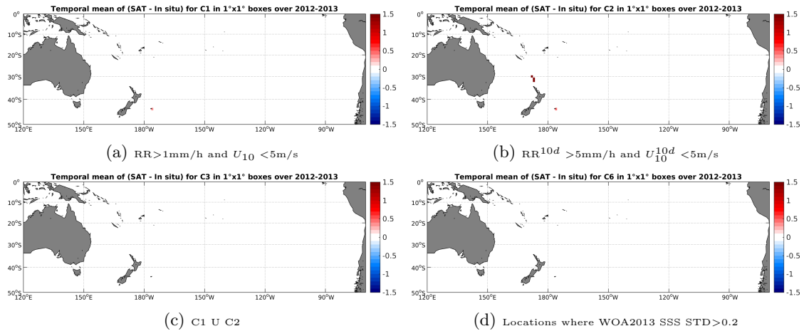
Figure 12: Temporal mean gridded over spatial boxes of size 1^\circ \times 1^\circ of \Delta SSS (Aquarius-L4-IPRC-V4-MONTHLY - TSG-GOSUD-Sailing-ship) for 4 different subdatasets corresponding to: RR > 1mm/h and U_{10} < 5\text{m/s} (a), RR^{10d} > 5\text{mm/h} and U_{10}^{10d} < 5\text{m/s} (b), C1 U C2 (c), Locations where WOA2013 SSS STD > 0.2 (d).
