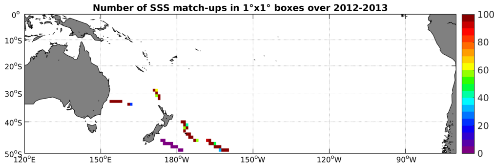
Figure 4: Number of SSS match-ups between TSG-GOSUD-Sailing-ship SSS and the Aquarius-L4-IPRC-V4-MONTHLY SSS product for the South Pacific Ocean Pi-MEP region over 1^{\circ} \times 1^{\circ} boxes and for the full satellite product period.
