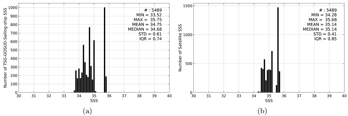
Figure 2: Histograms of SSS from TSG-GOSUD-Sailing-ship (a) and Aquarius-L4-IPRC-V4-MONTHLY (b) considering all match-up pairs per bins of 0.1 over the South Pacific Ocean Pi-MEP region and for the full satellite product period.
