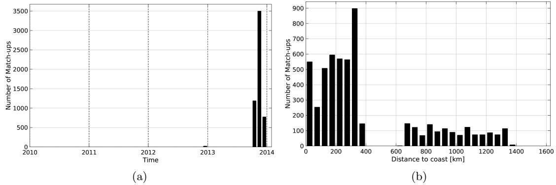
Figure 1: Number of match-ups between TSG-GOSUD-Sailing-ship and Aquarius-L4-IPRC-V4-MONTHLY SSS as a function of time (a) and as function of the distance to coast (b) over the South Pacific Ocean Pi-MEP region and for the full satellite product period.
