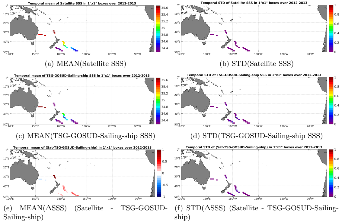
Figure 6: Temporal mean (left) and STD (right) of SSS from Aquarius-L4-IPRC-V4-MONTHLY (top), TSG-GOSUD-Sailing-ship (middle), and of \Delta SSS (Satellite - TSG-GOSUD-Sailing-ship). Only match-up pairs are used to generate these maps.
