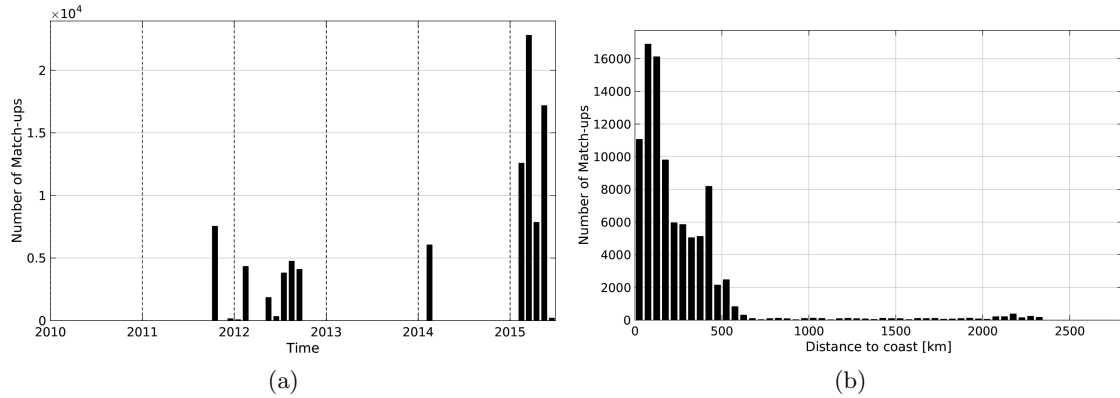
Figure 1: Number of match-ups between TSG-GOSUD-Research-vessel and Aquarius-L4-IPRC-V4-MONTHLY SSS as a function of time (a) and as function of the distance to coast (b) over the South Pacific Ocean Pi-MEP region and for the full satellite product period.
