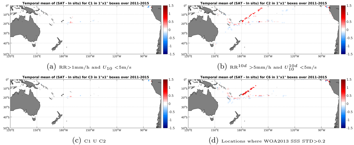
Figure 12: Temporal mean gridded over spatial boxes of size 1^\circ \times 1^\circ of \Delta SSS (Aquarius-L4-IPRC-V4-MONTHLY - TSG-GOSUD-Research-vessel) for 4 different subdatasets corresponding to: RR > 1\text{mm/h} and U_{10} < 5\text{m/s} (a), RR^{10d} > 5\text{mm/h} and U_{10}^{10d} < 5\text{m/s} (b), C1 U C2 (c), Locations where WOA2013 SSS STD > 0.2 (d).
