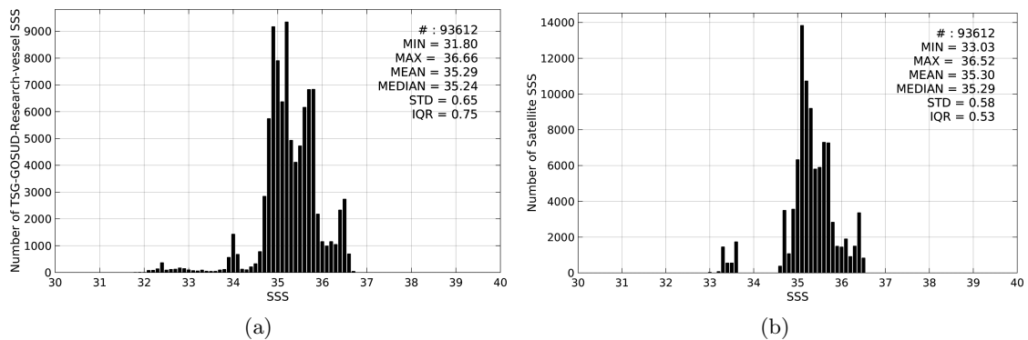
Figure 2: Histograms of SSS from TSG-GOSUD-Research-vessel (a) and Aquarius-L4-IPRC-V4-MONTHLY (b) considering all match-up pairs per bins of 0.1 over the South Pacific Ocean Pi-MEP region and for the full satellite product period.
