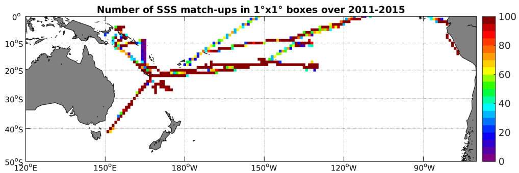
Figure 4: Number of SSS match-ups between TSG-GOSUD-Research-vessel SSS and the Aquarius-L4-IPRC-V4-MONTHLY SSS product for the South Pacific Ocean Pi-MEP region over 1°x1° boxes and for the full satellite product period.
