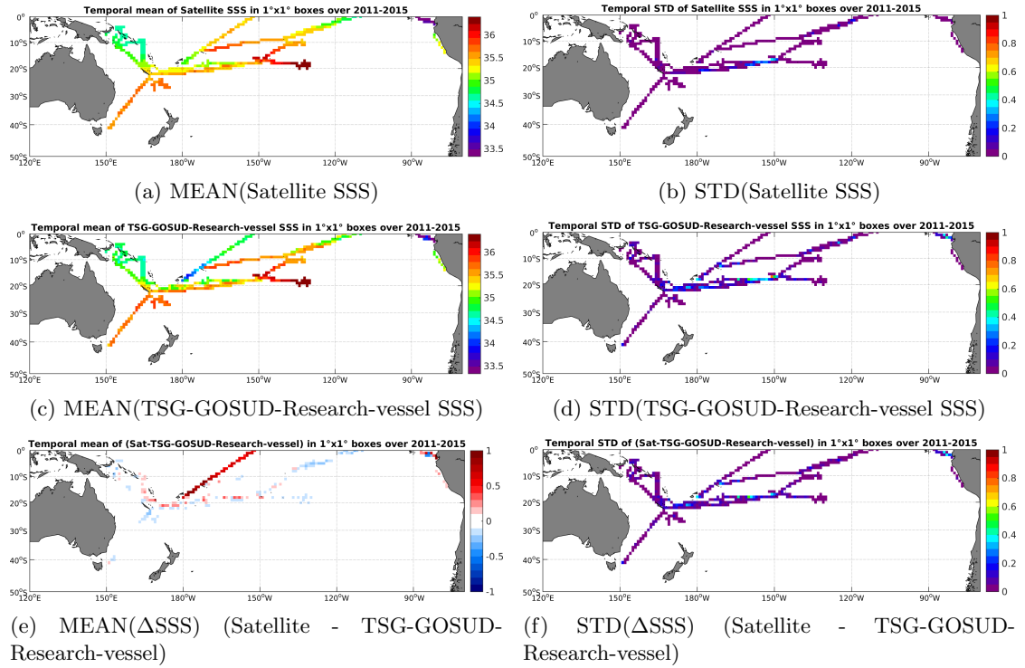
Figure 6: Temporal mean (left) and STD (right) of SSS from Aquarius-L4-IPRC-V4-MONTHLY (top), TSG-GOSUD-Research-vessel (middle), and of \Delta SSS (Satellite - TSG-GOSUD-Research-vessel). Only match-up pairs are used to generate these maps.
