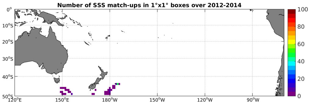
Figure 4: Number of SSS match-ups between Sea mammals SSS and the Aquarius-L4-IPRC-V4-MONTHLY SSS product for the South Pacific Ocean Pi-MEP region over 1^\circ \times 1^\circ boxes and for the full satellite product period.
