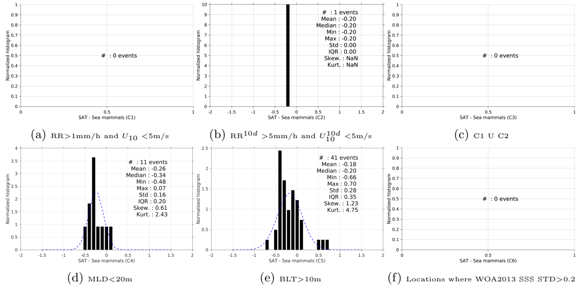
Figure 13: Normalized histogram of \Delta SSS (Aquarius-L4-IPRC-V4-MONTHLY - Sea mammals) for 6 different subdatasets corresponding to: RR > 1\text{mm/h} and U_{10} < 5\text{m/s} (a), RR^{10d} > 5\text{mm/h} and U_{10}^{10d} < 5\text{m/s} (b), C1 U C2 (c), MLD < 20\text{m} (d), BLT > 10\text{m} (e), Locations where WOA2013 SSS STD > 0.2 (f).
