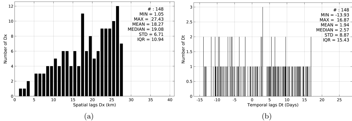
Figure 5: Histograms of the spatial (a) and temporal (b) lags between the time of the Sea mammals measurements and the date of the corresponding Aquarius-L4-IPRC-V4-MONTHLY SSS product.
