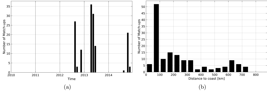
Figure 1: Number of match-ups between Sea mammals and Aquarius-L4-IPRC-V4-MONTHLY SSS as a function of time (a) and as function of the distance to coast (b) over the South Pacific Ocean Pi-MEP region and for the full satellite product period.
