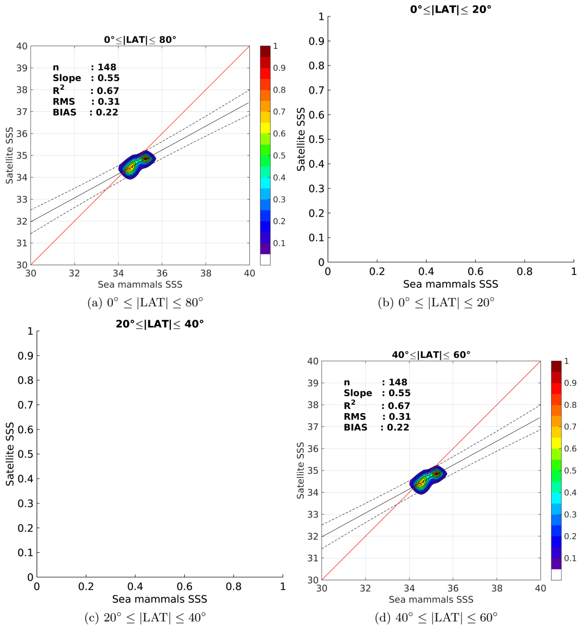
Figure 9: Contour maps of the concentration of Aquarius-L4-IPRC-V4-MONTHLY SSS (y-axis) versus Sea mammals SSS (x-axis) at match-up pairs for different latitude bands. For each plot, the red line shows x=y . The black thin and dashed lines indicate a linear fit through the data cloud and the \pm 95\% confidence levels, respectively. The number match-up pairs n , the slope and R^2 coefficient of the linear fit, the root mean square (RMS) and the mean bias between satellite and in situ data are indicated for each latitude band in each plots.
