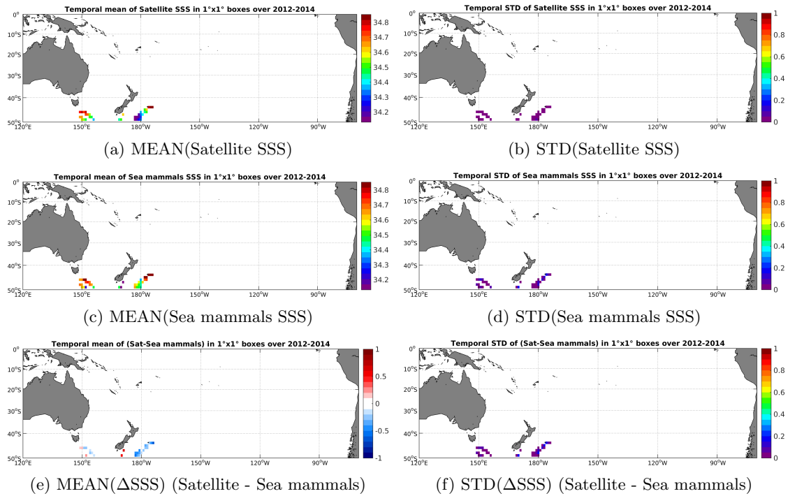
Figure 6: Temporal mean (left) and STD (right) of SSS from Aquarius-L4-IPRC-V4-MONTHLY (top), Sea mammals (middle), and of \Delta SSS (Satellite - Sea mammals). Only match-up pairs are used to generate these maps.
