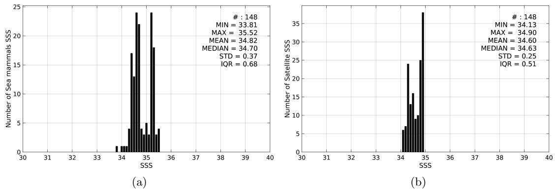
Figure 2: Histograms of SSS from Sea mammals (a) and Aquarius-L4-IPRC-V4-MONTHLY (b) considering all match-up pairs per bins of 0.1 over the South Pacific Ocean Pi-MEP region and for the full satellite product period.
