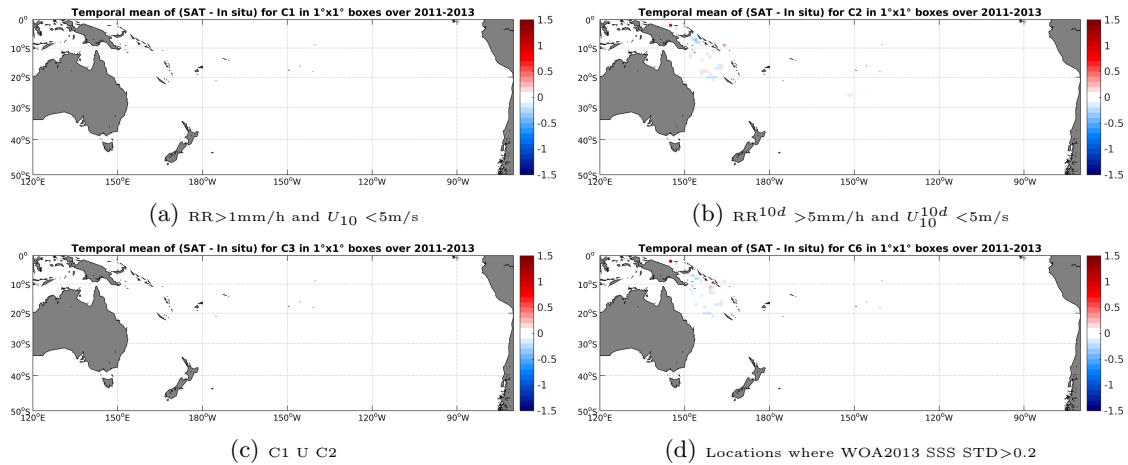
Figure 11: Temporal mean gridded over spatial boxes of size 1^\circ \times 1^\circ of \Delta SSS (Aquarius-L4-IPRC-V4-MONTHLY - Surface drifters) for 4 different subdatasets corresponding to: RR > 1\text{mm/h} and U_{10} < 5\text{m/s} (a), RR^{10d} > 5\text{mm/h} and U_{10}^{10d} < 5\text{m/s} (b), C1 U C2 (c), Locations where WOA2013 SSS STD > 0.2 (d).
