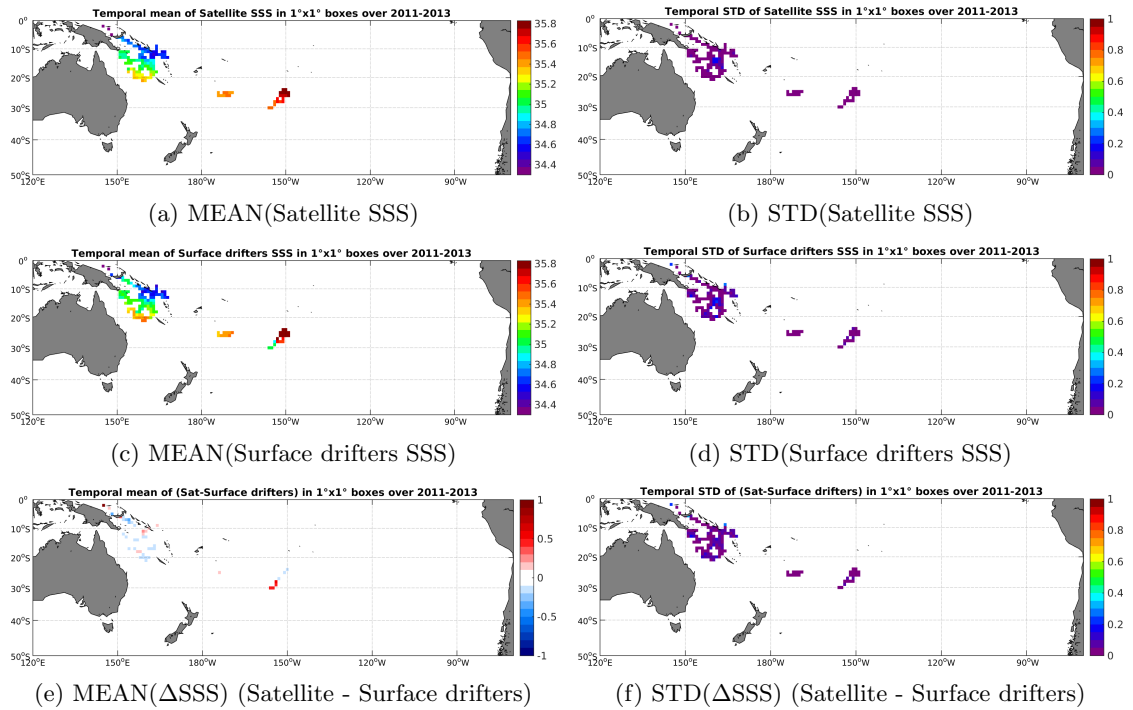
Figure 5: Temporal mean (left) and STD (right) of SSS from Aquarius-L4-IPRC-V4-MONTHLY (top), Surface drifters (middle), and of \Delta SSS (Satellite - Surface drifters). Only match-up pairs are used to generate these maps.
