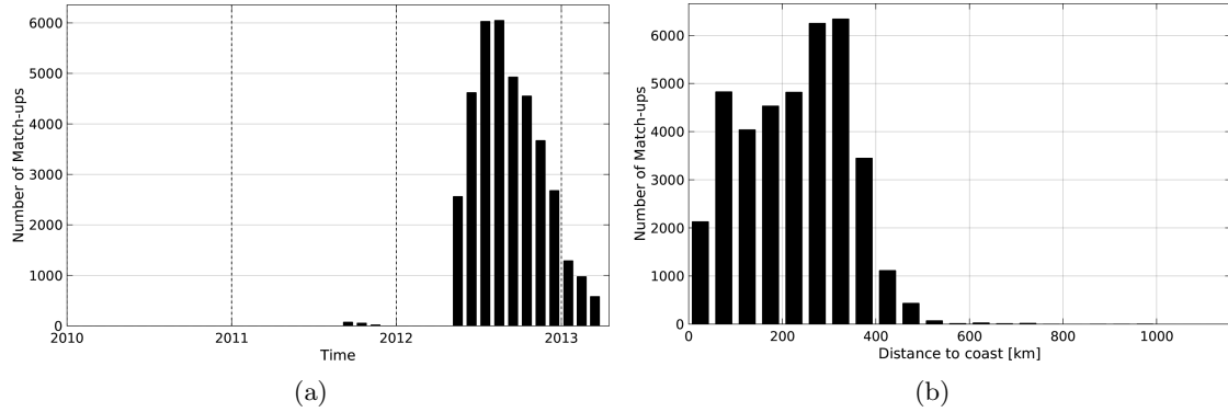
Figure 1: Number of match-ups between Surface drifters and Aquarius-L4-IPRC-V4-MONTHLY SSS as a function of time (a) and as function of the distance to coast (b) over the South Pacific Ocean Pi-MEP region and for the full satellite product period.
