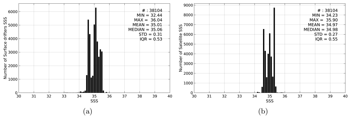
Figure 2: Histograms of SSS from Surface drifters (a) and Aquarius-L4-IPRC-V4-MONTHLY (b) considering all match-up pairs per bins of 0.1 over the South Pacific Ocean Pi-MEP region and for the full satellite product period.
