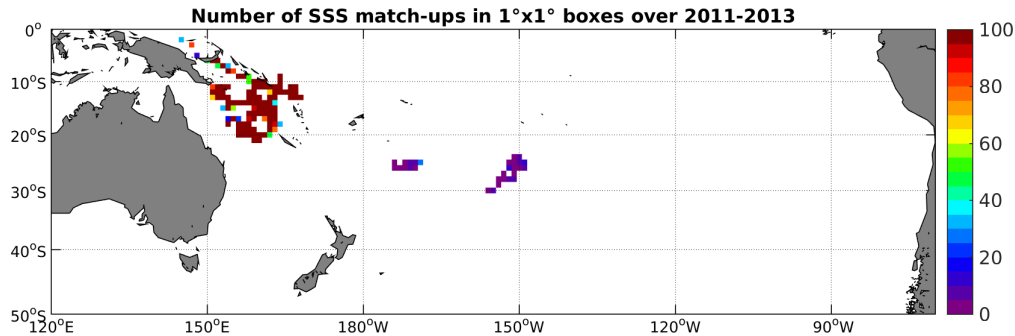
Figure 3: Number of SSS match-ups between Surface drifters SSS and the Aquarius-L4-IPRC-V4-MONTHLY SSS product for the South Pacific Ocean Pi-MEP region over 1^\circ \times 1^\circ boxes and for the full satellite product period.
