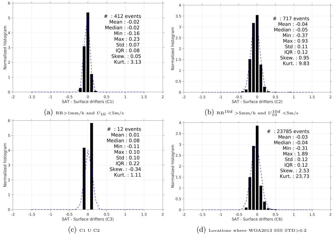
Figure 12: Normalized histogram of \Delta SSS (Aquarius-L4-IPRC-V4-MONTHLY - Surface drifters) for 6 different subdatasets corresponding to: RR > 1mm/h and U_{10} < 5 m/s (a), RR^{10d} > 5 mm/h and U_{10}^{10d} < 5 m/s (b), C1 U C2 (c), Locations where WOA2013 SSS STD > 0.2 (d).
