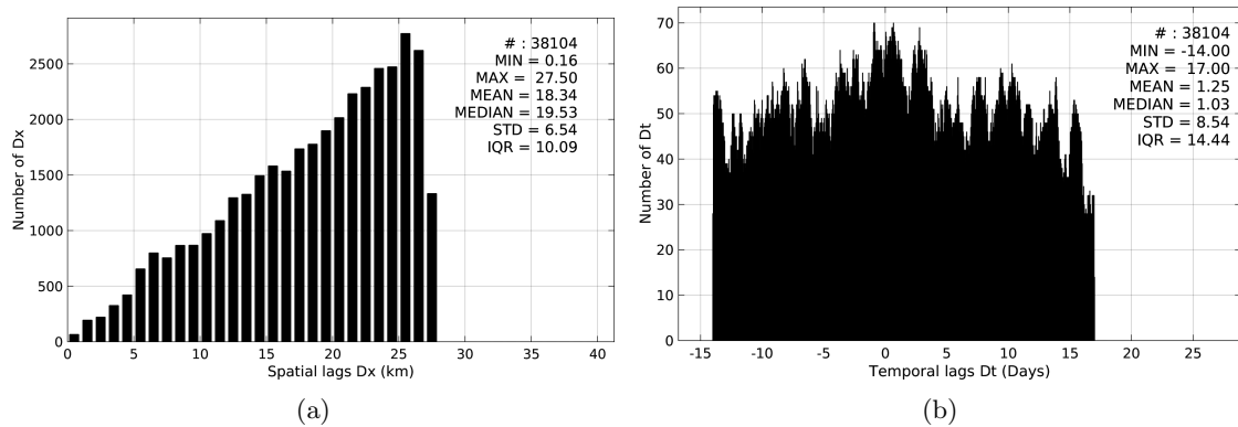
Figure 4: Histograms of the spatial (a) and temporal (b) lags between the time of the Surface drifters measurements and the date of the corresponding Aquarius-L4-IPRC-V4-MONTHLY SSS product.
