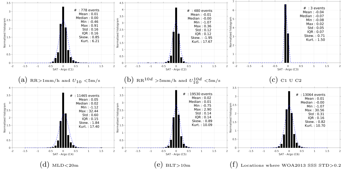
Figure 13: Normalized histogram of \Delta SSS (Aquarius-L4-IPRC-V4-MONTHLY - Argo) for 6 different subdatasets corresponding to: RR>1mm/h and U_{10} < 5 m/s (a), RR 10d >5mm/h and U_{10}^{10d} < 5 m/s (b), C1 U C2 (c),MLD<20m (d),BLT>10m (e),Locations where WOA2013 SSS STD>0.2 (f).
