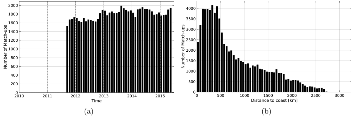
Figure 1: Number of match-ups between Argo and Aquarius-L4-IPRC-V4-MONTHLY SSS as a function of time (a) and as function of the distance to coast (b) over the South Pacific Ocean Pi-MEP region and for the full satellite product period.
