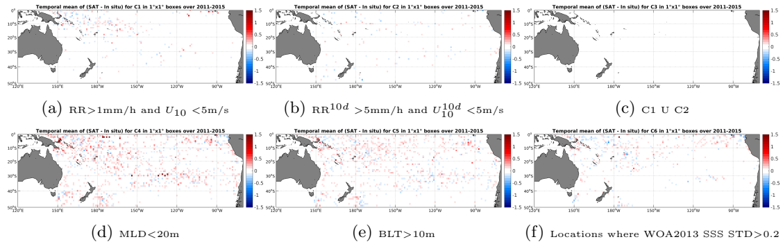
Figure 12: Temporal mean gridded over spatial boxes of size 1^\circ \times 1^\circ of \Delta SSS (Aquarius-L4-IPRC-V4-MONTHLY - Argo) for 6 different subdatasets corresponding to:RR >1 mm/h and U_{10} < 5 m/s (a), RR^{10d} > 5 mm/h and U_{10}^{10d} < 5 m/s (b), C1 U C2 (c),MLD <20 m (d),BLT >10 m (e),Locations where WOA2013 SSS STD >0.2 (f).
