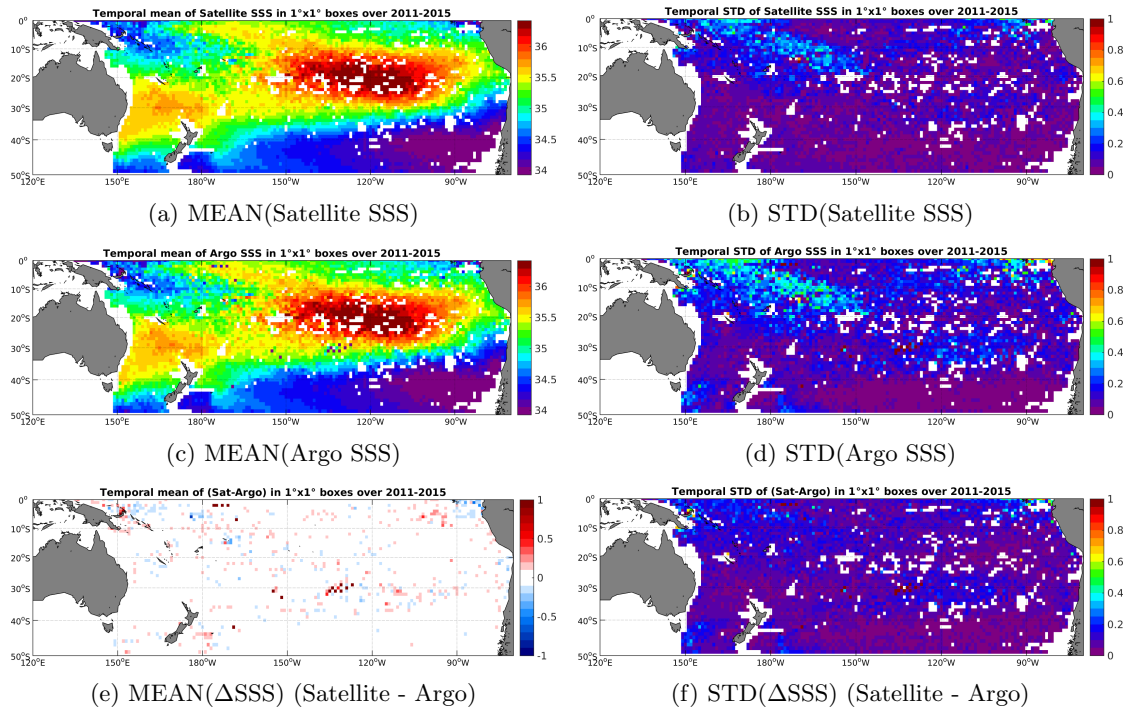
Figure 6: Temporal mean (left) and STD (right) of SSS from Aquarius-L4-IPRC-V4-MONTHLY (top), Argo (middle), and of \Delta SSS (Satellite - Argo). Only match-up pairs are used to generate these maps.
