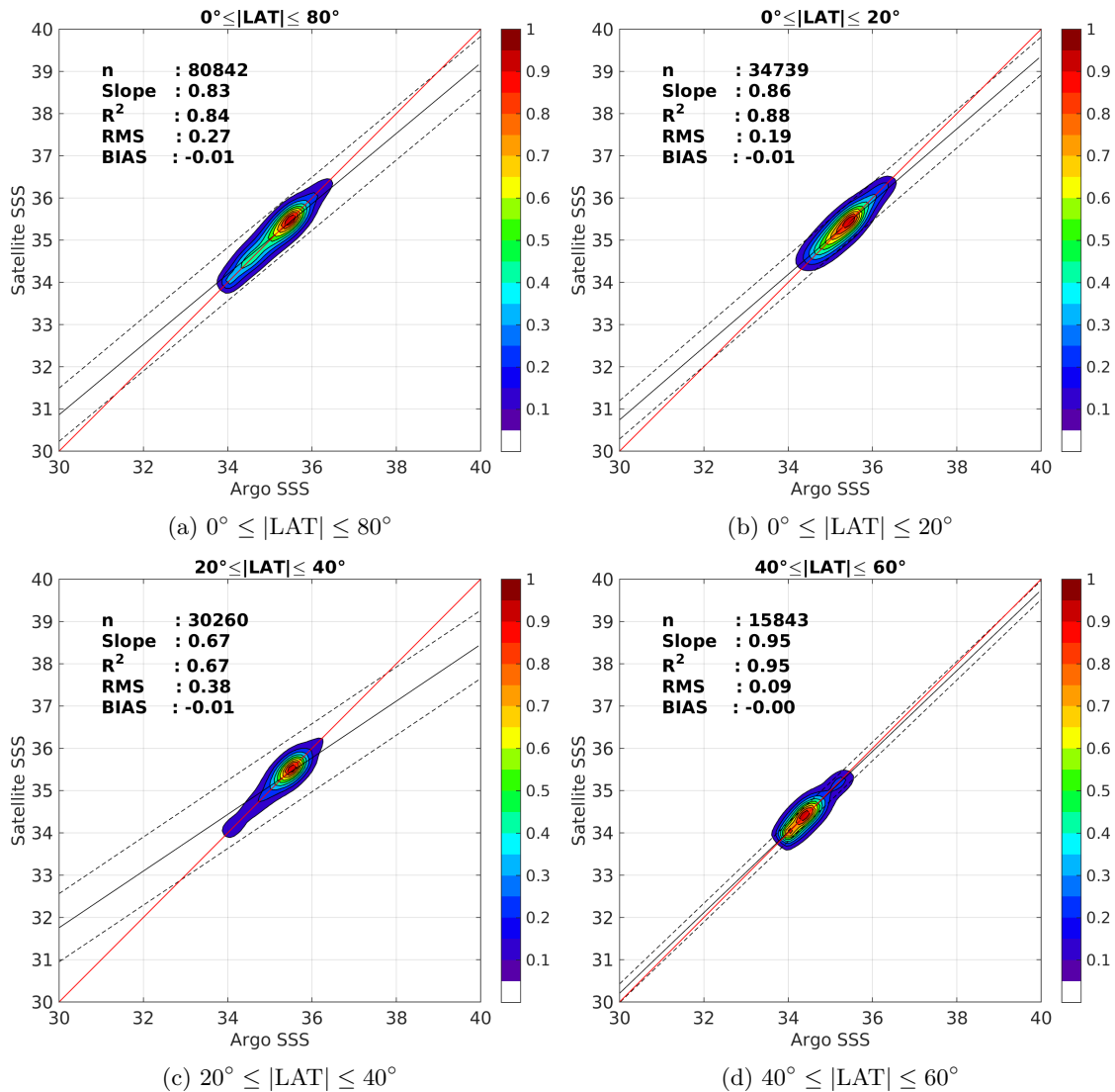
Figure 9: Contour maps of the concentration of Aquarius-L4-IPRC-V4-MONTHLY SSS (y-axis) versus Argo SSS (x-axis) at match-up pairs for different latitude bands. For each plot, the red line shows x=y . The black thin and dashed lines indicate a linear fit through the data cloud and the \pm 95\% confidence levels, respectively. The number match-up pairs n , the slope and R^2 coefficient of the linear fit, the root mean square (RMS) and the mean bias between satellite and in situ data are indicated for each latitude band in each plots.
