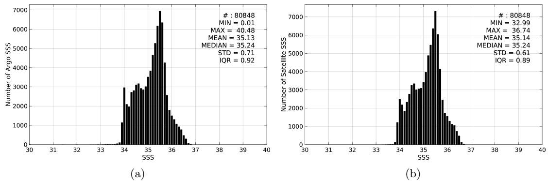
Figure 2: Histograms of SSS from Argo (a) and Aquarius-L4-IPRC-V4-MONTHLY (b) considering all match-up pairs per bins of 0.1 over the South Pacific Ocean Pi-MEP region and for the full satellite product period.
