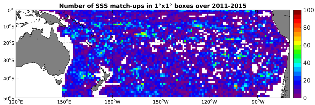
Figure 4: Number of SSS match-ups between Argo SSS and the Aquarius-L4-IPRC-V4-MONTHLY SSS product for the South Pacific Ocean Pi-MEP region over 1^{\circ} \times 1^{\circ} boxes and for the full satellite product period.
