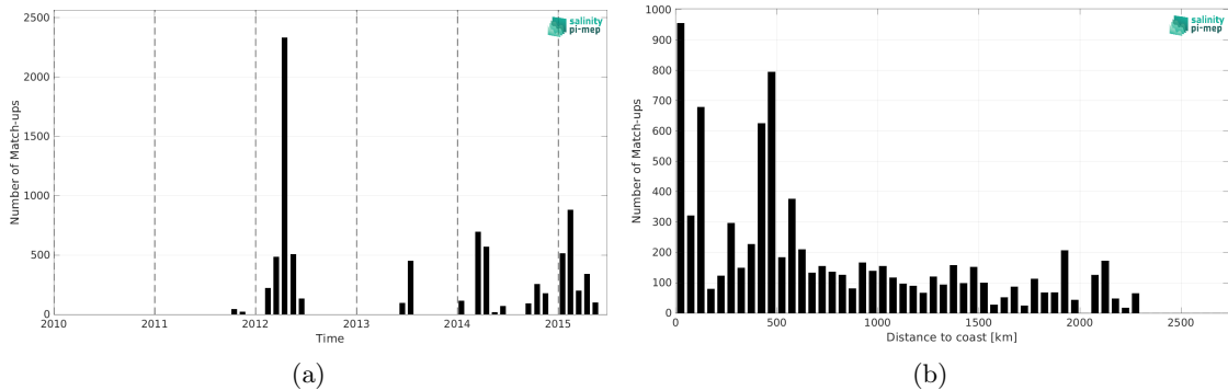
Figure 2: Number of match-ups between TSG (SAMOS) and Aquarius SSS L3 OR v5 - 7-Day running (NASA-GSFC) SSS as a function of time (a) and as function of the distance to coast (b) over the South Pacific Ocean Pi-MEP region and for the full satellite product period.
