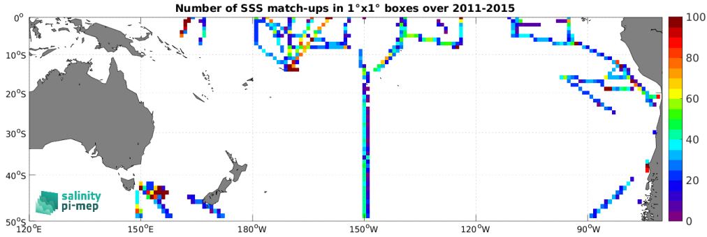
Figure 4: Number of SSS match-ups between TSG (SAMOS) SSS and the Aquarius SSS L3 OR v5 - 7-Day running (NASA-GSFC) SSS product for the South Pacific Ocean Pi-MEP region over 1^\circ \times 1^\circ boxes and for the full satellite product period.
