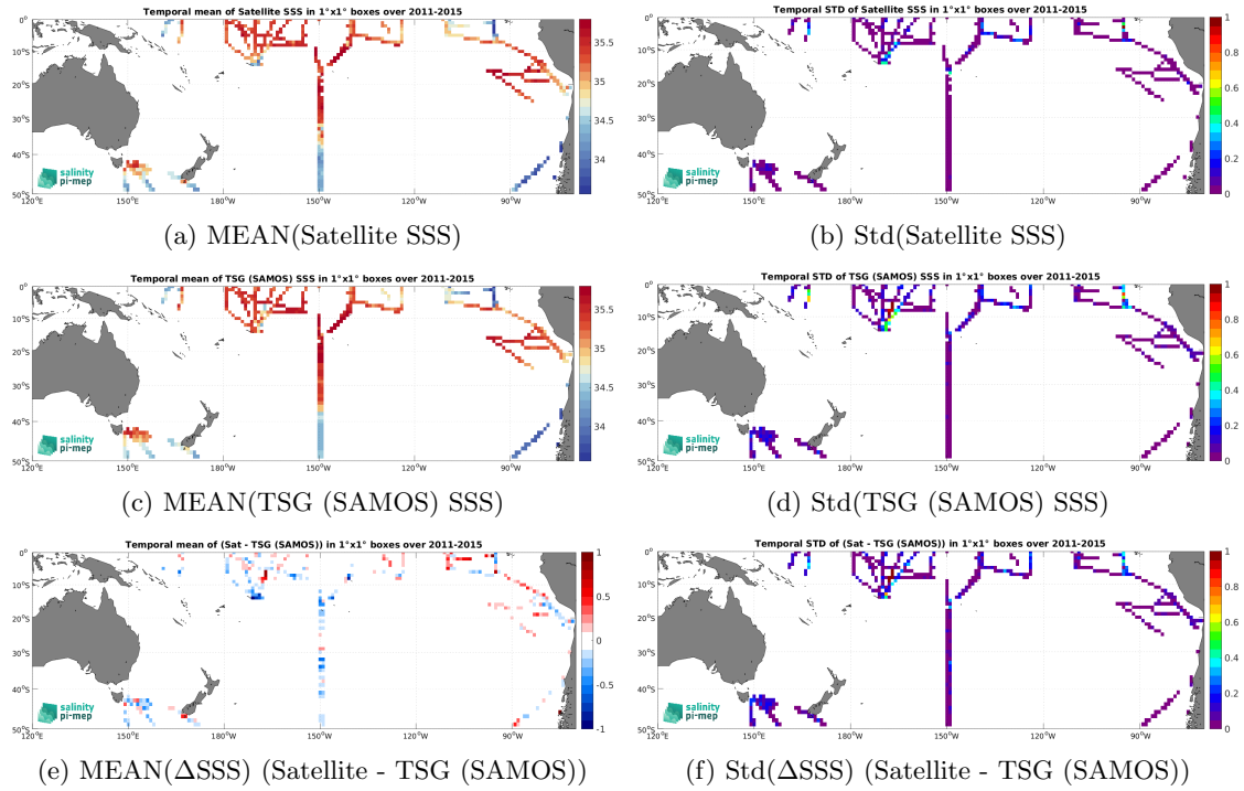
Figure 6: Temporal mean (left) and Std (right) of SSS from Aquarius SSS L3 OR v5 - 7-Day running (NASA-GSFC) (top), TSG (SAMOS) (middle), and of \Delta SSS (Satellite - TSG (SAMOS)). Only match-up pairs are used to generate these maps.
