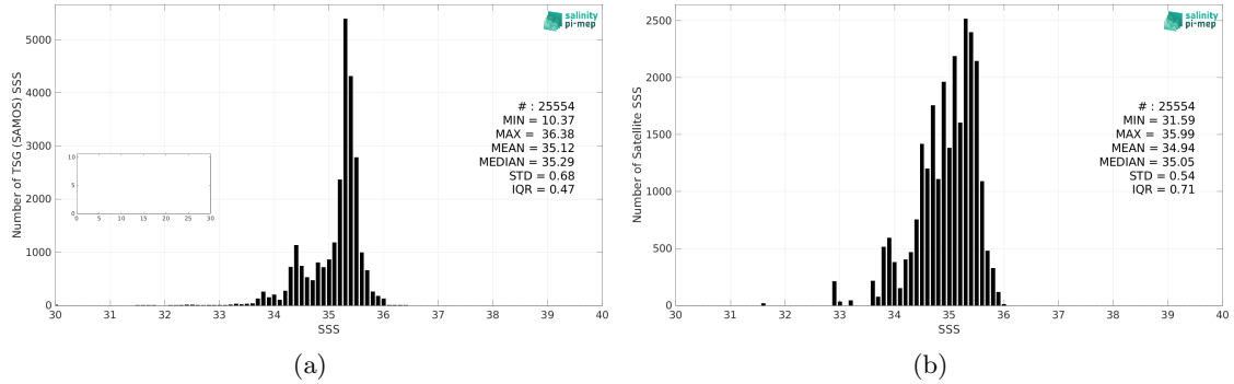
Figure 2: Histograms of SSS from TSG (SAMOS) (a) and Aquarius SSS L3 OR v5 - 7-Day running (NASA-GSFC) (b) considering all match-up pairs per bins of 0.1 over the South Pacific Ocean Pi-MEP region and for the full satellite product period.
