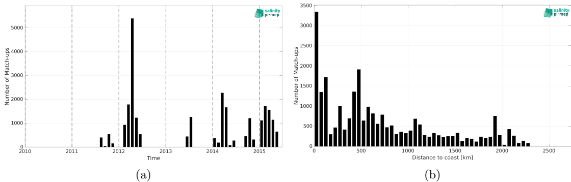
Figure 1: Number of match-ups between TSG (SAMOS) and Aquarius SSS L3 OR v5 - 7-Day running (NASA-GSFC) SSS as a function of time (a) and as function of the distance to coast (b) over the South Pacific Ocean Pi-MEP region and for the full satellite product period.
