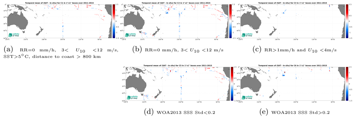
Figure 12: Temporal mean gridded over spatial boxes of size 1^\circ \times 1^\circ of \Delta\text{SSS} (Aquarius SSS L3 OR v5 - 7-Day running (NASA-GSFC) - TSG (SAMOS)) for 5 different subdatasets corresponding to:RR=0 mm/h, 3 < U_{10} < 12 m/s, SST >5^\circ\text{C} , distance to coast > 800 km (a), RR=0 mm/h, 3 < U_{10} < 12 m/s (b), RR >1 mm/h and U_{10} < 4 m/s (c), WOA2013 SSS Std <0.2 (d), WOA2013 SSS Std >0.2 (e).
