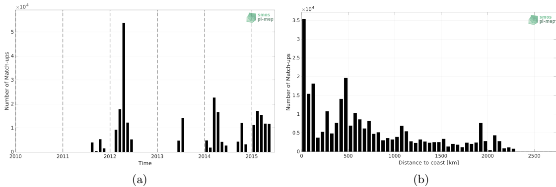
Figure 1: Number of match-ups between TSG (SAMOS) and Aquarius SSS L3 OR v5 - 7-Day running (NASA-GSFC) SSS as a function of time (a) and as function of the distance to coast (b) over the South Pacific Ocean Pi-MEP region and for the full satellite product period.
