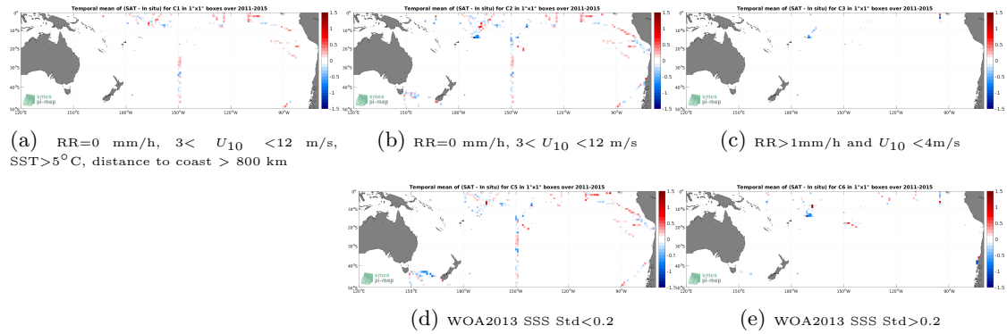
Figure 12: Temporal mean gridded over spatial boxes of size 1^\circ \times 1^\circ of \Delta SSS (Aquarius SSS L3 OR v5 - 7-Day running (NASA-GSFC) - TSG (SAMOS)) for 5 different subdatasets corresponding to:RR=0 mm/h, 3 < U_{10} < 12 m/s, SST >5^\circ C, distance to coast > 800 km (a), RR=0 mm/h, 3 < U_{10} < 12 m/s (b), RR >1 mm/h and U_{10} < 4 m/s (c), WOA2013 SSS Std <0.2 (d), WOA2013 SSS Std >0.2 (e).
