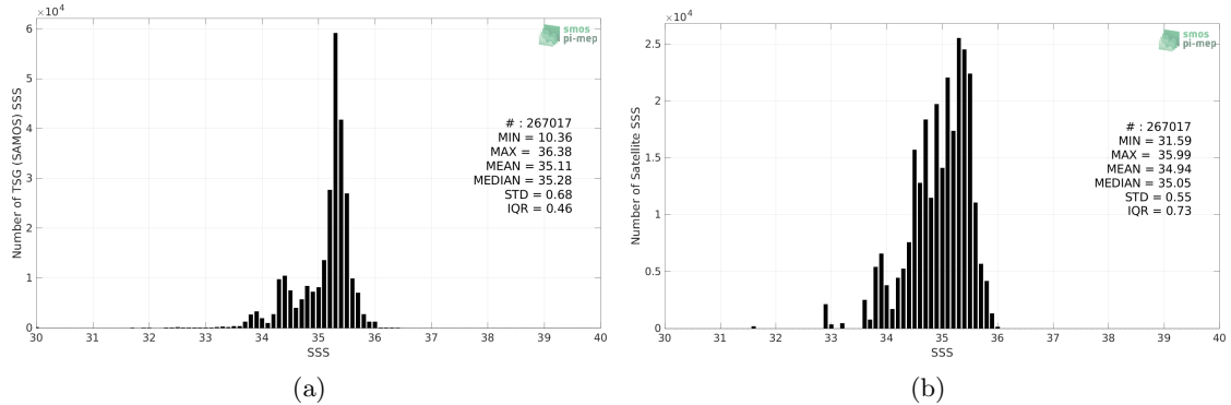
Figure 2: Histograms of SSS from TSG (SAMOS) (a) and Aquarius SSS L3 OR v5 - 7-Day running (NASA-GSFC) (b) considering all match-up pairs per bins of 0.1 over the South Pacific Ocean Pi-MEP region and for the full satellite product period.
