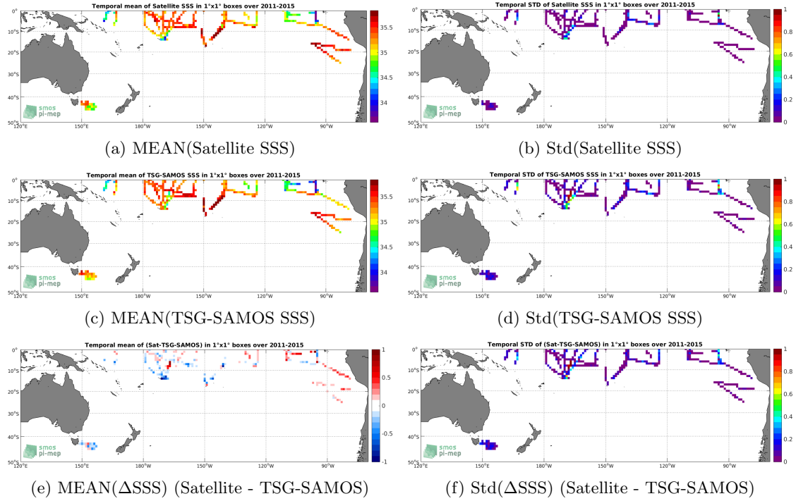
Figure 6: Temporal mean (left) and Std (right) of SSS from Aquarius-L3-OR-V5-7DAY-RUNNING-1DEG (top), TSG-SAMOS (middle), and of \Delta SSS (Satellite - TSG-SAMOS). Only match-up pairs are used to generate these maps.
