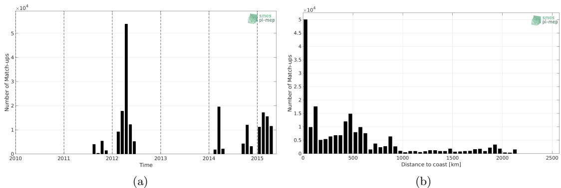
Figure 1: Number of match-ups between TSG-SAMOS and Aquarius-L3-OR-V5-7DAY-RUNNING-1DEG SSS as a function of time (a) and as function of the distance to coast (b) over the South Pacific Ocean Pi-MEP region and for the full satellite product period.
