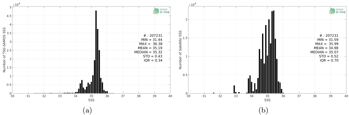
Figure 2: Histograms of SSS from TSG-SAMOS (a) and Aquarius-L3-OR-V5-7DAY-RUNNING-1DEG (b) considering all match-up pairs per bins of 0.1 over the South Pacific Ocean Pi-MEP region and for the full satellite product period.
