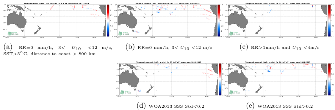
Figure 12: Temporal mean gridded over spatial boxes of size 1^\circ \times 1^\circ of \Delta SSS (Aquarius-L3-OR-V5-7DAY-RUNNING-1DEG - TSG-SAMOS) for 5 different subdatasets corresponding to:RR=0 mm/h, 3 < U_{10} < 12 m/s, SST >5^\circ C, distance to coast > 800 km (a), RR=0 mm/h, 3 < U_{10} < 12 m/s (b), RR >1 mm/h and U_{10} < 4 m/s (c), WOA2013 SSS Std <0.2 (d), WOA2013 SSS Std >0.2 (e).
