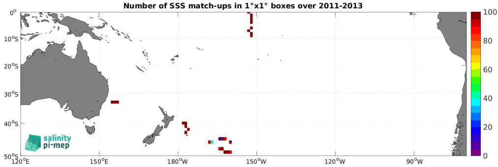
Figure 5: Number of SSS match-ups between TSG (GOSUD-Sailing-ship) SSS and the Aquarius SSS L3 OR v5 - 7-Day running (NASA-GSFC) SSS product for the South Pacific Ocean Pi-MEP region over 1^\circ \times 1^\circ boxes and for the full satellite product period.
