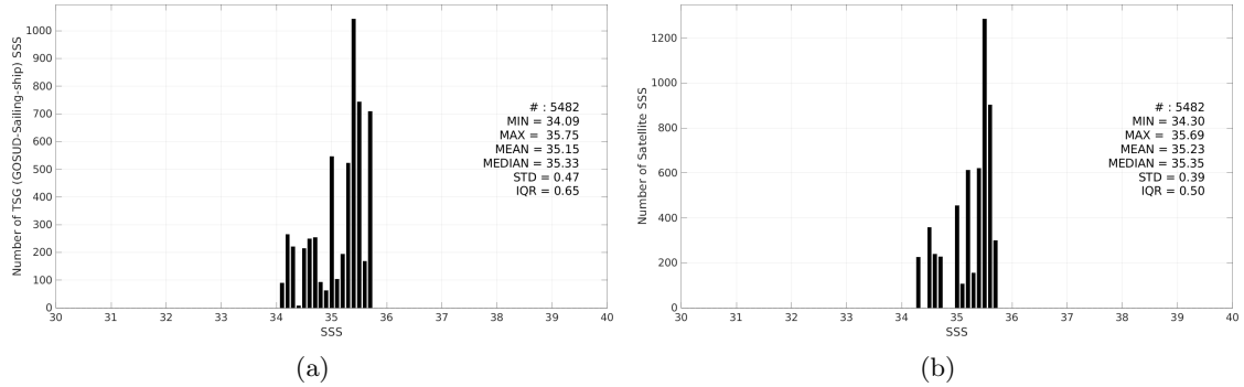
Figure 3: Histograms of SSS from TSG (GOSUD-Sailing-ship) (a) and Aquarius SSS L3 OR v5 - 7-Day running (NASA-GSFC) (b) considering all match-up pairs per bins of 0.1 over the South Pacific Ocean Pi-MEP region and for the full satellite product period.
