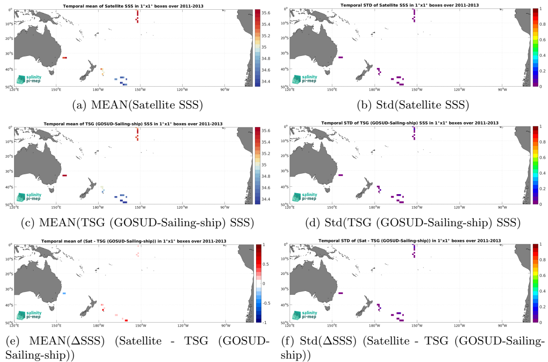
Figure 7: Temporal mean (left) and Std (right) of SSS from Aquarius SSS L3 OR v5 - 7-Day running (NASA-GSFC) (top), TSG (GOSUD-Sailing-ship) (middle), and of \Delta SSS (Satellite - TSG (GOSUD-Sailing-ship)). Only match-up pairs are used to generate these maps.
