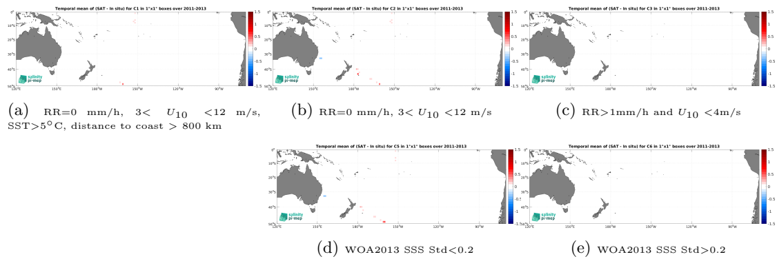
Figure 14: Temporal mean gridded over spatial boxes of size 1^\circ \times 1^\circ of \Delta SSS (Aquarius SSS L3 OR v5 - 7-Day running (NASA-GSFC) - TSG (GOSUD-Sailing-ship)) for 5 different subdatasets corresponding to:RR=0 mm/h, 3 < U_{10} < 12 m/s, SST >5^\circ\text{C} , distance to coast > 800 km (a), RR=0 mm/h, 3 < U_{10} < 12 m/s (b), RR >1 mm/h and U_{10} < 4 m/s (c), WOA2013 SSS Std <0.2 (d), WOA2013 SSS Std >0.2 (e).
