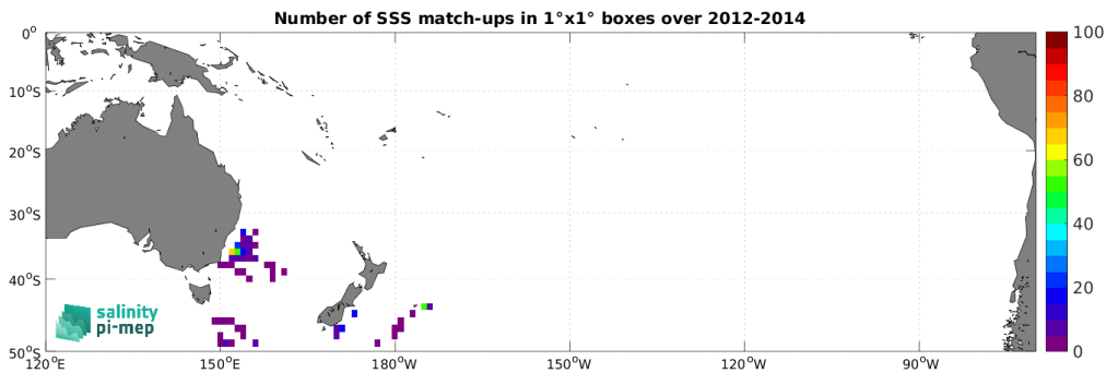
Figure 5: Number of SSS match-ups between Marine mammals SSS and the Aquarius SSS L3 OR v5 - 7-Day running (NASA-GSFC) SSS product for the South Pacific Ocean Pi-MEP region over 1^\circ \times 1^\circ boxes and for the full satellite product period.
