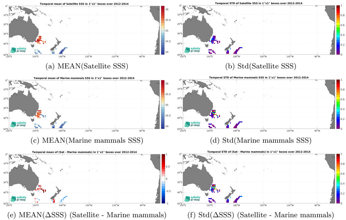
Figure 6: Temporal mean (left) and Std (right) of SSS from Aquarius SSS L3 OR v5 - 7-Day running (NASA-GSFC) (top), Marine mammals (middle), and of \Delta SSS (Satellite - Marine mammals). Only match-up pairs are used to generate these maps.
