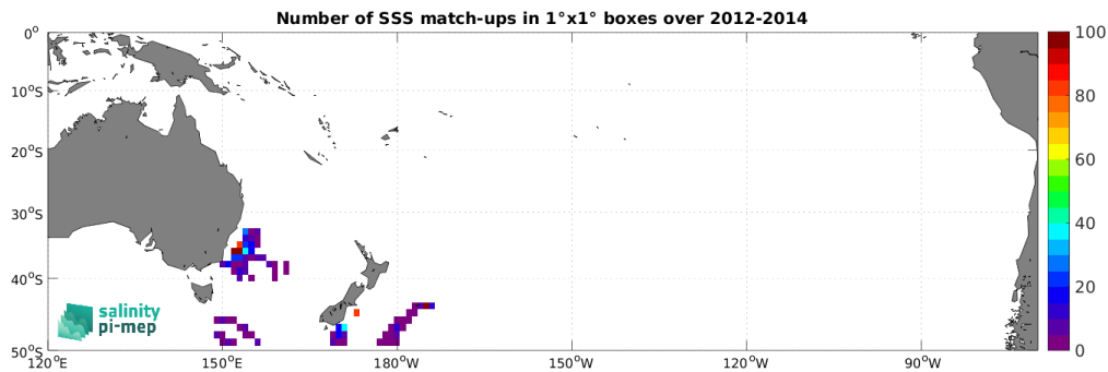
Figure 4: Number of SSS match-ups between Marine mammals SSS and the Aquarius SSS L3 OR v5 - 7-Day running (NASA-GSFC) SSS product for the South Pacific Ocean Pi-MEP region over 1^\circ \times 1^\circ boxes and for the full satellite product period.
