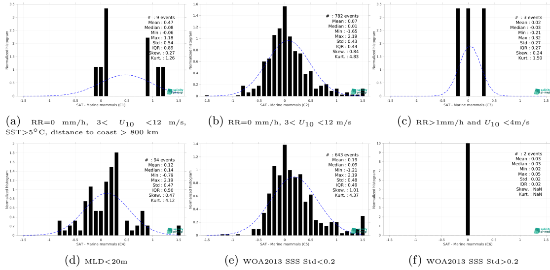
Figure 13: Normalized histogram of \Delta\text{SSS} (Aquarius SSS L3 OR v5 - 7-Day running (NASA-GSFC) - Marine mammals) for 6 different subdatasets corresponding to: RR=0 mm/h, 3 < U_{10} < 12 m/s, SST>5°C, distance to coast > 800 km (a), RR=0 mm/h, 3 < U_{10} < 12 m/s (b), RR>1mm/h and U_{10} < 4 m/s (c), MLD<20m (d), WOA2013 SSS Std<0.2 (e), WOA2013 SSS Std>0.2 (f).
