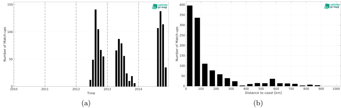
Figure 1: Number of match-ups between Marine mammals and Aquarius SSS L3 OR v5 - 7-Day running (NASA-GSFC) SSS as a function of time (a) and as function of the distance to coast (b) over the South Pacific Ocean Pi-MEP region and for the full satellite product period.
