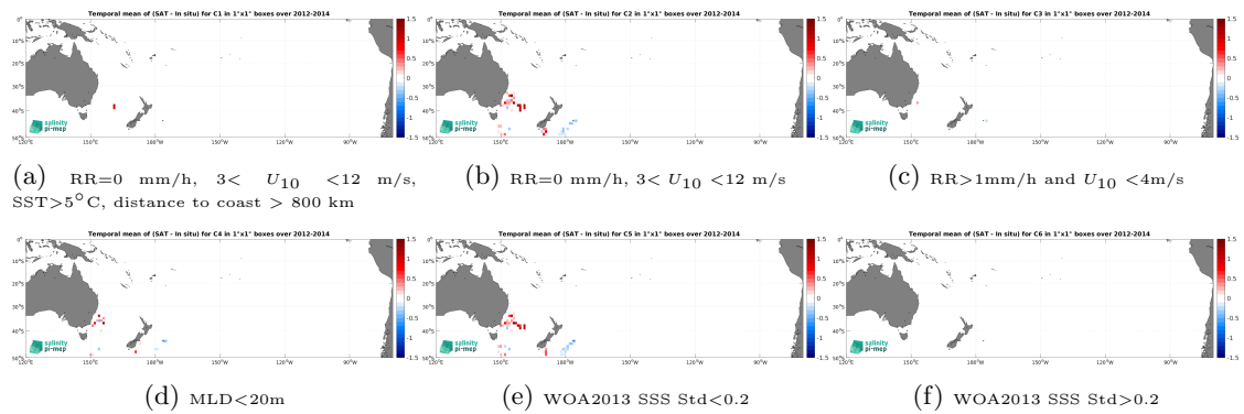
Figure 12: Temporal mean gridded over spatial boxes of size 1^\circ \times 1^\circ of \Delta SSS (Aquarius SSS L3 OR v5 - 7-Day running (NASA-GSFC) - Marine mammals) for 6 different subdatasets corresponding to:RR=0 mm/h, 3 < U_{10} < 12 m/s, SST >5^\circ C, distance to coast > 800 km (a), RR=0 mm/h, 3 < U_{10} < 12 m/s (b), RR >1 mm/h and U_{10} < 4 m/s (c),MLD <20 m (d),WOA2013 SSS Std <0.2 (e),WOA2013 SSS Std >0.2 (f).
