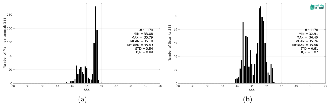
Figure 2: Histograms of SSS from Marine mammals (a) and Aquarius SSS L3 OR v5 - 7-Day running (NASA-GSFC) (b) considering all match-up pairs per bins of 0.1 over the South Pacific Ocean Pi-MEP region and for the full satellite product period.
