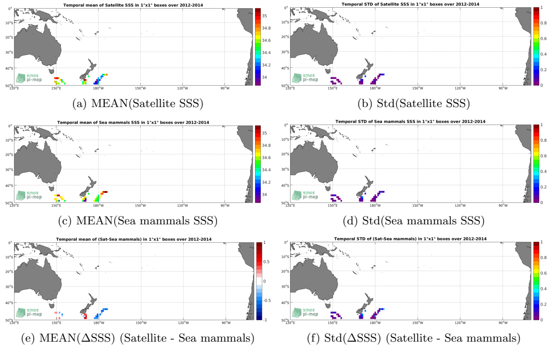
Figure 6: Temporal mean (left) and Std (right) of SSS from Aquarius-L3-OR-V5-7DAY-RUNNING-1DEG (top), Sea mammals (middle), and of \Delta SSS (Satellite - Sea mammals). Only match-up pairs are used to generate these maps.
