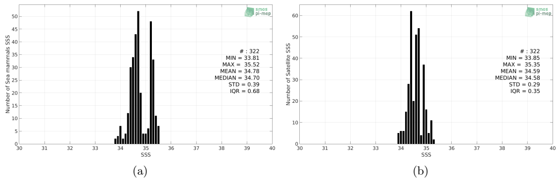
Figure 2: Histograms of SSS from Sea mammals (a) and Aquarius-L3-OR-V5-7DAY-RUNNING-1DEG (b) considering all match-up pairs per bins of 0.1 over the South Pacific Ocean Pi-MEP region and for the full satellite product period.
