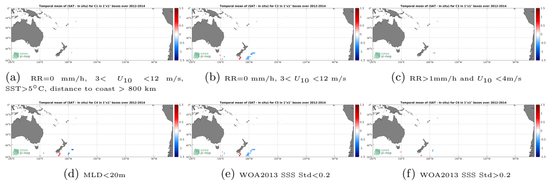
Figure 12: Temporal mean gridded over spatial boxes of size 1^\circ \times 1^\circ of \Delta SSS (Aquarius-L3-OR-V5-7DAY-RUNNING-1DEG - Sea mammals) for 6 different subdatasets corresponding to:RR=0 mm/h, 3 < U_{10} < 12 m/s, SST > 5^\circ C , distance to coast > 800 km (a), RR=0 mm/h, 3 < U_{10} < 12 m/s (b), RR > 1 mm/h and U_{10} < 4 m/s (c),MLD < 20 m (d),WOA2013 SSS Std < 0.2 (e),WOA2013 SSS Std > 0.2 (f).
