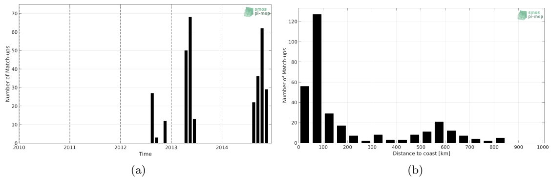
Figure 1: Number of match-ups between Sea mammals and Aquarius-L3-OR-V5-7DAY-RUNNING-1DEG SSS as a function of time (a) and as function of the distance to coast (b) over the South Pacific Ocean Pi-MEP region and for the full satellite product period.
