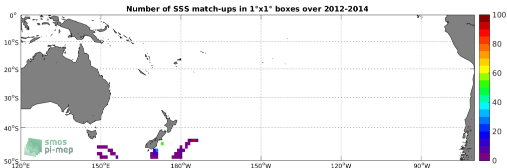
Figure 4: Number of SSS match-ups between Sea mammals SSS and the Aquarius-L3-OR-V5-7DAY-RUNNING-1DEG SSS product for the South Pacific Ocean Pi-MEP region over 1^\circ \times 1^\circ boxes and for the full satellite product period.
