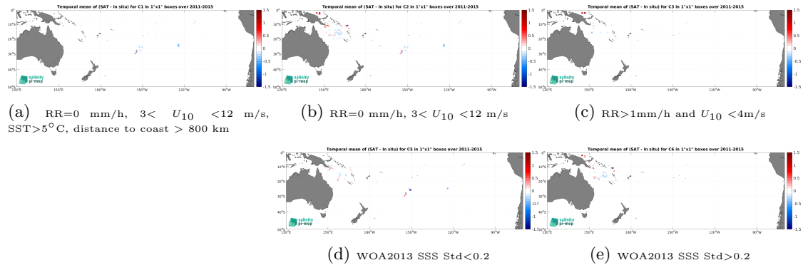
Figure 13: Temporal mean gridded over spatial boxes of size 1^\circ \times 1^\circ of \Delta\text{SSS} (Aquarius SSS L3 OR v5 - 7-Day running (NASA-GSFC) - Surface drifters) for 5 different subdatasets corresponding to:RR=0 mm/h, 3 < U_{10} < 12 m/s, SST >5^\circ\text{C} , distance to coast > 800 km (a), RR=0 mm/h, 3 < U_{10} < 12 m/s (b), RR >1 mm/h and U_{10} < 4 m/s (c), WOA2013 SSS Std <0.2 (d), WOA2013 SSS Std >0.2 (e).
