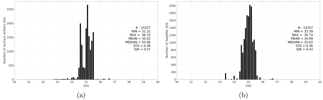
Figure 3: Histograms of SSS from Surface drifters (a) and Aquarius SSS L3 OR v5 - 7-Day running (NASA-GSFC) (b) considering all match-up pairs per bins of 0.1 over the South Pacific Ocean Pi-MEP region and for the full satellite product period.
