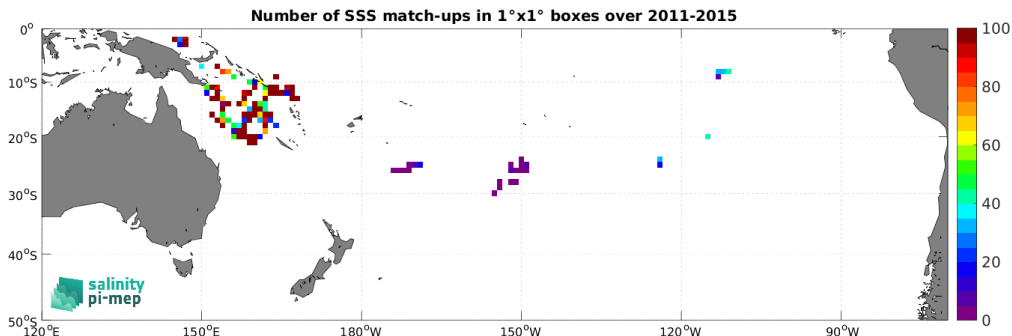
Figure 4: Number of SSS match-ups between Surface drifters SSS and the Aquarius SSS L3 OR v5 - 7-Day running (NASA-GSFC) SSS product for the South Pacific Ocean Pi-MEP region over 1^\circ \times 1^\circ boxes and for the full satellite product period.
