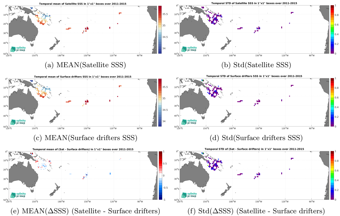
Figure 6: Temporal mean (left) and Std (right) of SSS from Aquarius SSS L3 OR v5 - 7-Day running (NASA-GSFC) (top), Surface drifters (middle), and of \Delta SSS (Satellite - Surface drifters). Only match-up pairs are used to generate these maps.
