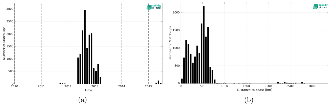
Figure 2: Number of match-ups between Surface drifters and Aquarius SSS L3 OR v5 - 7-Day running (NASA-GSFC) SSS as a function of time (a) and as function of the distance to coast (b) over the South Pacific Ocean Pi-MEP region and for the full satellite product period.
