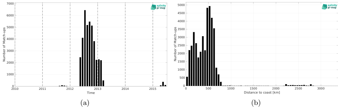
Figure 1: Number of match-ups between Surface drifters and Aquarius SSS L3 OR v5 - 7-Day running (NASA-GSFC) SSS as a function of time (a) and as function of the distance to coast (b) over the South Pacific Ocean Pi-MEP region and for the full satellite product period.
