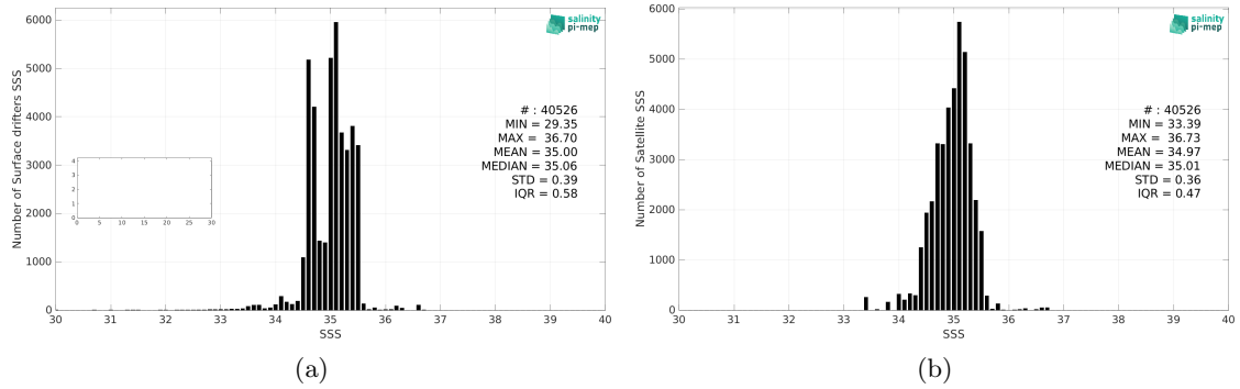
Figure 2: Histograms of SSS from Surface drifters (a) and Aquarius SSS L3 OR v5 - 7-Day running (NASA-GSFC) (b) considering all match-up pairs per bins of 0.1 over the South Pacific Ocean Pi-MEP region and for the full satellite product period.
