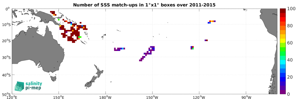
Figure 3: Number of SSS match-ups between Surface drifters SSS and the Aquarius SSS L3 OR v5 - 7-Day running (NASA-GSFC) SSS product for the South Pacific Ocean Pi-MEP region over 1^\circ \times 1^\circ boxes and for the full satellite product period.
