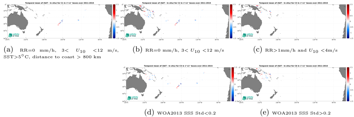
Figure 11: Temporal mean gridded over spatial boxes of size 1^\circ \times 1^\circ of \Delta\text{SSS} (Aquarius SSS L3 OR v5 - 7-Day running (NASA-GSFC) - Surface drifters) for 5 different subdatasets corresponding to:RR=0 mm/h, 3 < U_{10} < 12 m/s, SST >5^\circ\text{C} , distance to coast > 800 km (a), RR=0 mm/h, 3 < U_{10} < 12 m/s (b), RR >1 mm/h and U_{10} < 4 m/s (c), WOA2013 SSS Std <0.2 (d), WOA2013 SSS Std >0.2 (e).
