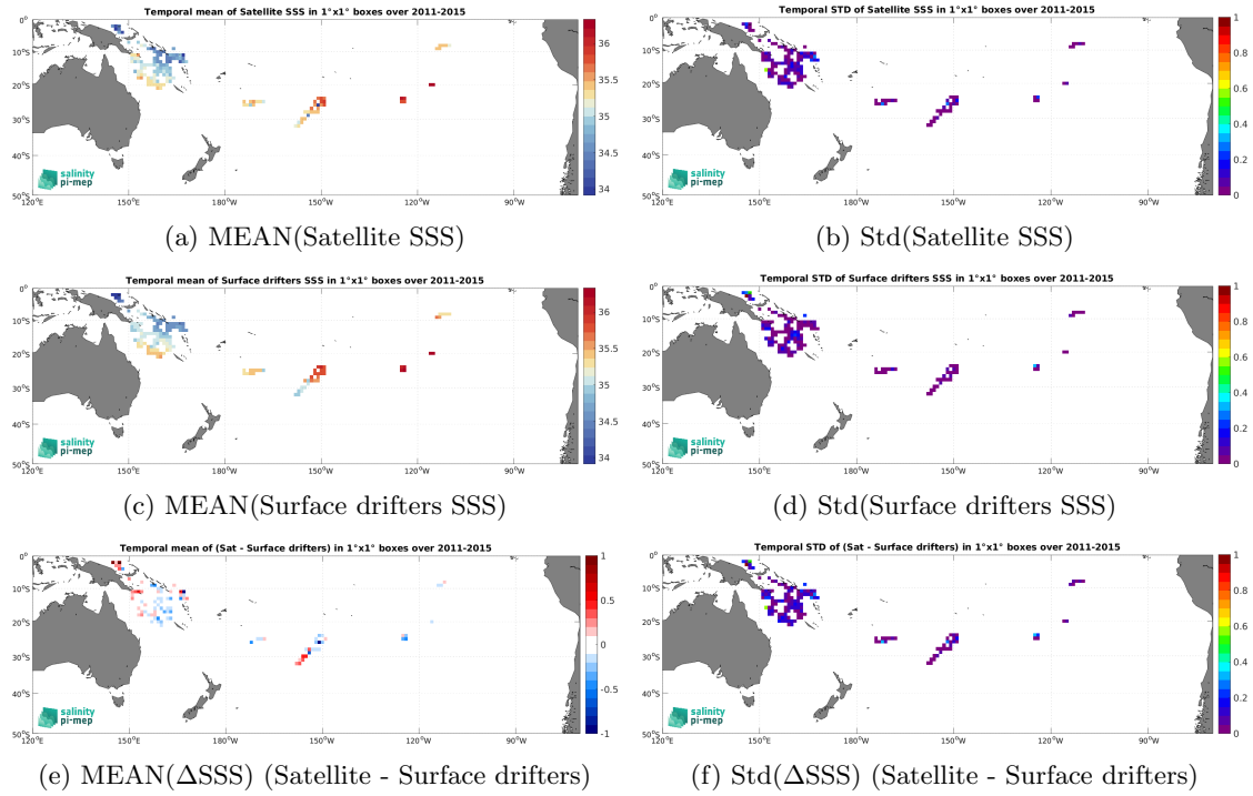
Figure 5: Temporal mean (left) and Std (right) of SSS from Aquarius SSS L3 OR v5 - 7-Day running (NASA-GSFC) (top), Surface drifters (middle), and of \Delta SSS (Satellite - Surface drifters). Only match-up pairs are used to generate these maps.
