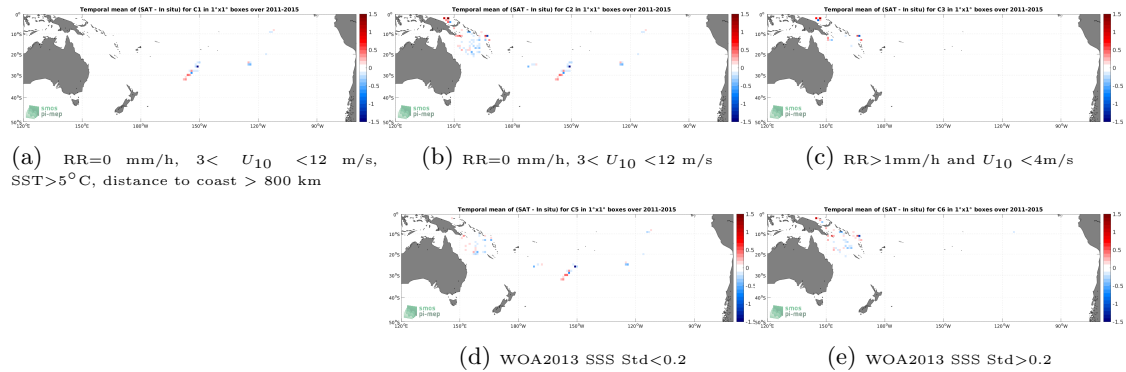
Figure 11: Temporal mean gridded over spatial boxes of size 1^\circ \times 1^\circ of \Delta SSS (Aquarius SSS L3 OR v5 - 7-Day running (NASA-GSFC) - Surface drifters) for 5 different subdatasets corresponding to:RR=0 mm/h, 3 < U_{10} < 12 m/s, SST >5^\circ C, distance to coast > 800 km (a), RR=0 mm/h, 3 < U_{10} < 12 m/s (b), RR >1 mm/h and U_{10} < 4 m/s (c), WOA2013 SSS Std <0.2 (d), WOA2013 SSS Std >0.2 (e).
