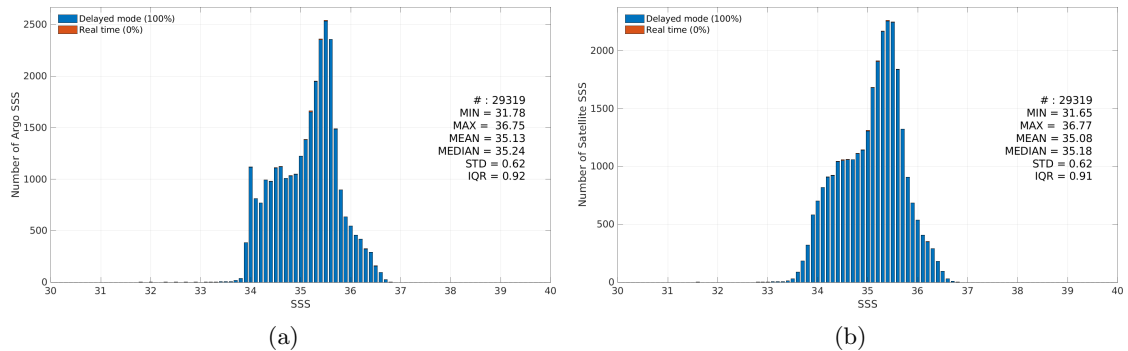
Figure 3: Histograms of SSS from Argo (a) and Aquarius SSS L3 OR v5 - 7-Day running (NASA-GSFC) (b) considering all match-up pairs per bins of 0.1 over the South Pacific Ocean Pi-MEP region and for the full satellite product period.
