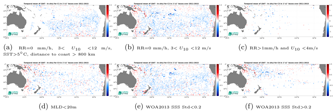
Figure 14: Temporal mean gridded over spatial boxes of size 1^\circ \times 1^\circ of \Delta SSS (Aquarius SSS L3 OR v5 - 7-Day running (NASA-GSFC) - Argo) for 6 different subdatasets corresponding to:RR=0 mm/h, 3 < U_{10} < 12 m/s, SST >5^\circ C, distance to coast > 800 km (a), RR=0 mm/h, 3 < U_{10} < 12 m/s (b), RR >1 mm/h and U_{10} < 4 m/s (c),MLD <20 m (d),WOA2013 SSS Std <0.2 (e),WOA2013 SSS Std >0.2 (f).
