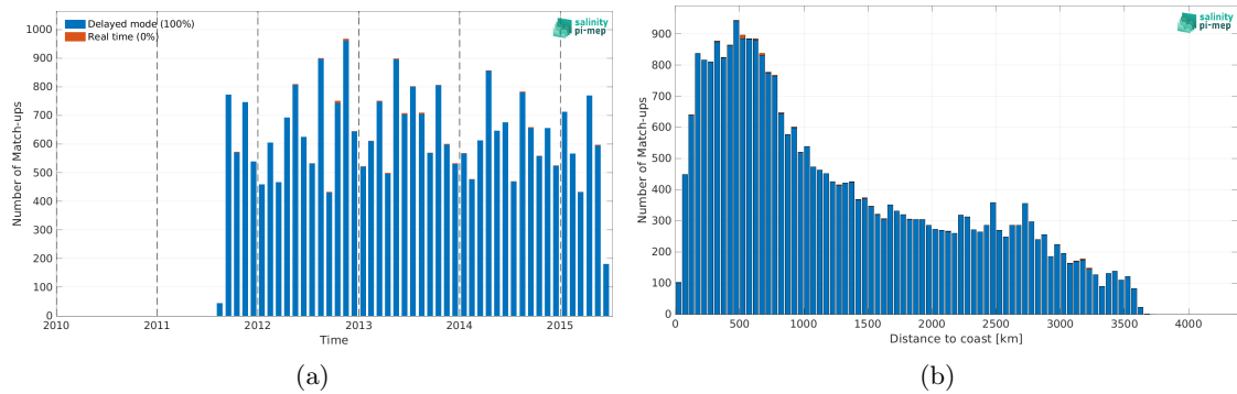
Figure 2: Number of match-ups between Argo and Aquarius SSS L3 OR v5 - 7-Day running (NASA-GSFC) SSS as a function of time (a) and as function of the distance to coast (b) over the South Pacific Ocean Pi-MEP region and for the full satellite product period.
