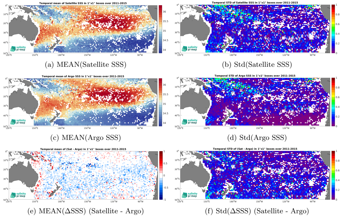
Figure 7: Temporal mean (left) and Std (right) of SSS from Aquarius SSS L3 OR v5 - 7-Day running (NASA-GSFC) (top), Argo (middle), and of \Delta SSS (Satellite - Argo). Only match-up pairs are used to generate these maps.
