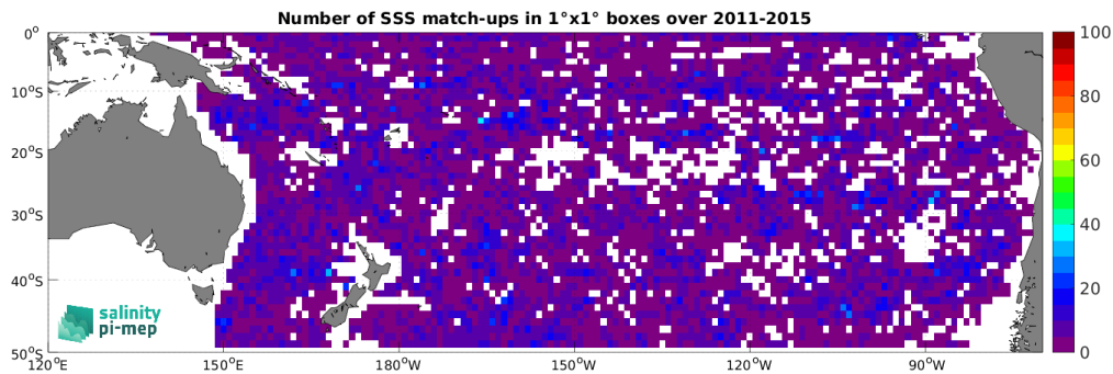
Figure 5: Number of SSS match-ups between Argo SSS and the Aquarius SSS L3 OR v5 - 7-Day running (NASA-GSFC) SSS product for the South Pacific Ocean Pi-MEP region over 1^\circ \times 1^\circ boxes and for the full satellite product period.
