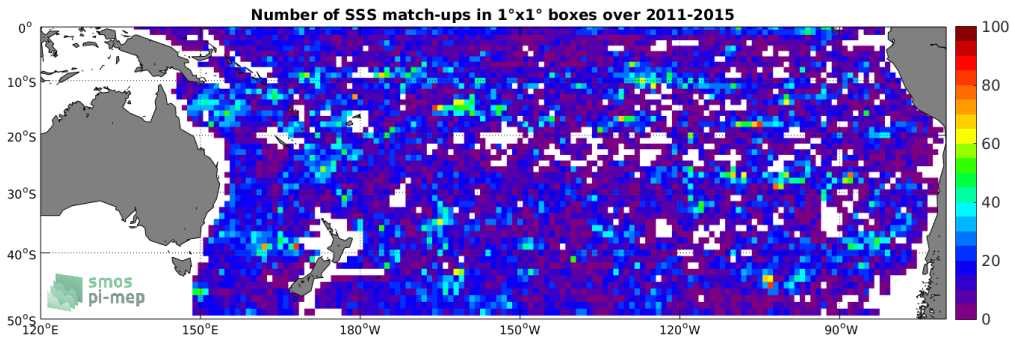
Figure 4: Number of SSS match-ups between Argo SSS and the Aquarius-L3-OR-V5-7DAY-RUNNING-1DEG SSS product for the South Pacific Ocean Pi-MEP region over 1^\circ \times 1^\circ boxes and for the full satellite product period.
