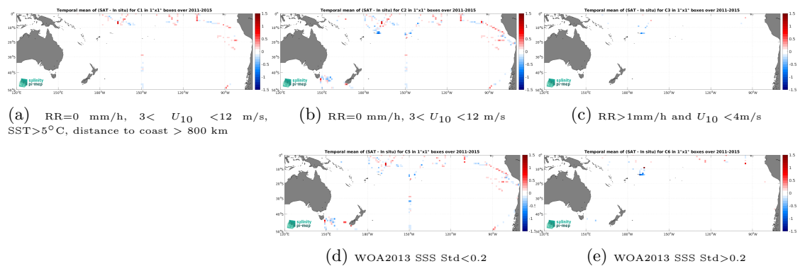
Figure 14: Temporal mean gridded over spatial boxes of size 1^\circ \times 1^\circ of \Delta SSS (Aquarius SSS L3 OR v5 - 7-Day running - Rain mask (NASA-GSFC) - TSG (SAMOS)) for 5 different subdatasets corresponding to:RR=0 mm/h, 3 < U_{10} < 12 m/s, SST >5^\circ\text{C} , distance to coast > 800 km (a), RR=0 mm/h, 3 < U_{10} < 12 m/s (b), RR >1 mm/h and U_{10} < 4 m/s (c), WOA2013 SSS Std <0.2 (d), WOA2013 SSS Std >0.2 (e).
