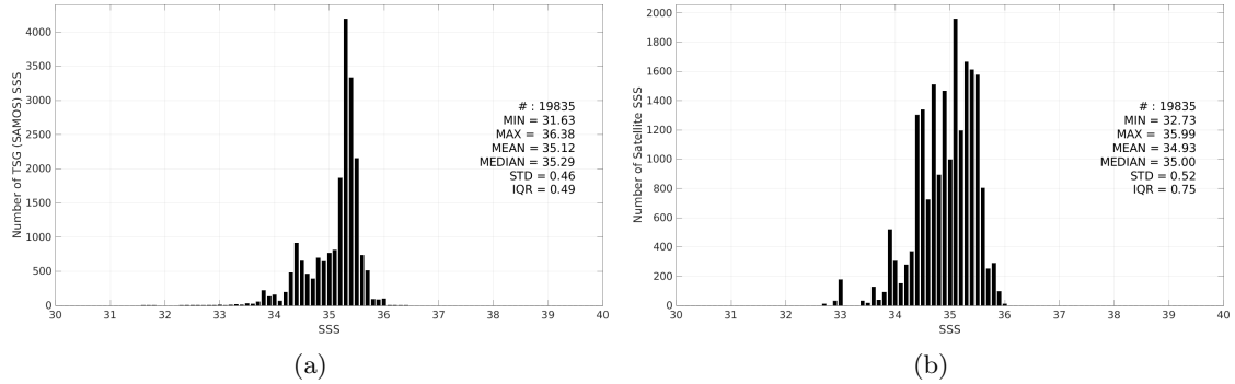
Figure 3: Histograms of SSS from TSG (SAMOS) (a) and Aquarius SSS L3 OR v5 - 7-Day running - Rain mask (NASA-GSFC) (b) considering all match-up pairs per bins of 0.1 over the South Pacific Ocean Pi-MEP region and for the full satellite product period.
