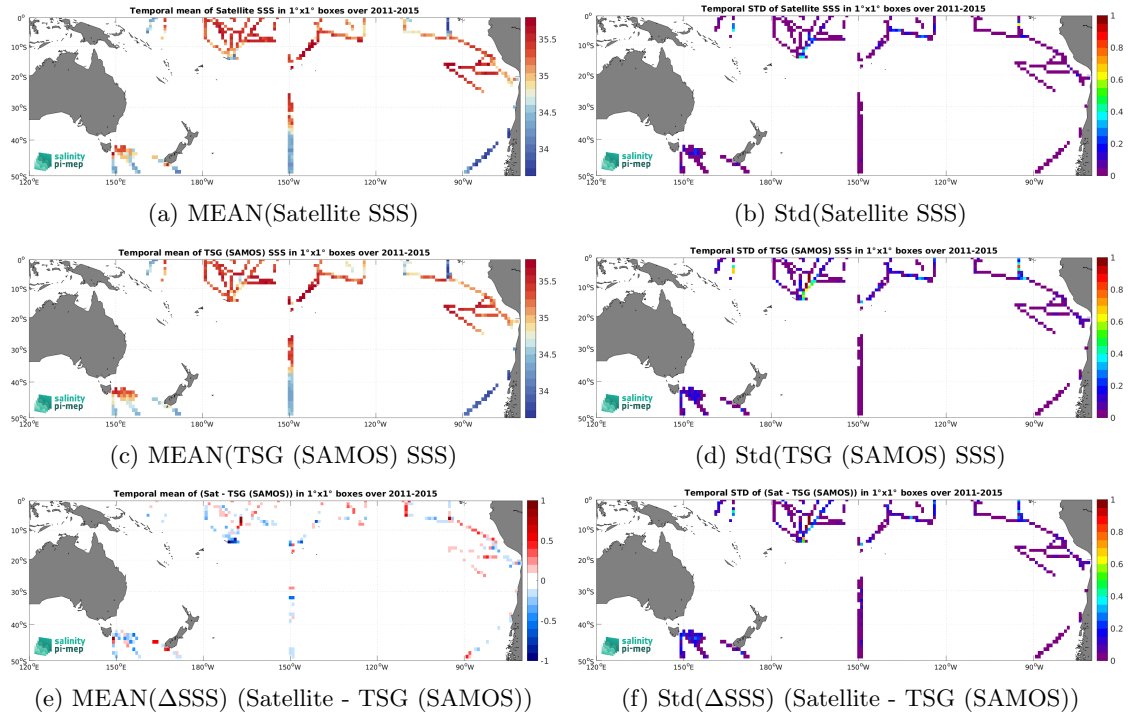
Figure 7: Temporal mean (left) and Std (right) of SSS from Aquarius SSS L3 OR v5 - 7-Day running - Rain mask (NASA-GSFC) (top), TSG (SAMOS) (middle), and of \Delta SSS (Satellite - TSG (SAMOS)). Only match-up pairs are used to generate these maps.
