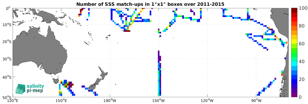
Figure 5: Number of SSS match-ups between TSG (SAMOS) SSS and the Aquarius SSS L3 OR v5 - 7-Day running - Rain mask (NASA-GSFC) SSS product for the South Pacific Ocean Pi-MEP region over 1^\circ \times 1^\circ boxes and for the full satellite product period.
