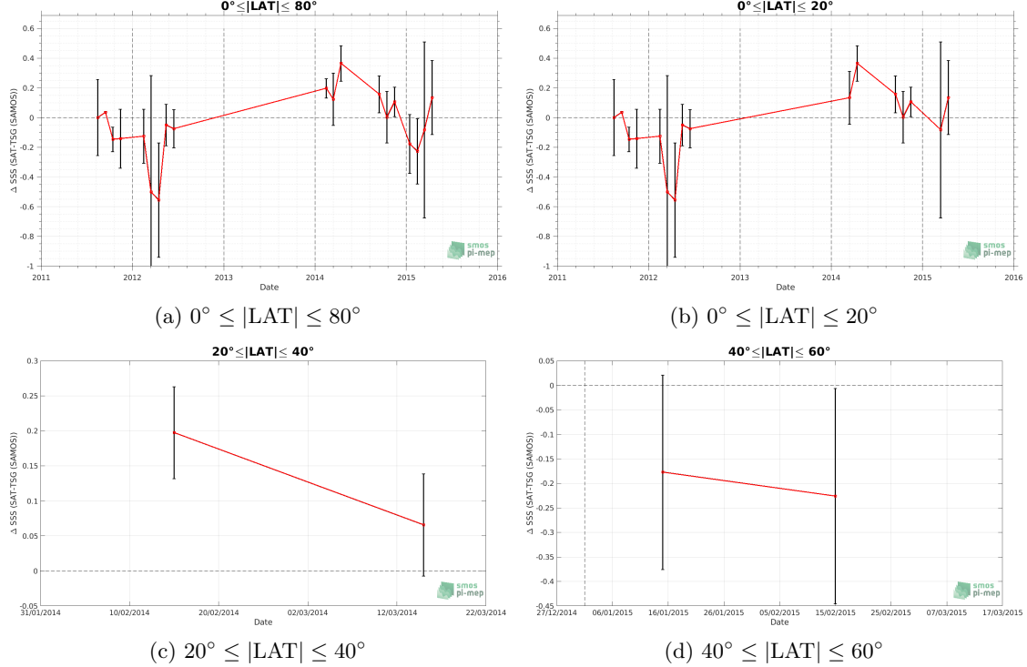
Figure 10: Monthly median (red curves) of \Delta\text{SSS} (Satellite - TSG (SAMOS)) and \pm 1 Std (black vertical thick bars) as function of time for all the collected Pi-MEP match-up pairs estimated over the South Pacific Ocean Pi-MEP region and for the full satellite product period are shown for different latitude bands: (a) 80°S-80°N, (b) 20°S-20°N, (c) 40°S-20°S and 20°N-40°N and (d) 60°S-40°S and 40°N-60°N.
