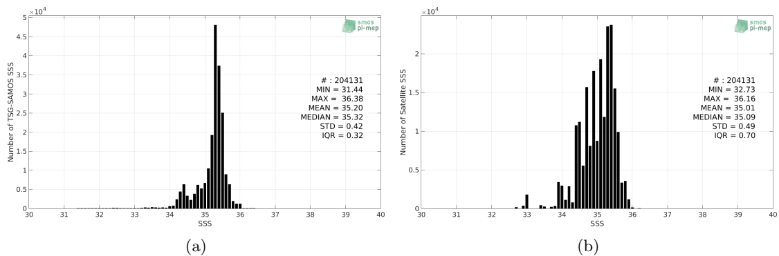
Figure 2: Histograms of SSS from TSG-SAMOS (a) and Aquarius-L3-OR-V5-7DAY-RUNNING-RAIN-MASK-1DEG (b) considering all match-up pairs per bins of 0.1 over the South Pacific Ocean Pi-MEP region and for the full satellite product period.
