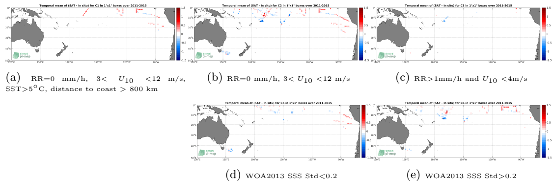
Figure 12: Temporal mean gridded over spatial boxes of size 1^\circ \times 1^\circ of \Delta SSS (Aquarius-L3-OR-V5-7DAY-RUNNING-RAIN-MASK-1DEG - TSG-SAMOS) for 5 different subdatasets corresponding to:RR=0 mm/h, 3 < U_{10} < 12 m/s, SST >5^\circ C, distance to coast > 800 km (a), RR=0 mm/h, 3 < U_{10} < 12 m/s (b), RR >1 mm/h and U_{10} < 4 m/s (c), WOA2013 SSS Std <0.2 (d), WOA2013 SSS Std >0.2 (e).
