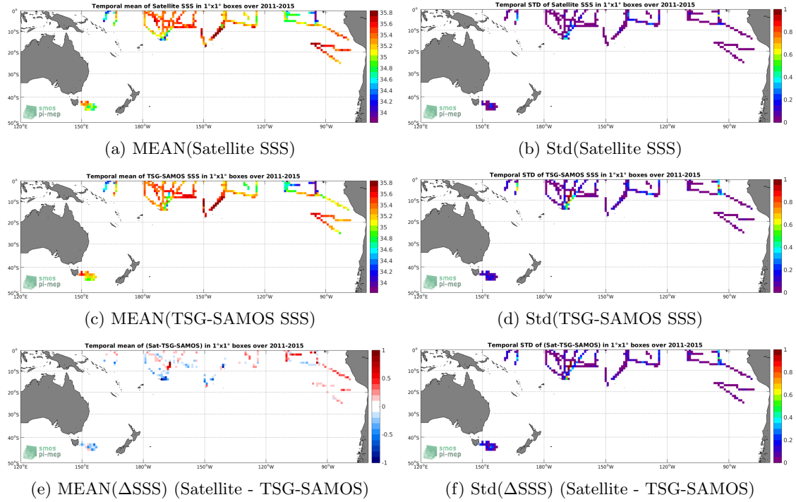
Figure 6: Temporal mean (left) and Std (right) of SSS from Aquarius-L3-OR-V5-7DAY-RUNNING-RAIN-MASK-1DEG (top), TSG-SAMOS (middle), and of \Delta SSS (Satellite - TSG-SAMOS). Only match-up pairs are used to generate these maps.
