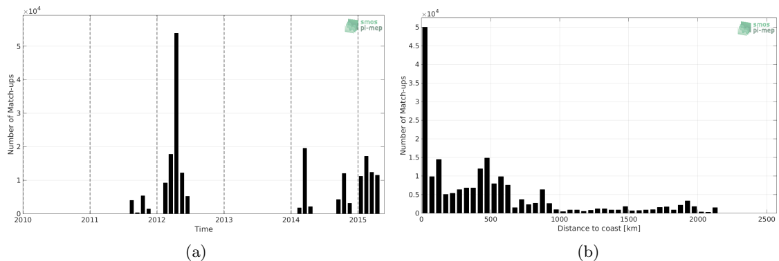
Figure 1: Number of match-ups between TSG-SAMOS and Aquarius-L3-OR-V5-7DAY-RUNNING-RAIN-MASK-1DEG SSS as a function of time (a) and as function of the distance to coast (b) over the South Pacific Ocean Pi-MEP region and for the full satellite product period.
