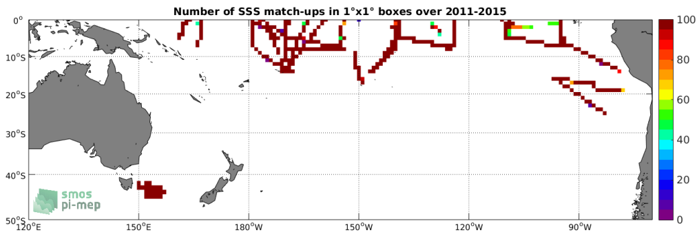
Figure 4: Number of SSS match-ups between TSG-SAMOS SSS and the Aquarius-L3-OR-V5-7DAY-RUNNING-RAIN-MASK-1DEG SSS product for the South Pacific Ocean Pi-MEP region over 1^\circ \times 1^\circ boxes and for the full satellite product period.
