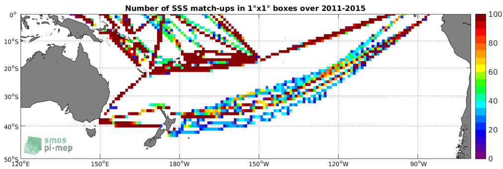
Figure 4: Number of SSS match-ups between TSG-LEGOS-DM SSS and the Aquarius-L3-OR-V5-7DAY-RUNNING-RAIN-MASK-1DEG SSS product for the South Pacific Ocean Pi-MEP region over 1°x1° boxes and for the full satellite product period.
