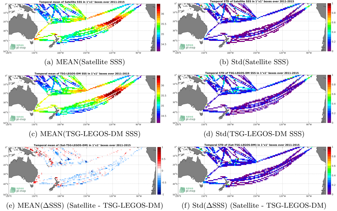
Figure 6: Temporal mean (left) and Std (right) of SSS from Aquarius-L3-OR-V5-7DAY-RUNNING-RAIN-MASK-1DEG (top), TSG-LEGOS-DM (middle), and of \Delta SSS (Satellite - TSG-LEGOS-DM). Only match-up pairs are used to generate these maps.
