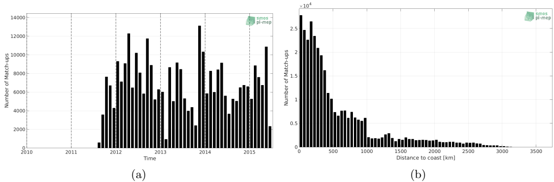
Figure 1: Number of match-ups between TSG-LEGOS-DM and Aquarius-L3-OR-V5-7DAY-RUNNING-RAIN-MASK-1DEG SSS as a function of time (a) and as function of the distance to coast (b) over the South Pacific Ocean Pi-MEP region and for the full satellite product period.
