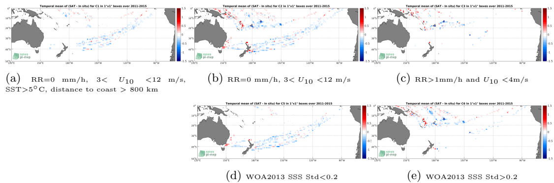
Figure 12: Temporal mean gridded over spatial boxes of size 1^\circ \times 1^\circ of \Delta SSS (Aquarius-L3-OR-V5-7DAY-RUNNING-RAIN-MASK-1DEG - TSG-LEGOS-DM) for 5 different subdatasets corresponding to:RR=0 mm/h, 3 < U_{10} < 12 m/s, SST >5^\circ C, distance to coast > 800 km (a), RR=0 mm/h, 3 < U_{10} < 12 m/s (b), RR >1 mm/h and U_{10} < 4 m/s (c), WOA2013 SSS Std <0.2 (d), WOA2013 SSS Std >0.2 (e).
