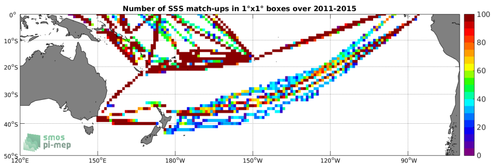
Figure 4: Number of SSS match-ups between TSG-LEGOS-DM SSS and the Aquarius-L3-OR-V5-7DAY-RUNNING-RAIN-MASK-1DEG SSS product for the South Pacific Ocean Pi-MEP region over 1^\circ \times 1^\circ boxes and for the full satellite product period.
