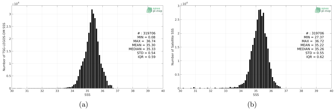
Figure 2: Histograms of SSS from TSG-LEGOS-DM (a) and Aquarius-L3-OR-V5-7DAY-RUNNING-RAIN-MASK-1DEG (b) considering all match-up pairs per bins of 0.1 over the South Pacific Ocean Pi-MEP region and for the full satellite product period.
