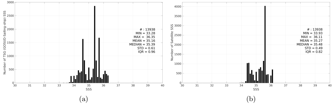
Figure 3: Histograms of SSS from TSG (GOSUD-Sailing-ship) (a) and Aquarius SSS L3 OR v5 - 7-Day running - Rain mask (NASA-GSFC) (b) considering all match-up pairs per bins of 0.1 over the South Pacific Ocean Pi-MEP region and for the full satellite product period.
