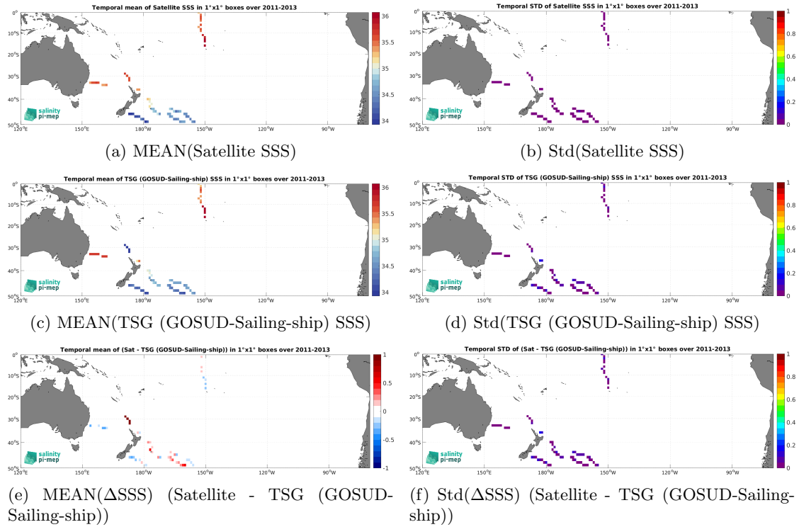
Figure 7: Temporal mean (left) and Std (right) of SSS from Aquarius SSS L3 OR v5 - 7-Day running - Rain mask (NASA-GSFC) (top), TSG (GOSUD-Sailing-ship) (middle), and of \Delta SSS (Satellite - TSG (GOSUD-Sailing-ship)). Only match-up pairs are used to generate these maps.
