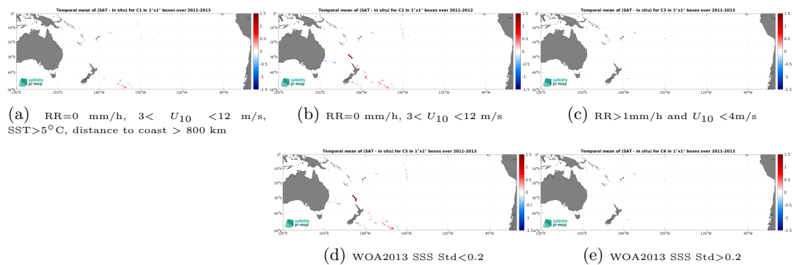
Figure 14: Temporal mean gridded over spatial boxes of size 1^\circ \times 1^\circ of \Delta SSS (Aquarius SSS L3 OR v5 - 7-Day running - Rain mask (NASA-GSFC) - TSG (GOSUD-Sailing-ship)) for 5 different subdatasets corresponding to:RR=0 mm/h, 3 < U_{10} < 12 m/s, SST >5^\circ\text{C} , distance to coast > 800 km (a), RR=0 mm/h, 3 < U_{10} < 12 m/s (b), RR >1 mm/h and U_{10} < 4 m/s (c), WOA2013 SSS Std <0.2 (d), WOA2013 SSS Std >0.2 (e).
