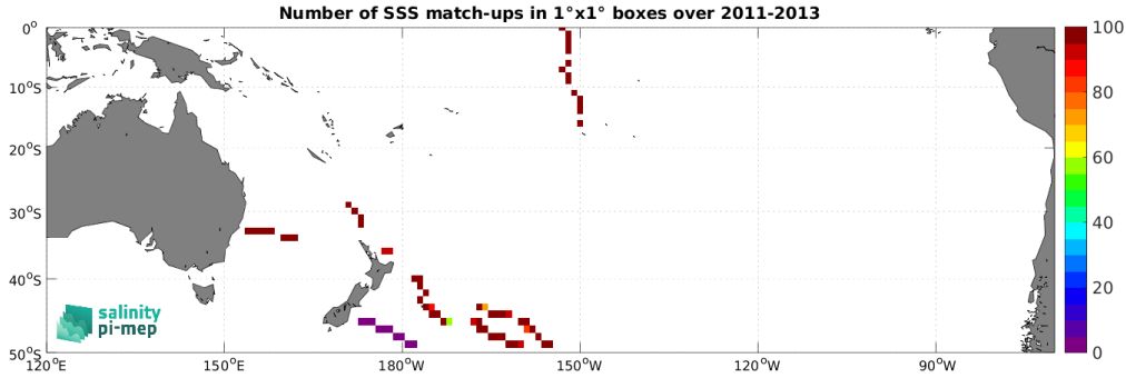
Figure 5: Number of SSS match-ups between TSG (GOSUD-Sailing-ship) SSS and the Aquarius SSS L3 OR v5 - 7-Day running - Rain mask (NASA-GSFC) SSS product for the South Pacific Ocean Pi-MEP region over 1^\circ \times 1^\circ boxes and for the full satellite product period.
