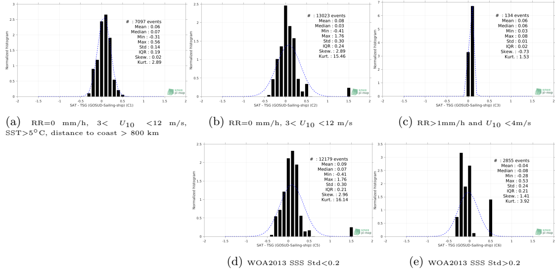
Figure 13: Normalized histogram of \Delta\text{SSS} (Aquarius SSS L3 OR v5 - 7-Day running - Rain mask (NASA-GSFC) - TSG (GOSUD-Sailing-ship)) for 5 different subdatasets corresponding to: RR=0 mm/h, 3 < U_{10} < 12 m/s, SST > 5^\circ\text{C} , distance to coast > 800 km (a), RR=0 mm/h, 3 < U_{10} < 12 m/s (b), RR > 1 mm/h and U_{10} < 4 m/s (c), WOA2013 SSS Std < 0.2 (d), WOA2013 SSS Std > 0.2 (e).
