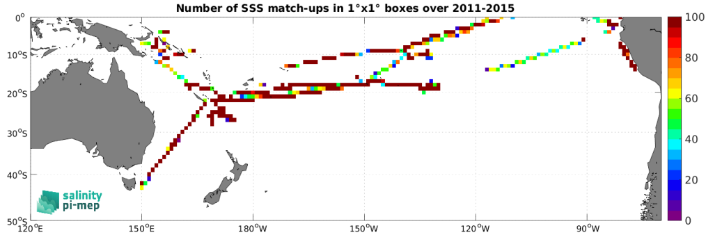
Figure 5: Number of SSS match-ups between TSG (GOSUD-Research-vessel) SSS and the Aquarius SSS L3 OR v5 - 7-Day running - Rain mask (NASA-GSFC) SSS product for the South Pacific Ocean Pi-MEP region over 1^\circ \times 1^\circ boxes and for the full satellite product period.
