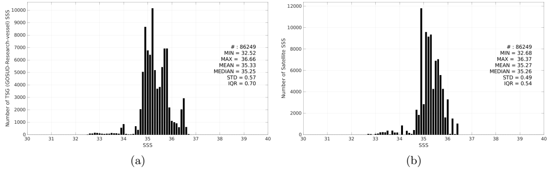
Figure 3: Histograms of SSS from TSG (GOSUD-Research-vessel) (a) and Aquarius SSS L3 OR v5 - 7-Day running - Rain mask (NASA-GSFC) (b) considering all match-up pairs per bins of 0.1 over the South Pacific Ocean Pi-MEP region and for the full satellite product period.
