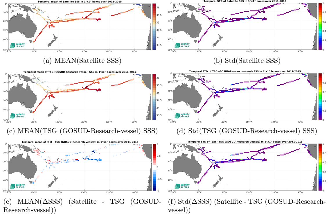
Figure 7: Temporal mean (left) and Std (right) of SSS from Aquarius SSS L3 OR v5 - 7-Day running - Rain mask (NASA-GSFC) (top), TSG (GOSUD-Research-vessel) (middle), and of \Delta\text{SSS} (Satellite - TSG (GOSUD-Research-vessel)). Only match-up pairs are used to generate these maps.
