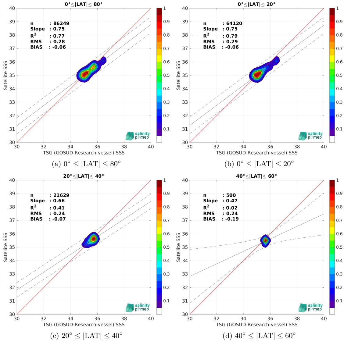
Figure 10: Contour maps of the concentration of Aquarius SSS L3 OR v5 - 7-Day running - Rain mask (NASA-GSFC) SSS ( y -axis) versus TSG (GOSUD-Research-vessel) SSS ( x -axis) at match-up pairs for different latitude bands. For each plot, the red line shows x=y . The black thin and dashed lines indicate a linear fit through the data cloud and the \pm 95\% confidence levels, respectively. The number match-up pairs n , the slope and R^2 coefficient of the linear fit, the root mean square (RMS) and the mean bias between satellite and in situ data are indicated for each latitude band in each plots.
