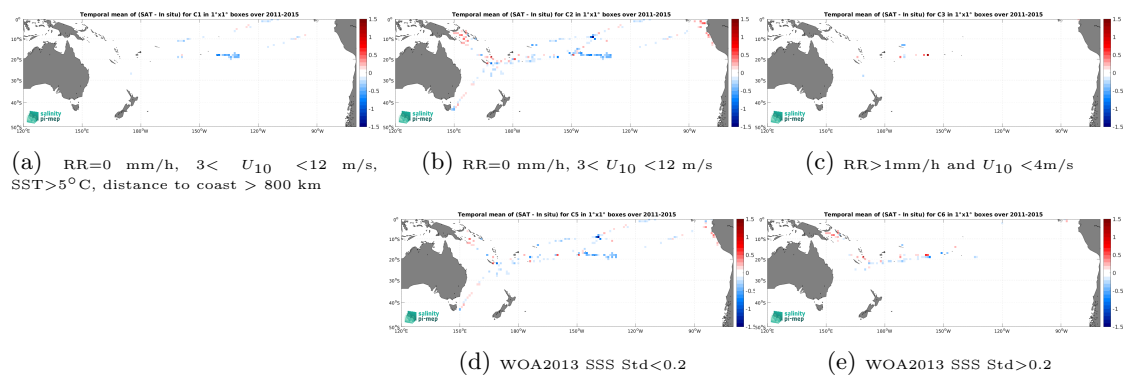
Figure 14: Temporal mean gridded over spatial boxes of size 1^\circ \times 1^\circ of \Delta SSS (Aquarius SSS L3 OR v5 - 7-Day running - Rain mask (NASA-GSFC) - TSG (GOSUD-Research-vessel)) for 5 different subdatasets corresponding to:RR=0 mm/h, 3 < U_{10} < 12 m/s, SST>5°C, distance to coast > 800 km (a), RR=0 mm/h, 3 < U_{10} < 12 m/s (b), RR>1mm/h and U_{10} < 4 m/s (c), WOA2013 SSS Std<0.2 (d), WOA2013 SSS Std>0.2 (e).
