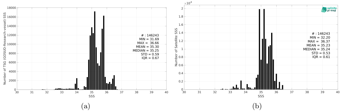
Figure 2: Histograms of SSS from TSG (GOSUD-Research-vessel) (a) and Aquarius SSS L3 OR v5 - 7-Day running - Rain mask (NASA-GSFC) (b) considering all match-up pairs per bins of 0.1 over the South Pacific Ocean Pi-MEP region and for the full satellite product period.
