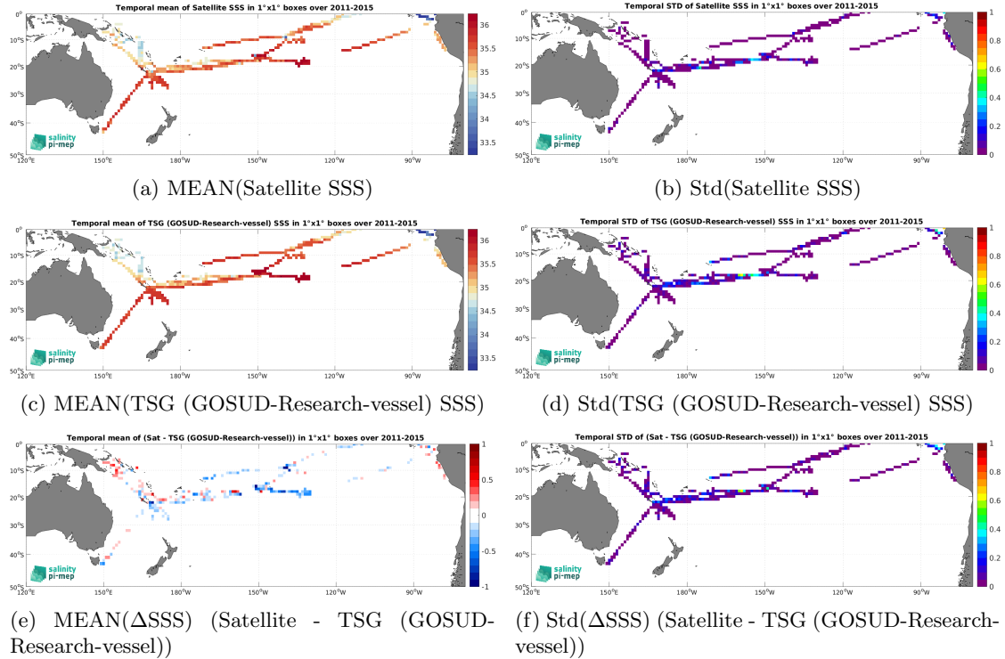
Figure 6: Temporal mean (left) and Std (right) of SSS from Aquarius SSS L3 OR v5 - 7-Day running - Rain mask (NASA-GSFC) (top), TSG (GOSUD-Research-vessel) (middle), and of \Delta\text{SSS} (Satellite - TSG (GOSUD-Research-vessel)). Only match-up pairs are used to generate these maps.
