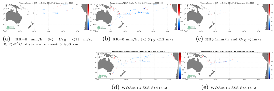
Figure 12: Temporal mean gridded over spatial boxes of size 1^\circ \times 1^\circ of \Delta SSS (Aquarius SSS L3 OR v5 - 7-Day running - Rain mask (NASA-GSFC) - TSG (GOSUD-Research-vessel)) for 5 different subdatasets corresponding to:RR=0 mm/h, 3 < U_{10} < 12 m/s, SST >5^\circ C, distance to coast > 800 km (a), RR=0 mm/h, 3 < U_{10} < 12 m/s (b), RR >1 mm/h and U_{10} < 4 m/s (c), WOA2013 SSS Std <0.2 (d), WOA2013 SSS Std >0.2 (e).
