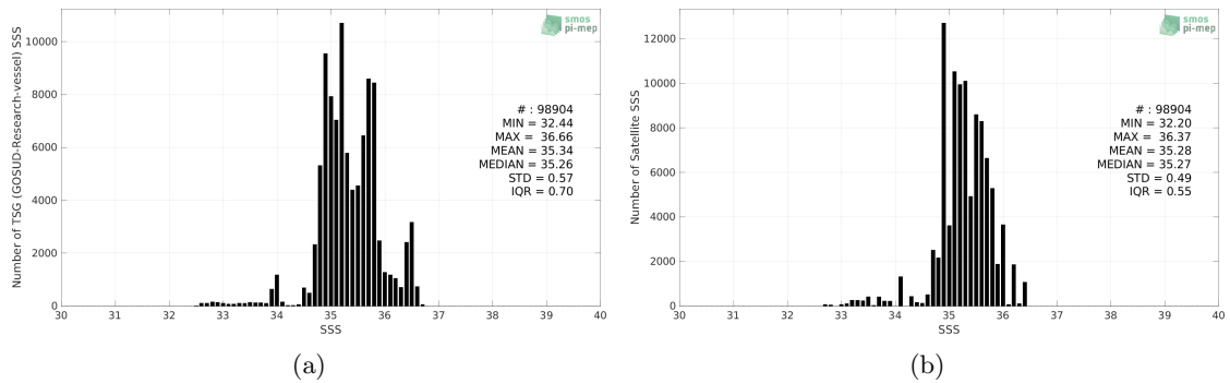
Figure 2: Histograms of SSS from TSG (GOSUD-Research-vessel) (a) and Aquarius SSS L3 OR v5 - 7-Day running - Rain mask (NASA-GSFC) (b) considering all match-up pairs per bins of 0.1 over the South Pacific Ocean Pi-MEP region and for the full satellite product period.
