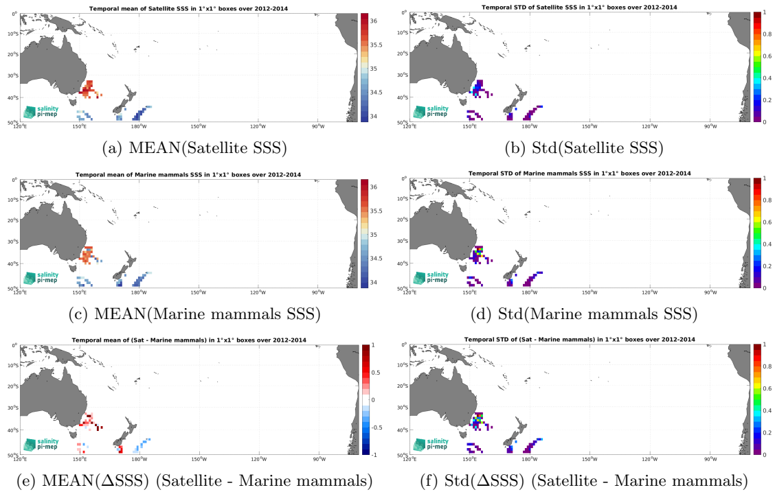
Figure 7: Temporal mean (left) and Std (right) of SSS from Aquarius SSS L3 OR v5 - 7-Day running - Rain mask (NASA-GSFC) (top), Marine mammals (middle), and of \Delta SSS (Satellite - Marine mammals). Only match-up pairs are used to generate these maps.
