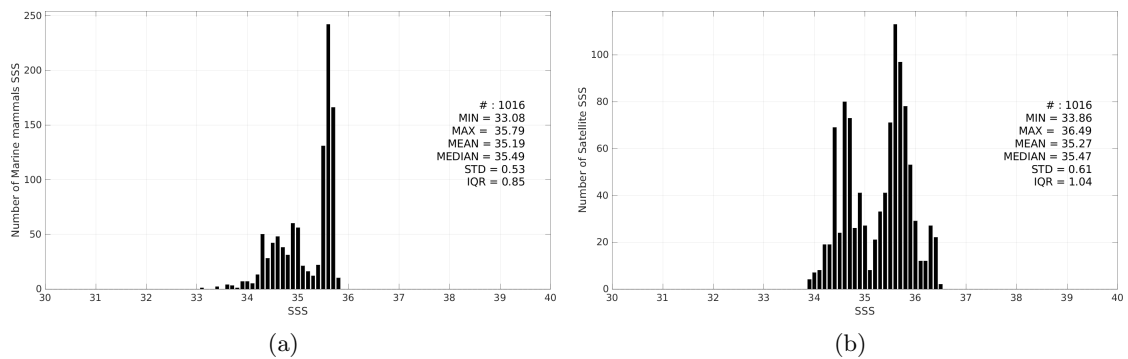
Figure 3: Histograms of SSS from Marine mammals (a) and Aquarius SSS L3 OR v5 - 7-Day running - Rain mask (NASA-GSFC) (b) considering all match-up pairs per bins of 0.1 over the South Pacific Ocean Pi-MEP region and for the full satellite product period.
