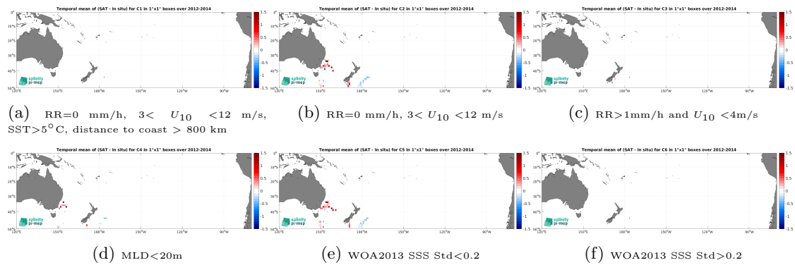
Figure 14: Temporal mean gridded over spatial boxes of size 1^\circ \times 1^\circ of \Delta SSS (Aquarius SSS L3 OR v5 - 7-Day running - Rain mask (NASA-GSFC) - Marine mammals) for 6 different subdatasets corresponding to:RR=0 mm/h, 3 < U_{10} < 12 m/s, SST >5^\circ C, distance to coast > 800 km (a), RR=0 mm/h, 3 < U_{10} < 12 m/s (b), RR >1 mm/h and U_{10} < 4 m/s (c),MLD <20 m (d),WOA2013 SSS Std <0.2 (e),WOA2013 SSS Std >0.2 (f).
