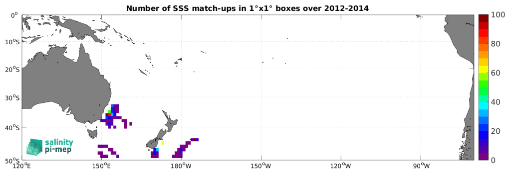
Figure 5: Number of SSS match-ups between Marine mammals SSS and the Aquarius SSS L3 OR v5 - 7-Day running - Rain mask (NASA-GSFC) SSS product for the South Pacific Ocean Pi-MEP region over 1^\circ \times 1^\circ boxes and for the full satellite product period.
