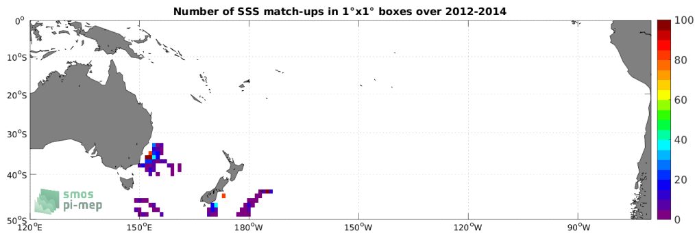
Figure 4: Number of SSS match-ups between Marine mammals SSS and the Aquarius SSS L3 OR v5 - 7-Day running - Rain mask (NASA-GSFC) SSS product for the South Pacific Ocean Pi-MEP region over 1^\circ \times 1^\circ boxes and for the full satellite product period.
