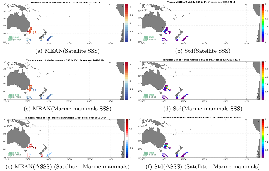
Figure 6: Temporal mean (left) and Std (right) of SSS from Aquarius SSS L3 OR v5 - 7-Day running - Rain mask (NASA-GSFC) (top), Marine mammals (middle), and of \Delta SSS (Satellite - Marine mammals). Only match-up pairs are used to generate these maps.
