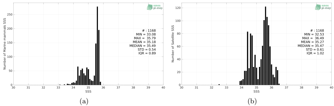
Figure 2: Histograms of SSS from Marine mammals (a) and Aquarius SSS L3 OR v5 - 7-Day running - Rain mask (NASA-GSFC) (b) considering all match-up pairs per bins of 0.1 over the South Pacific Ocean Pi-MEP region and for the full satellite product period.
