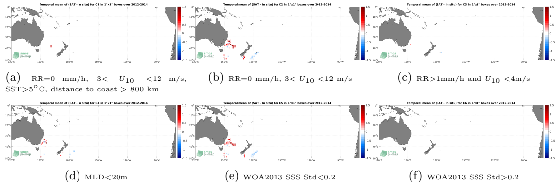
Figure 12: Temporal mean gridded over spatial boxes of size 1^{\circ}\times 1^{\circ} of \Delta\text{SSS} (Aquarius SSS L3 OR v5 - 7-Day running - Rain mask (NASA-GSFC) - Marine mammals) for 6 different subdatasets corresponding to:RR=0 mm/h, 3 < U_{10} < 12 m/s, SST >5^{\circ}\text{C} , distance to coast > 800 km (a), RR=0 mm/h, 3 < U_{10} < 12 m/s (b), RR >1\text{mm/h} and U_{10} < 4\text{m/s} (c),MLD <20\text{m} (d),WOA2013 SSS Std <0.2 (e),WOA2013 SSS Std >0.2 (f).
