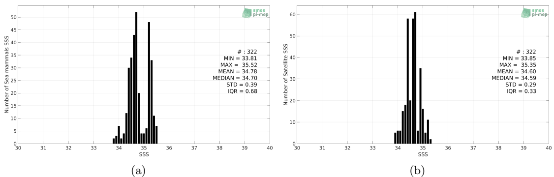
Figure 2: Histograms of SSS from Sea mammals (a) and Aquarius-L3-OR-V5-7DAY-RUNNING-RAIN-MASK-1DEG (b) considering all match-up pairs per bins of 0.1 over the South Pacific Ocean Pi-MEP region and for the full satellite product period.
