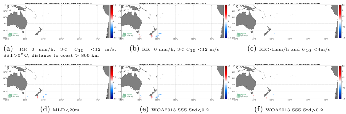
Figure 12: Temporal mean gridded over spatial boxes of size 1^\circ \times 1^\circ of \Delta SSS (Aquarius-L3-OR-V5-7DAY-RUNNING-RAIN-MASK-1DEG - Sea mammals) for 6 different subdatasets corresponding to: RR=0 mm/h, 3 < U_{10} < 12 m/s, SST > 5^\circ C, distance to coast > 800 km (a), RR=0 mm/h, 3 < U_{10} < 12 m/s (b), RR > 1 mm/h and U_{10} < 4 m/s (c), MLD < 20 m (d), WOA2013 SSS Std < 0.2 (e), WOA2013 SSS Std > 0.2 (f).
