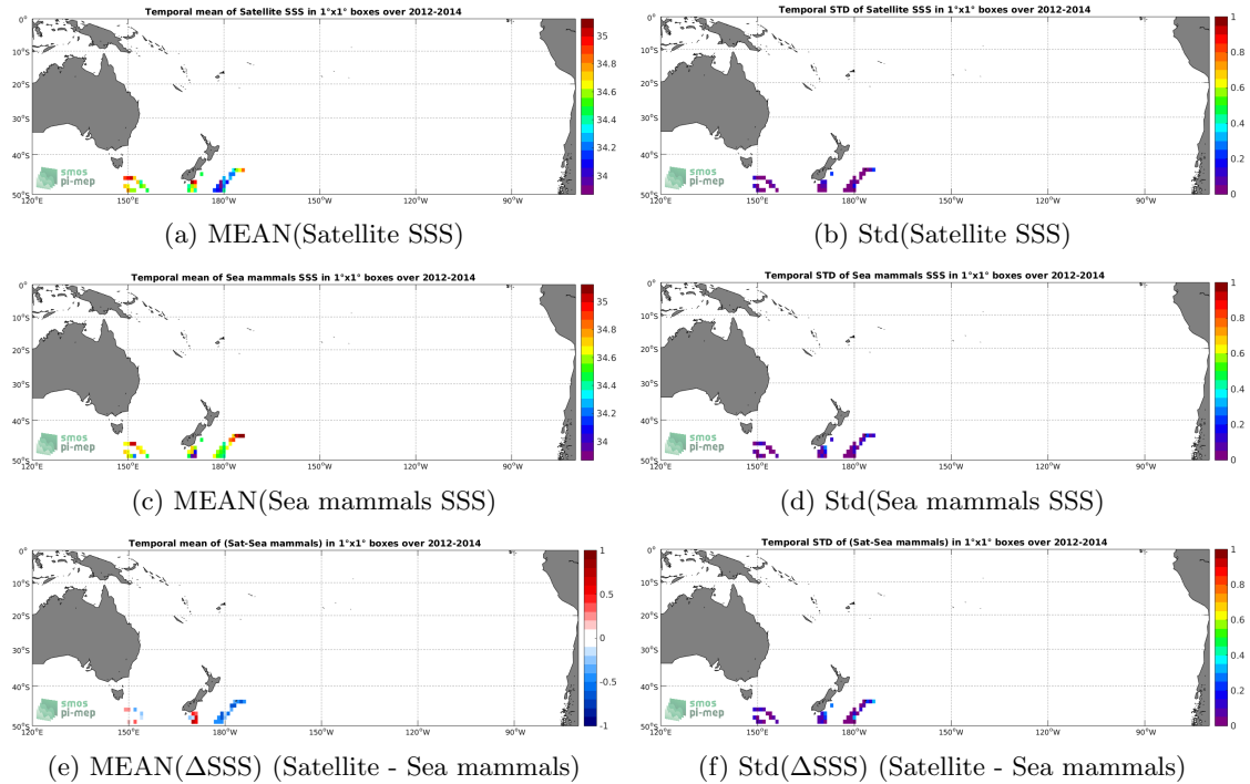
Figure 6: Temporal mean (left) and Std (right) of SSS from Aquarius-L3-OR-V5-7DAY-RUNNING-RAIN-MASK-1DEG (top), Sea mammals (middle), and of \Delta SSS (Satellite - Sea mammals). Only match-up pairs are used to generate these maps.
