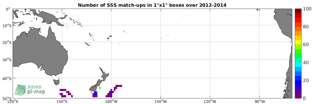
Figure 4: Number of SSS match-ups between Sea mammals SSS and the Aquarius-L3-OR-V5-7DAY-RUNNING-RAIN-MASK-1DEG SSS product for the South Pacific Ocean Pi-MEP region over 1^\circ \times 1^\circ boxes and for the full satellite product period.
