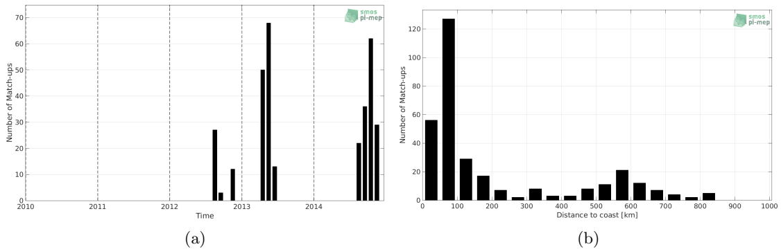
Figure 1: Number of match-ups between Sea mammals and Aquarius-L3-OR-V5-7DAY-RUNNING-RAIN-MASK-1DEG SSS as a function of time (a) and as function of the distance to coast (b) over the South Pacific Ocean Pi-MEP region and for the full satellite product period.
