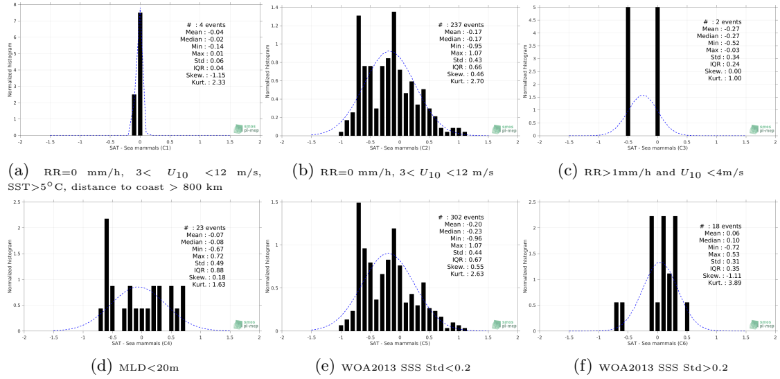
Figure 13: Normalized histogram of \Delta\text{SSS} (Aquarius-L3-OR-V5-7DAY-RUNNING-RAIN-MASK-1DEG - Sea mammals) for 6 different subdatasets corresponding to: RR=0 mm/h, 3 < U_{10} < 12 m/s, SST>5°C, distance to coast > 800 km (a), RR=0 mm/h, 3 < U_{10} < 12 m/s (b), RR>1mm/h and U_{10} < 4 m/s (c), MLD<20m (d), WOA2013 SSS Std<0.2 (e), WOA2013 SSS Std>0.2 (f).
