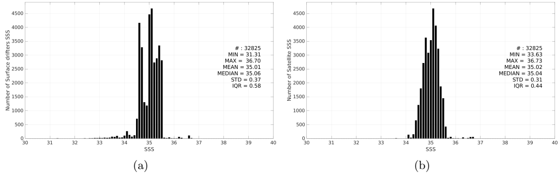
Figure 3: Histograms of SSS from Surface drifters (a) and Aquarius SSS L3 OR v5 - 7-Day running - Rain mask (NASA-GSFC) (b) considering all match-up pairs per bins of 0.1 over the South Pacific Ocean Pi-MEP region and for the full satellite product period.
