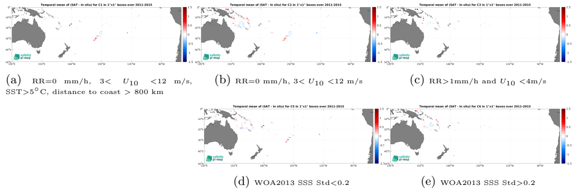
Figure 13: Temporal mean gridded over spatial boxes of size 1^\circ \times 1^\circ of \Delta SSS (Aquarius SSS L3 OR v5 - 7-Day running - Rain mask (NASA-GSFC) - Surface drifters) for 5 different subdatasets corresponding to:RR=0 mm/h, 3 < U_{10} < 12 m/s, SST >5^\circ\text{C} , distance to coast > 800 km (a), RR=0 mm/h, 3 < U_{10} < 12 m/s (b), RR >1 mm/h and U_{10} < 4 m/s (c), WOA2013 SSS Std <0.2 (d), WOA2013 SSS Std >0.2 (e).
