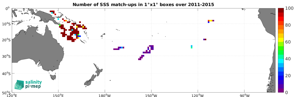
Figure 4: Number of SSS match-ups between Surface drifters SSS and the Aquarius SSS L3 OR v5 - 7-Day running - Rain mask (NASA-GSFC) SSS product for the South Pacific Ocean Pi-MEP region over 1^\circ \times 1^\circ boxes and for the full satellite product period.
