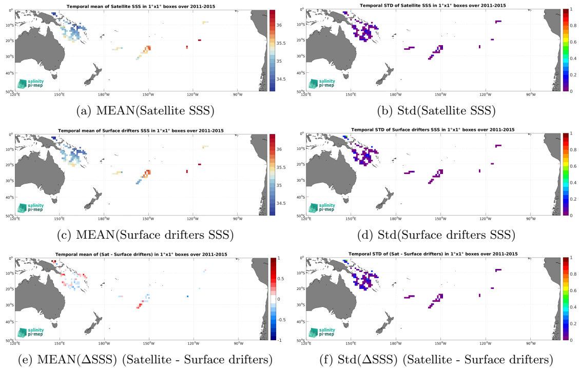
Figure 6: Temporal mean (left) and Std (right) of SSS from Aquarius SSS L3 OR v5 - 7-Day running - Rain mask (NASA-GSFC) (top), Surface drifters (middle), and of \Delta SSS (Satellite - Surface drifters). Only match-up pairs are used to generate these maps.
