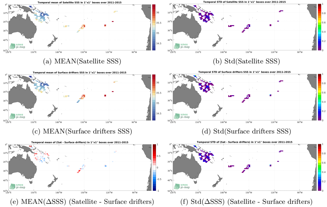
Figure 5: Temporal mean (left) and Std (right) of SSS from Aquarius SSS L3 OR v5 - 7-Day running - Rain mask (NASA-GSFC) (top), Surface drifters (middle), and of \Delta SSS (Satellite - Surface drifters). Only match-up pairs are used to generate these maps.
