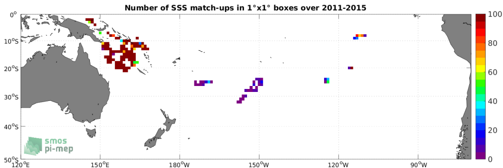
Figure 3: Number of SSS match-ups between Surface drifters SSS and the Aquarius SSS L3 OR v5 - 7-Day running - Rain mask (NASA-GSFC) SSS product for the South Pacific Ocean Pi-MEP region over 1^\circ \times 1^\circ boxes and for the full satellite product period.
