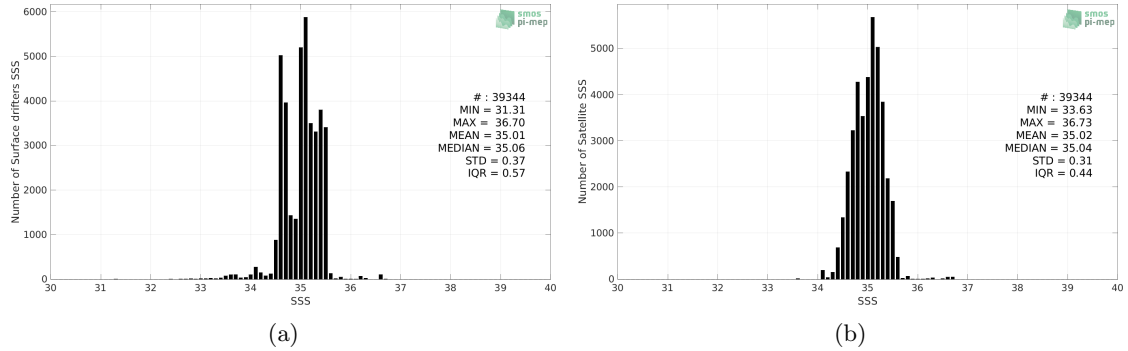
Figure 2: Histograms of SSS from Surface drifters (a) and Aquarius SSS L3 OR v5 - 7-Day running - Rain mask (NASA-GSFC) (b) considering all match-up pairs per bins of 0.1 over the South Pacific Ocean Pi-MEP region and for the full satellite product period.
