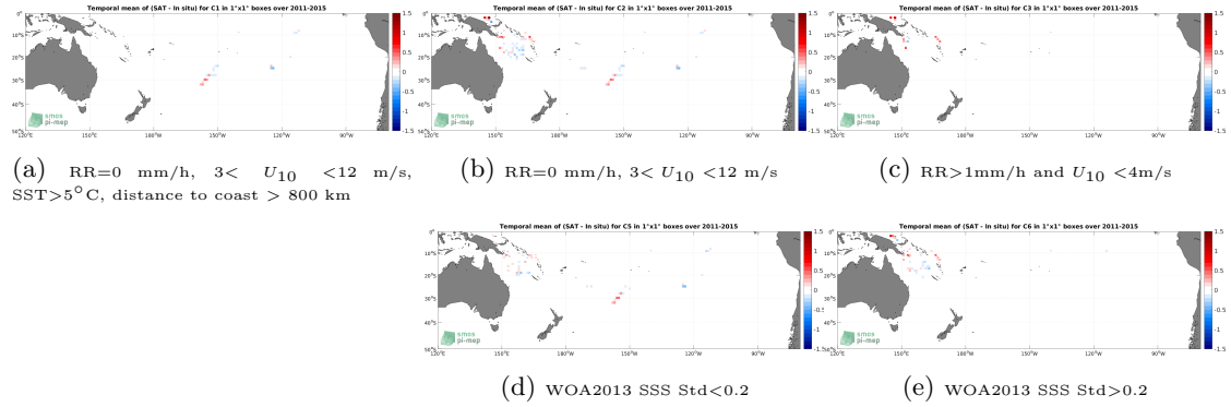
Figure 11: Temporal mean gridded over spatial boxes of size 1^{\circ}\times 1^{\circ} of \Delta\text{SSS} (Aquarius SSS L3 OR v5 - 7-Day running - Rain mask (NASA-GSFC) - Surface drifters) for 5 different subdatasets corresponding to: RR=0 mm/h, 3 < U_{10} < 12 m/s, SST > 5^{\circ}\text{C} , distance to coast > 800 km (a), RR=0 mm/h, 3 < U_{10} < 12 m/s (b), RR > 1 mm/h and U_{10} < 4 m/s (c), WOA2013 SSS Std < 0.2 (d), WOA2013 SSS Std > 0.2 (e).
